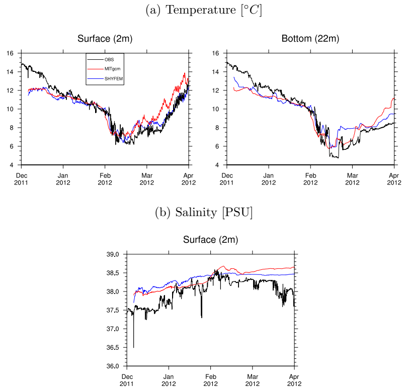
Fig. 1. Timeseries of (a) surface (left panel) and bottom (right panel) temperature and (b) surface salinity for SHYFEM (blue), MITgcm (red) and the Vida buoy observations (black).
