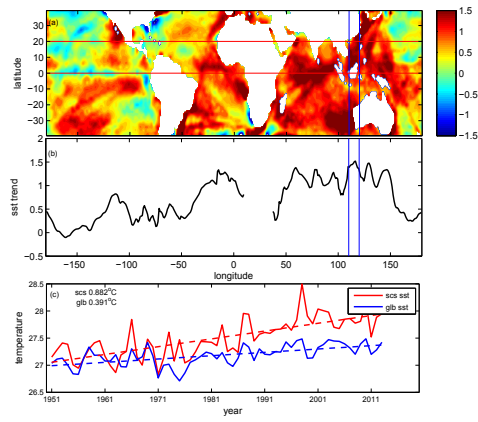
Figure R3. Linear trends (1951-2013) of the SST anomalies (color shaded unit: C /100 year) obtained from the HadISST (a). The Linear trends (1951-2013, 0-20° N meridional mean) of the SST anomalies (unit: C /100 year, b). The time series (1951-2013) of the SST in the SCS (red) and global mean (blue) obtained from the HadISST (c).
