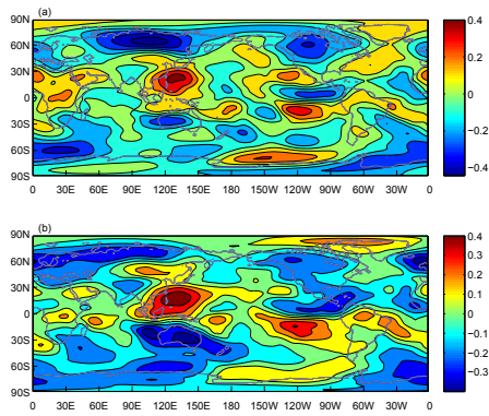
Figure R1. Lag correlation maps (lag day=15 day) of the northern SCS ( 12^{\circ} - 23^{\circ} N, 110^{\circ} - 121^{\circ} E) SSTA in the winter (October 2003 to March 2004) with global barotropic stream function (a) and baroclinic stream function.
