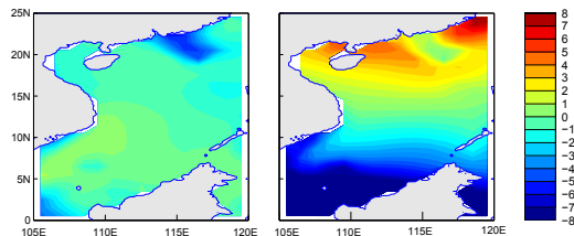
Figure R4. The summer- (a) and winter-mean (b) air-sea temperature difference (2 meter air temperature minus SST, units: C) in the SCS from 1982 to 2011, the 2 meter air temperature is from ECWMPF ERA-Interim and the OISST is from NOAA.
