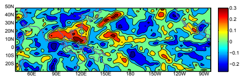
Figure R2. Lag correlation maps (Lag days=15d) of the northern SCS ( 12^{\circ} - 23^{\circ} N, 110^{\circ} - 121^{\circ} E) SSTA in the winter (October 2003 to March 2004) with global rainfall.
