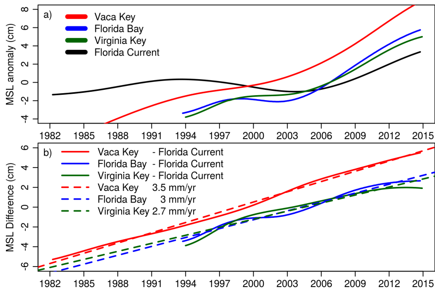
Figure 5. (a) \text{SSH-MSL} anomalies at Vaca Key, Florida Bay and Virginia Key from EMD residuals, and for the Florida Current at 27^\circ \text{N} assuming a \text{SSH-MSL}/\text{transport} rate of -1.4 \text{ cm Sv}^{-1} . (b) Difference of the Florida Current \text{SSH-MSL} anomaly from the \text{SSH-MSL} anomalies at Vaca Key, Florida Bay and Virginia Key. Dashed lines are linear regressions to the \text{SSH-MSL} differences.
