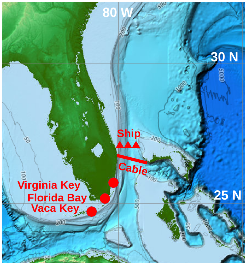
Figure 1. Map of Florida Straits with the cable and tide gauge and ship measurement locations. Bathymetry contours are in meters.
