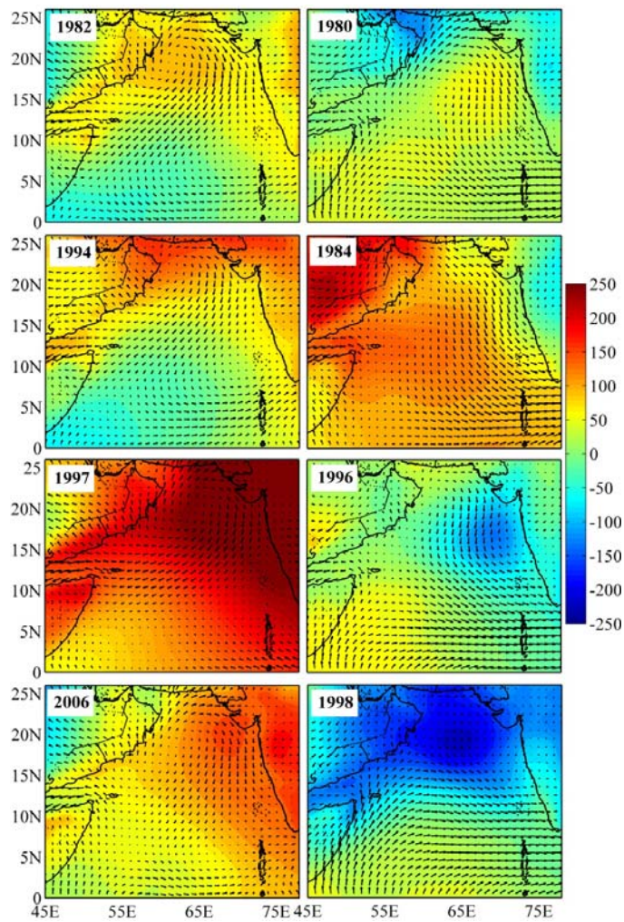
558 559 | Figure 978: Wind vector (m/s) and SLP anomaly (Pa) of eight strong positive (first column) 560 | and negative (second column) IOD years from 1979 to 2014. Years are shown inside the 561 | figure and SST anomaly of eastern and western equatorial IO with Dipole Mode Index for 562 | corresponding years are shown in Figure 4.
