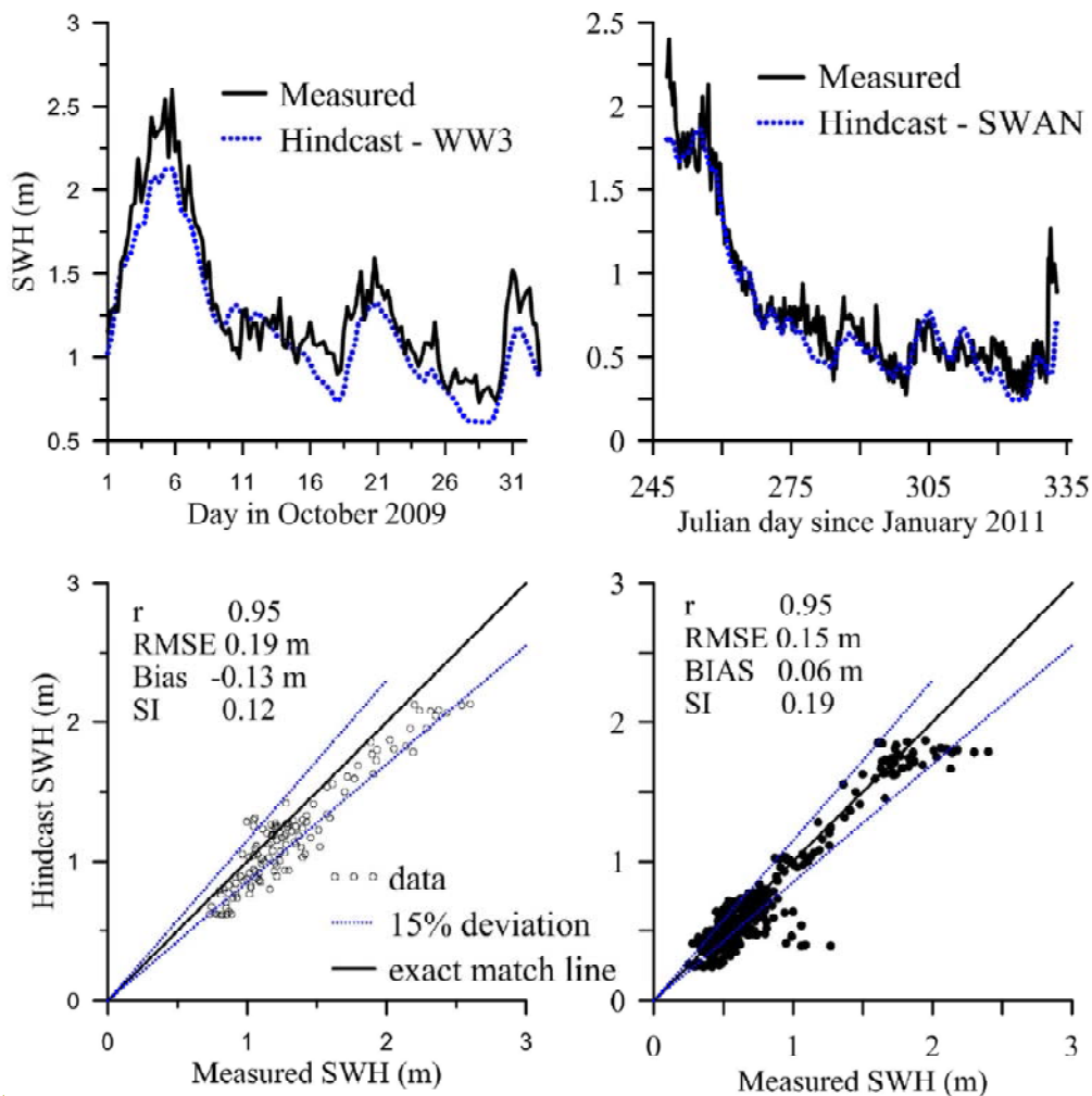
Figure 32: Comparison of hindcast SWH values with measured values. Left panel shows the values -during October 2009 at deep water location and the right panel shows the values during September-November 2011 at shallow water location (Ratnagiri).
