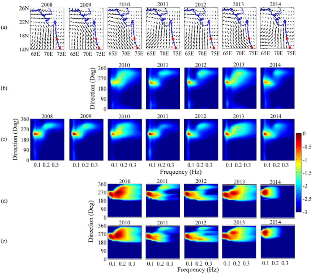
541 | Figure 645: Averaged wind pattern of October from 2008 to 2014 (row a). Averaged 542 measured wave frequency-directional spectra from 2008 to 2014 off Ratnagiri (row b) and off 543 Honnavar (row c) color bar is for spectral energy ( \text{m}^2 \cdot \text{Deg} / \text{Hz} ) d) Modeled directional 544 spectrum off Ratnagiri and (e) off Honnavar from 2010 to 2014. The spectral energy is shown 545 in logarithmic scale. SST anomalies of eastern and western equatorial IO with dipole mode 546 index are shown in Figure 4.
