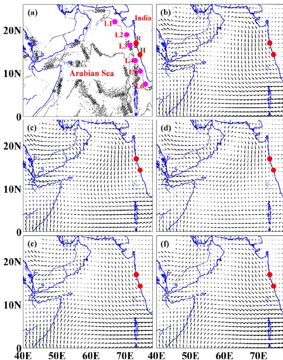
Figure 1: (a) The six locations considered to study the role of DMI on the wave climate is L1 to L6. The wave measuring locations (Ratnagiri and Honnavar) in central eastern AS is shown as red dots, (b) Composite climatological wind pattern during October in AS and part of equatorial Indian Ocean from 1958 to 2014. Averaged wind pattern during (c) pure positive IOD, (d) combined positive IOD, (e) Pure negative IOD and (f) Combined negative IOD from 1958 to 2014.
