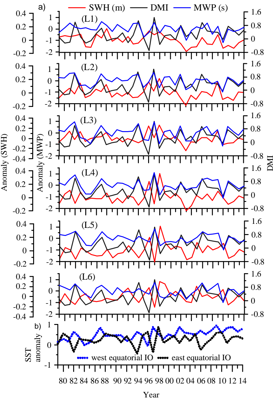
535 | Figure 4.53: a) Anomaly of significant wave height (SWH) and mean wave period (MWP) at 536 | selected six locations off west coast of India during October from 1979 to 2014. The wave
