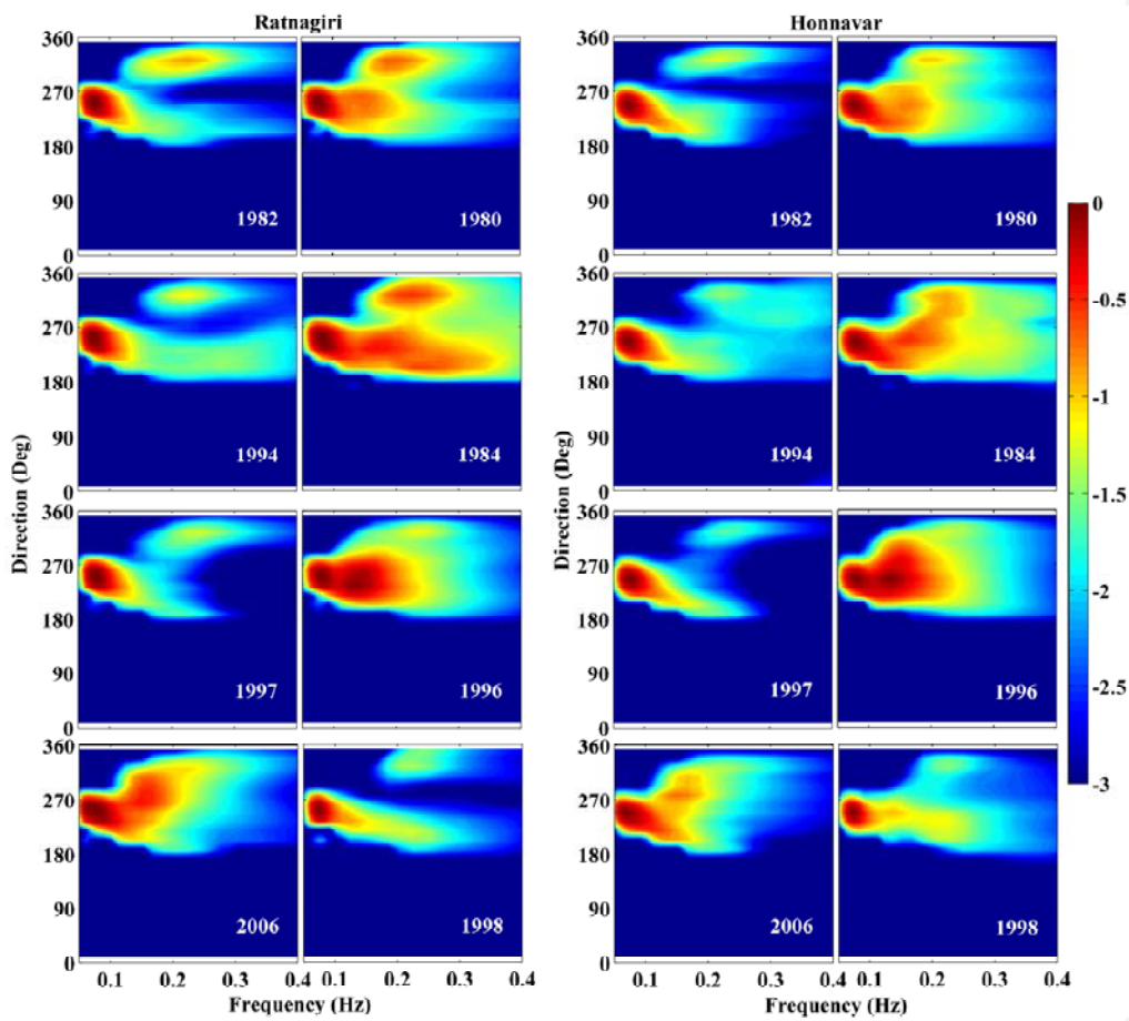
564 | Figure 4: Modeled directional spectrum off Honnavar and Ratnagiri for selected positive 565 | and negative IOD years (columns one and three for positive IOD and two and four for 566 | negative IOD). Corresponding years are shown inside the figures and dipole mode index are 567 | shown in Figure 4. The spectral energy is shown in logarithmic scale.
