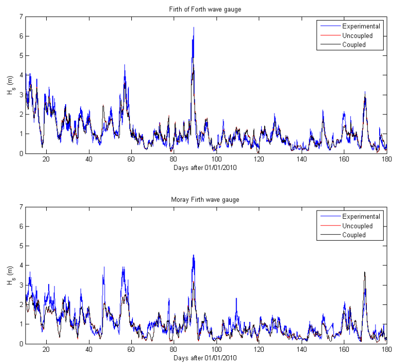
Figure 3. Comparison between observed and modelled H_s in the Firth of Forth and in the Moray Firth for 2010
