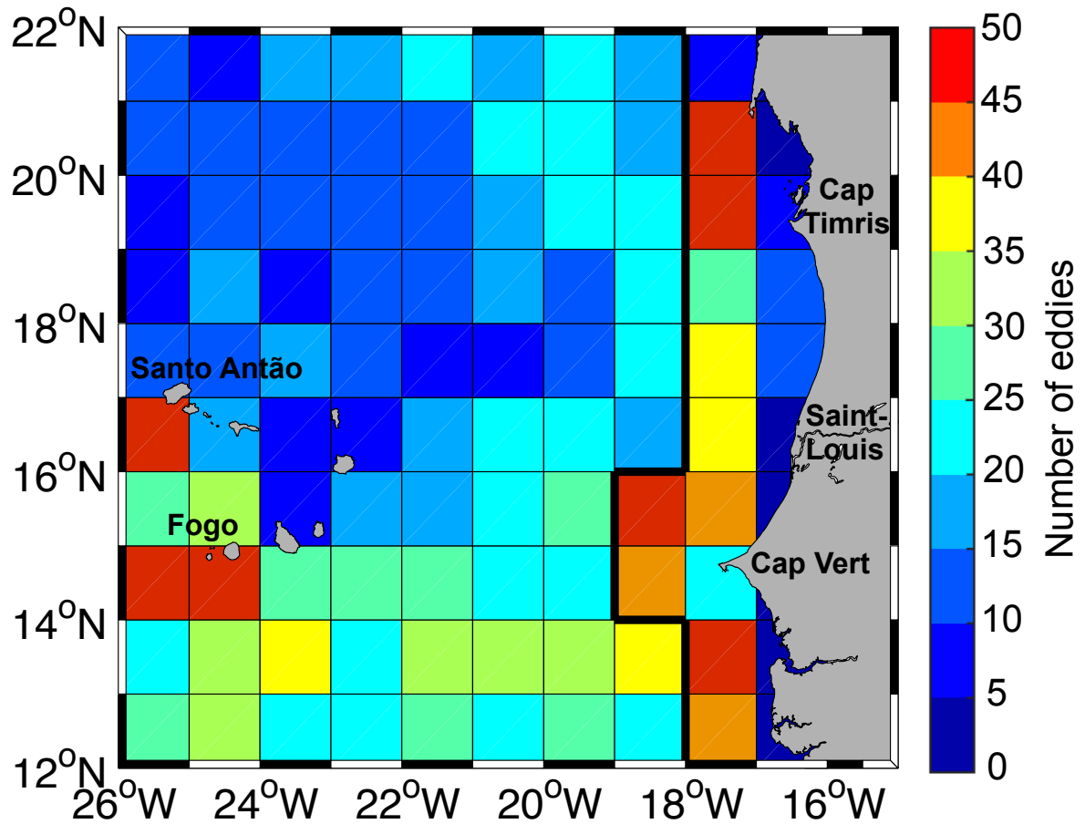
2 Figure 7: Number of eddies generated in 1^\circ \times 1^\circ boxes (colors) between 1995 and 2013 based on the results of 3 the OW-method. Marked are the headlands Cap Timiris (Mauretania), Saint-Louis (Senegal), Cap Vert (Senegal) 4 and the Islands Santo Antão (Cape Verde) and Fogo (Cape Verde), which can be associated with high eddy 5 generation. The thick solid black line along 18^\circ\text{W}/19^\circ\text{W} separates the coastal region from the offshore region. 6
