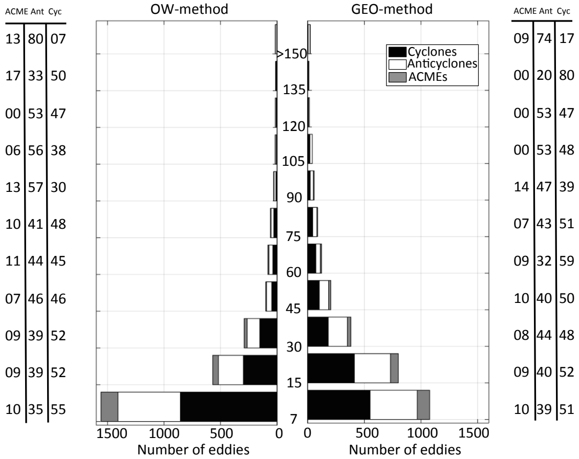
2 Figure 6: Number of eddies against lifetime in days from the OW-method (left) and GEO-method (right). 3 Percentage of ACMEs, anticyclones (Ant) and cyclones (Cyc) is given in the tables on the right and left.
