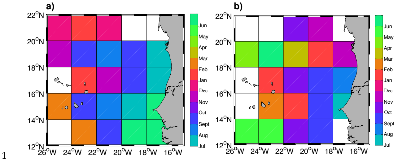
2 Figure 10: Phase of the annual harmonic of the number of detected eddies in 2^\circ \times 2^\circ boxes based on the results 3 of the OW-method for a) cyclones and b) anticyclones. Phases are only shown for boxes with an amplitude 4 larger than 2.5 eddies. Phase is given in month of the year with maximum eddy number. 5
