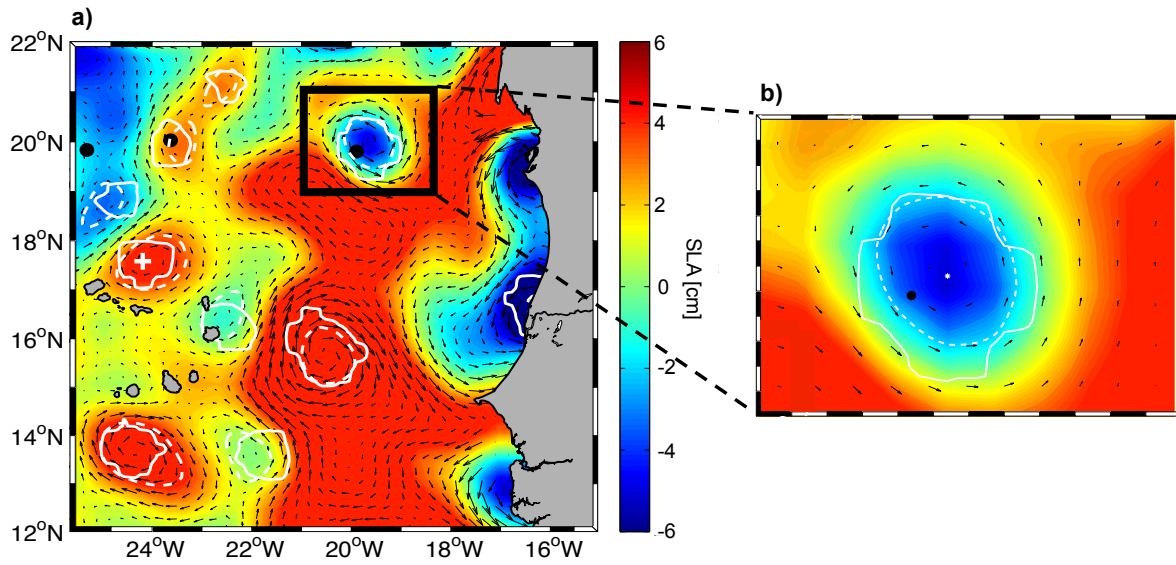
Figure 4: Snapshot of the SLA for Dec. 22, 2010, with the results of the eddy-detection methods: OW-Method (solid white line) and the GEO-Method (dashed white line) with geostrophic velocities superimposed (black arrows). The black dots mark Argo float profiles, the white cross in a ) indicates the CVOO mooring. In b ) a zoom of a selected region with a cyclonic eddy is shown.
