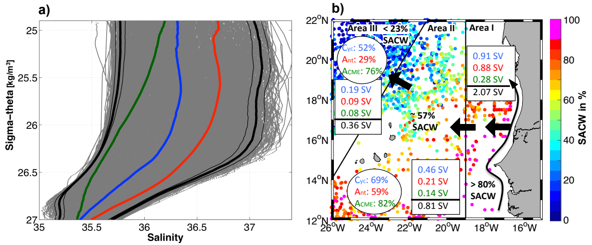
2 Figure 16: a) S- \sigma_0 diagram with thick and thin black lines indicating mean and standard deviation, respectively, 3 of characteristic SACW and NACW properties derived from the ensemble of profiles taken in the TANWA 4 (grey lines). Mean eddy dependent watermass properties are given for cyclones (blue line), anticyclones (red 5 line) and ACMEs (green line). b) Percentage of SACW in the upper 350m as shown for all available profiles 6 (color) and as mean numbers for the three regions: the extended boundary current region (Area I), the transition 7 zone (Area II) and the subtropical gyre region (Area III) that are separated by black straight lines. Numbers in 8 the white circles are the mean percentage of SACW of the composite cyclones (blue), anticyclones (red) and 9 ACMEs (green) in the corresponding areas. The eddy transport of SACW from the boundary current into Area I, 10 from Area I into Area II and from Area II into Area III is marked by thick black arrows with transport numbers 11 in Sv given in the white boxes for composite cyclones (blue), anticyclones (red), ACMEs (green) and total 12 transport (black).
