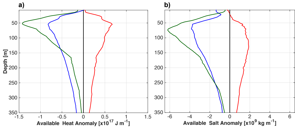
2 Figure 13: Mean profiles of available a) heat and b) salt anomaly per meter of the composite cyclone (blue line), 3 anticyclone (red line) and ACME (green line). 4
