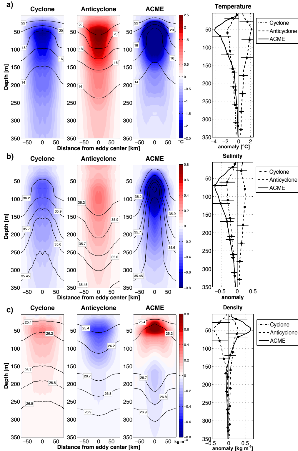
2 Figure 12: Vertical structure of the composite cyclone, anticyclone and ACME in the TANWA as presented as 3 sections through the eddy center (left three columns) and mean anomaly profiles (right column). In a) potential 4 temperature anomaly, in b) salinity anomaly and in c) potential density anomaly as calculated by using the 5 nearest profile outside of the eddy is shown. Black contour lines in the left three columns mark isolines of 6 temperature ( a ), salinity ( b ) and potential density ( c ). In the right column, solid lines represent the composite 7 ACME, dashed lines the anticyclone and dashed-dotted lines the cyclone; the error bars at selected depths 8 represent the standard deviation calculated from the individual anomaly profiles. 9
