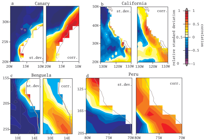
Figure 3. Correlation patterns between the seasonal (June–August, except for Benguela September–November) upwelling field in each Eastern Boundary Upwelling System and the simultaneous spatial mean alongshore wind stress (right panels) and the relative standard deviation of the upwelling field (left panels) simulated in one of the past 1000 simulations ( r_1 ) (900–1849) with the Earth System Model MPI-ESM.
