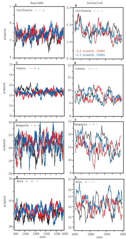
Figure 6. Time series of the simulated upwelling indices in each upwelling region simulated in two ensembles of climate simulations (three members each), denoted past1000 (900–1849) and historical (1850–2005), with the MPI-ESM model. The plus and minus signs in each panel indicate the sign of the long-term trend, their value being included whenever statistically significant. The series have been low-pass filtered with a 30 year filter for past1000 and a 10 year filter for the historical ensembles.
