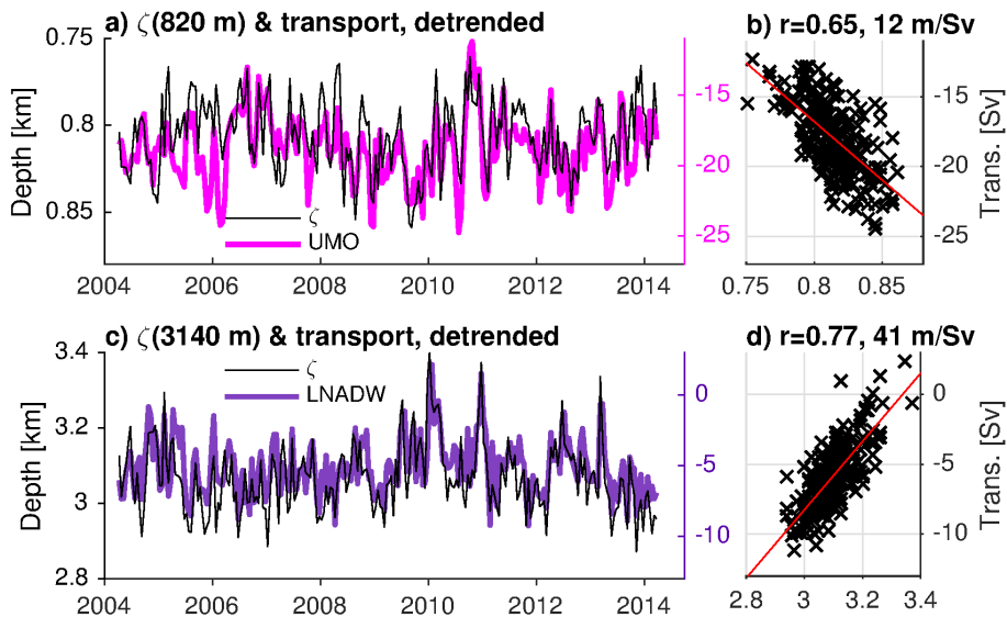
Figure 8. Time series of deseasonalized , detrended transports and isopycnal depths. (a) UMO transport (magenta) and the depth of the density surface with mean position at 820 m (highest correlation with UMO) at the west. (c) LNADW transport (purple) and the depth of the density surface with highest correlation (at 3140 m). Scatter plots are shown in (b, d) , where the least squares linear regression is overlaid.
