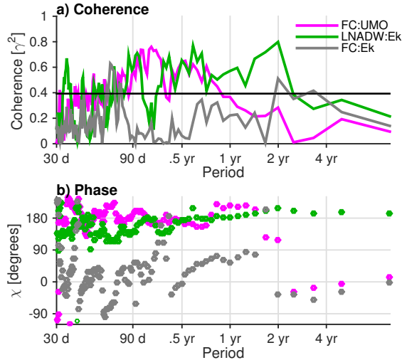
Figure 9. Coherence between MOC components: UMO and FC (magenta), LNADW and Ekman (purplegreen) and FC and Ekman (grey), where time series are the original 10 day filtered (seasonal variations retained). The top panel shows coherence, where significance is delimited by the black horizontal line. The lower panel shows the phase relationship at each period in degrees.
