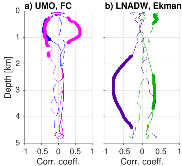
Figure 7. Correlation between isopycnal displacements at each depth and transport time series, where time series are deseasonalized and detrended. (a) Correlation between UMO (magenta) and isopycnal displacements at the west (solid) and east (dashed), and between FC (blue) and isopycnal displacements at the west (solid) and east (dashed). Significant correlations are indicated by the thicker line. (b) The same, but for LNADW (purple) and Ekman (green).
