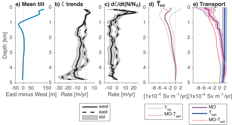
Figure 11. Trend in isopycnal displacements and transports. (a) Mean height difference between isopycnals in the east and west. (b) Trend in isopycnal displacements at the western and eastern boundaries, where a negative (positive) trend indicates downward (upward) movement of isopycnals. The solid (dashed) line is for displacements at the west (east). (c) Trend in displacements scaled by buoyancy frequency with N_0 = 1 \times 10^{-3} \text{ s}^{-1} . (d) Trend in \tilde{T}_{\text{int}} from Eq. (2). The red line is the trend in \text{MO}(z) - T_{\text{ext}} . (e) Trends in transport-per-unit-depth of mid-ocean ( \text{MO}(z) ) in magenta, T_{\text{ext}} in blue. All time series were twice-monthly. Confidence intervals on the trends are shaded. The dotted line shows a zero trend.
