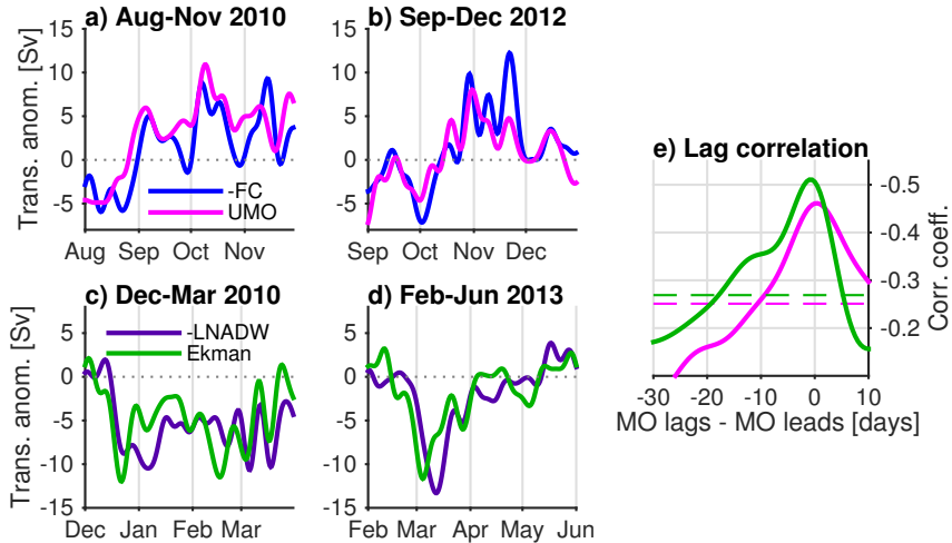
Figure 6. Ten-day filtered transport anomaly time series of UMO and FC ( a, b ) and LNADW and Ekman ( c, d ). The ten-year mean has been removed, but the seasonal cycle and trends are retained. Time ranges have been chosen to correspond to large anomalies in both time series, to visualize possible lags. ( e ) Lag correlation between ten-day filtered UMO and FC (magenta) and Ekman and LNADW (green). 95 % significance is marked by the dashed lines, same color.
