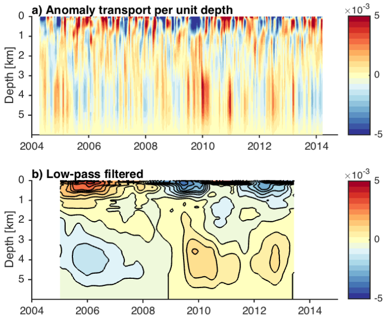
Figure 2. Transport-per-unit-depth anomalies of the mid-ocean transport at 26° N, where the time mean profile over the ten years has been removed. (a) The top panel shows the twice-monthly, deseasonalized variability and (b) the lower panel is further deseasonalized and filtered with the 1.5 year filter. Red (blue) shows transports which are anomalously northward (southward).
