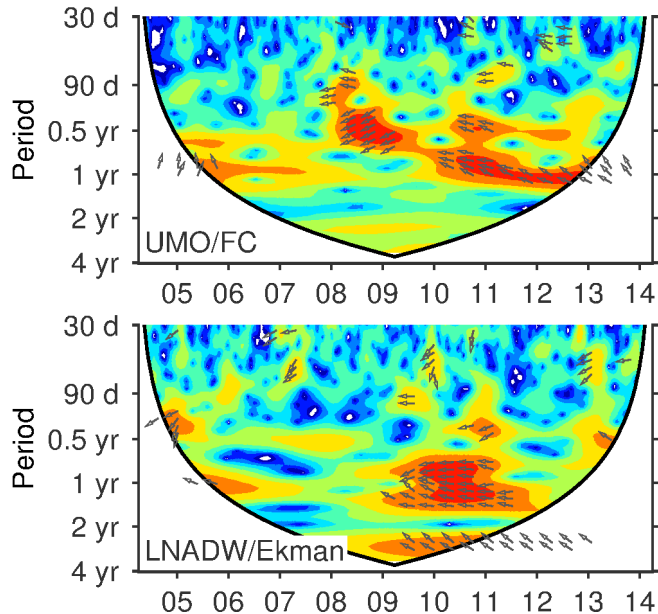
Figure 10. (a) Cross wavelet transform between the FC and UMO shows high power (red) with a fixed phase-relationship since 2007 at periods between 60–400 days. (b) Cross wavelet transform between Ekman and LNADW shows high power primarily at annual periods during the 2009–2010 events, as well as sub-annual from 50–150 days in 2005, 2011, and 2013 (Arrows pointing to the left indicate out-of-phase relationship or anti-correlation, and are only shown when the relationship is significant . Deviations from 180^\circ indicate a lag or phase shift.).
