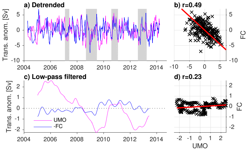
Figure 4. Transport anomaly time series (left column) for the FC (blue) and UMO (magenta). Zero anomaly is marked with the dashed line. Scatter plots of the same (right column) with correlation coefficients ( r ) noted. In (a, b) , the deseasonalized , detrended time series are used. In (c, d) , the time series are further deseasonalized and low-pass filtered, but not detrended . The orthogonal regression line is overlaid on the scatter plots. Grey bars highlight periods noted in the text.
