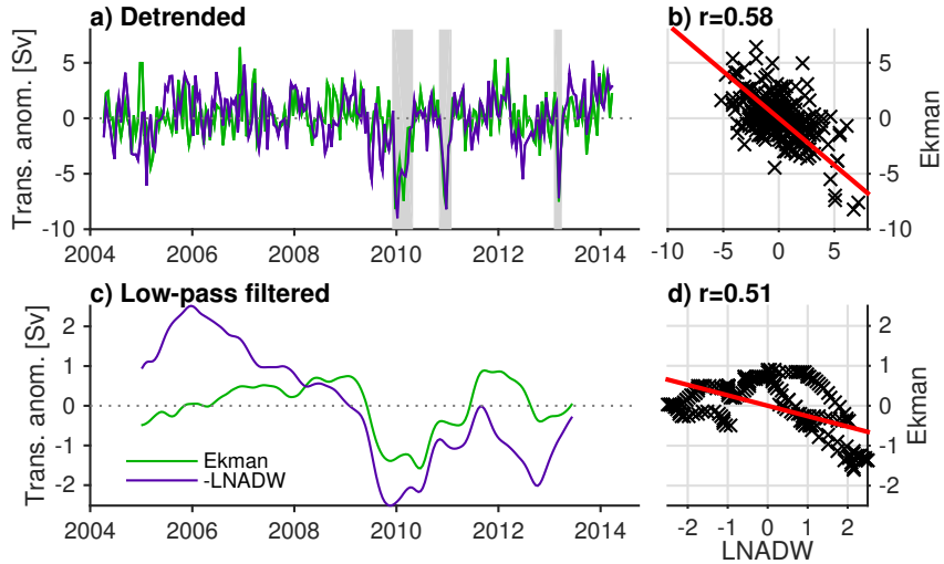
Figure 5. As Fig. 4 but for the Ekman and -LNADW transport anomaly time series.
