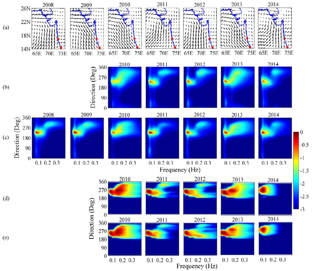
492 Figure5: Averaged wind pattern of October from 2008 to 2014 (row a). Averaged measured 493 wave frequency-directional spectra from 2008 to 2014 off Ratnagiri (row b) and off 494 Honnavar (row c) color bar is for spectral energy ( \text{m}^2 \cdot \text{Deg} / \text{Hz} ) d) Modeled directional 495 spectrum off Ratnagiri and (e) off Honnavar from 2010 to 2014. The spectral energy is shown 496 in logarithmic scale base to 10. SST anomalies of eastern and western equatorial IO with 497 DMI are shown in Figure 4.
