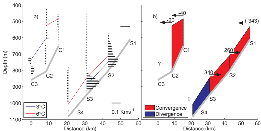
Figure 12. (a) Observed mean eddy temperature fluxes \overline{v'T'} at mooring array C and S (black bar) and the deployment mean position of the 3 °C (blue line) and 6 °C (red line) isotherm. The bottom is shown in grey and the scale for the temperature fluxes is given in the lower right corner. (b) Net eddy heat flux (10 5 W m -1 ), integrated up to the deployment mean position of the 6 °C isotherm (red line in a). The colors indicate convergence (red) and divergence (blue) and the arrows show the direction of the flux while the numbers above the moorings give the magnitude.
