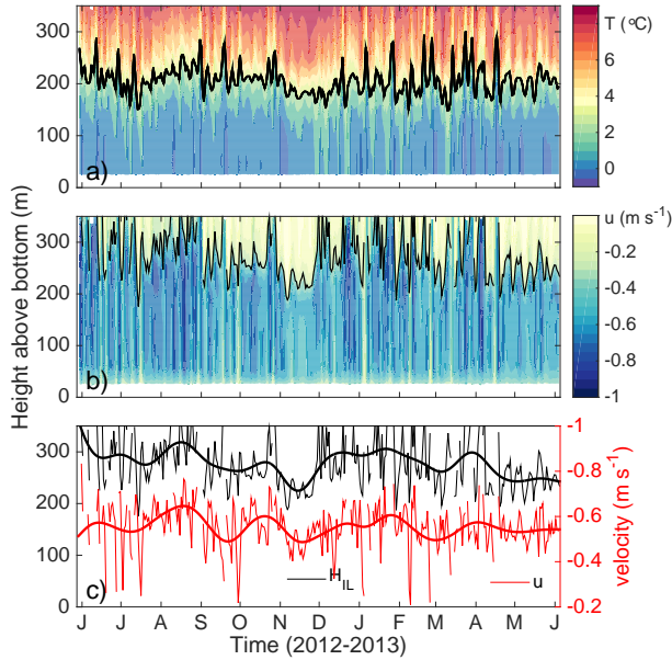
Figure 5. Time-height plots of daily (a) temperature ( ^\circ\text{C} ) and (b) u velocity ( \text{m s}^{-1} ) from mooring C2. The bold black line in (a) marks the 3^\circ\text{C} isotherm, and the thin black line in (b) is the kinematic interface height H_{IL} . (c) Time series of daily (thin) and 3 week low-passed (bold) H_{IL} (black) and the plume velocity (red) averaged within H_{IL} .
