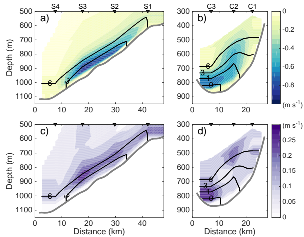
Figure 4. Cross-sectional distribution of alongstream velocity u ( \text{m s}^{-1} ), in colour, with average isotherms ( ^{\circ}\text{C} ) overlaid as black contours. Time-average ( a , b ) and standard deviation ( c , d ) of daily data over the common period 30 May 2012–17 January 2013 when complete records exist at both sections: ( a , c ) section S, and ( b , d ) section C.
