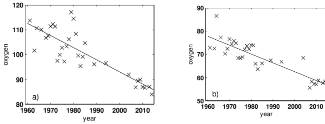
2 Figure 7. Mean dissolved oxygen concentration time series ( \mu\text{mol kg}^{-1} ) for the area 10\text{-}14^\circ\text{N} , 3 20\text{-}30^\circ\text{W} with fitted linear trend and 95% confidence interval for (a) 100\text{--}300\text{ m} ( -0.49 \pm 4 0.16 \mu\text{mol kg}^{-1} \text{ year}^{-1} ) and (b) 300\text{--}700\text{ m} ( -0.35 \pm 0.16 \mu\text{mol kg}^{-1} \text{ year}^{-1} ).
