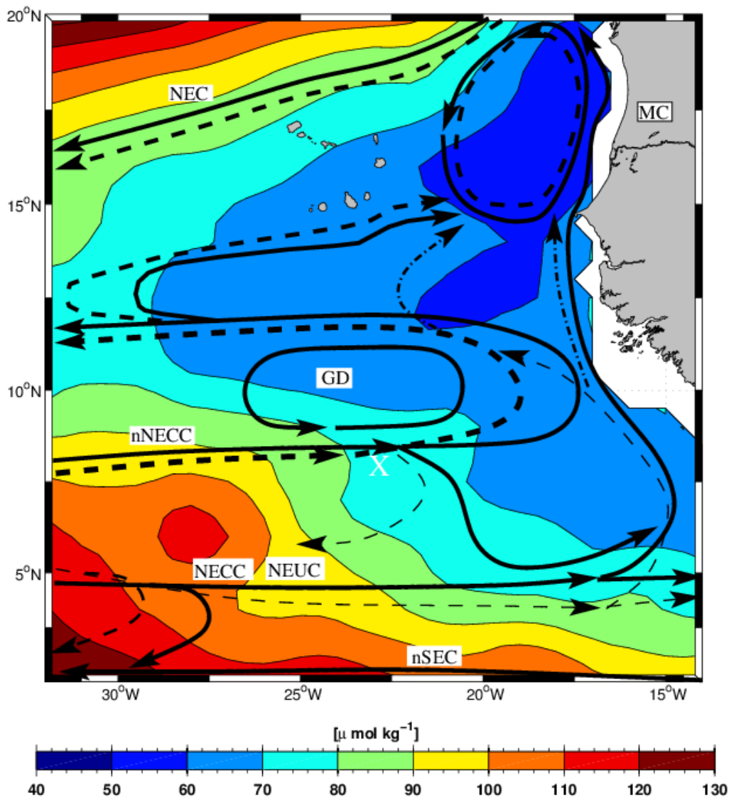
11 Figure 12. Schematic flow field based on the results from this investigation and on earlier 12 schematics (e.g. Mittelstaedt, 1983; Stramma and Schott, 1999; Stramma et al., 2008b; Peña-
