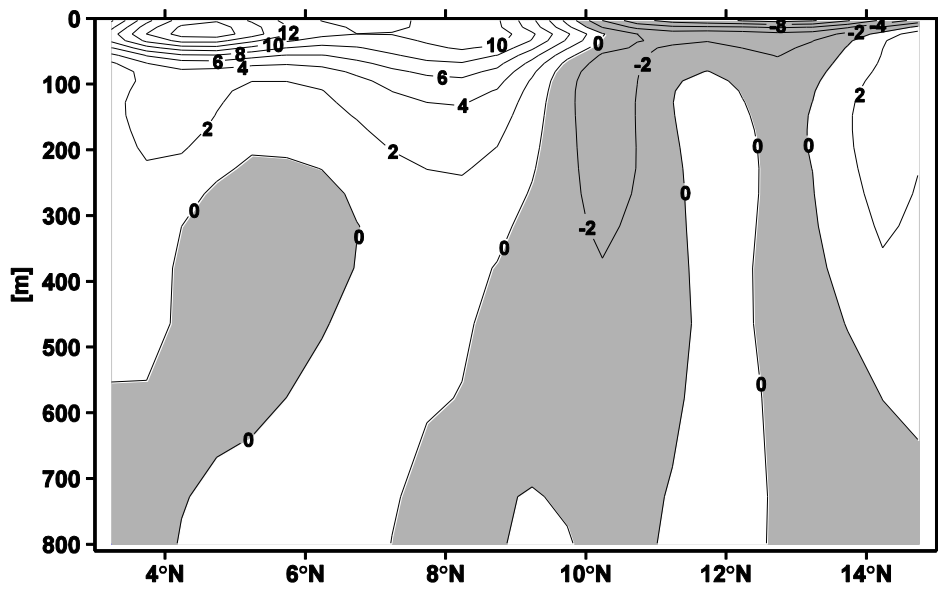
2 Figure 3. SODA model mean velocity section in \text{cm s}^{-1} for the period 2001 to 2010 along 3 23^\circ\text{W} (positive eastward).
