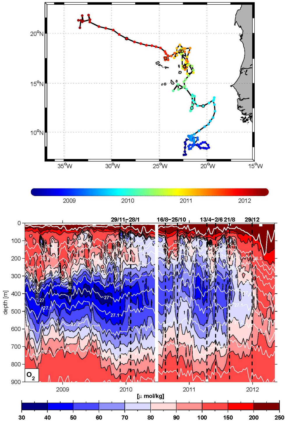
1 2 Figure 9. Measurements of float f350 in the tropical eastern North Atlantic between April 3 2008 and May 2012 with float path (color coded) in time (top) and oxygen distribution 4 (bottom) in \mu\text{mol kg}^{-1} (color) vs. time in the upper 900 m, density contours are marked in 5 white, the mixed layer depth defined for the depth where the density is 0.125 \text{ kg m}^{-3} larger
