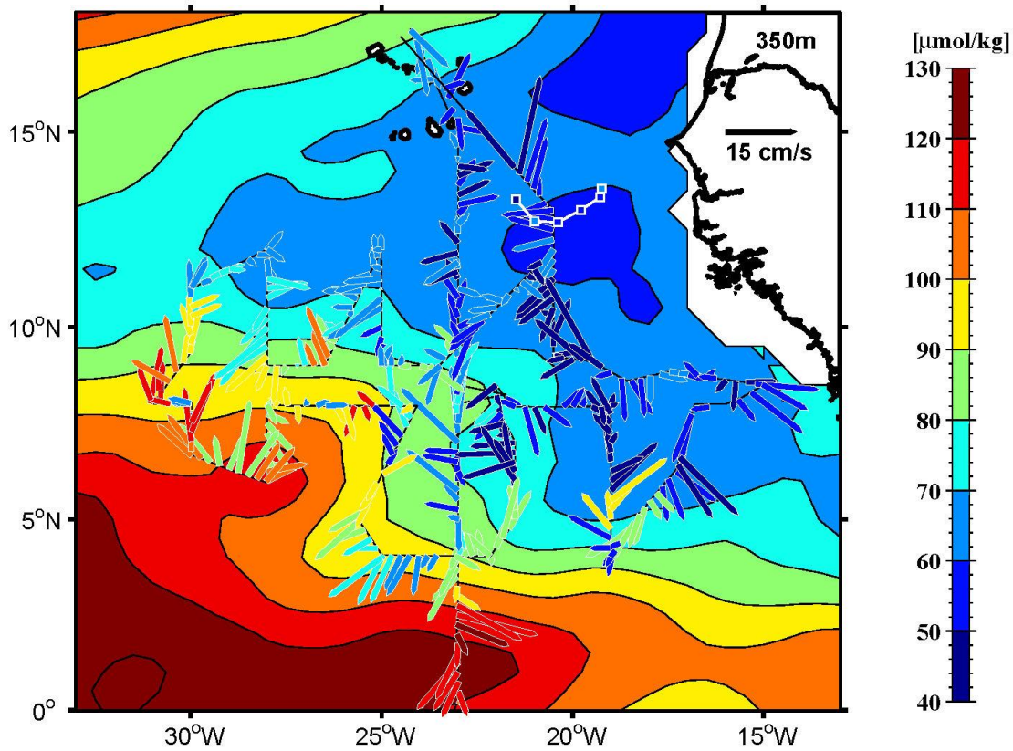
1 2 Figure 6. Horizontal distribution of ADCP velocity vectors converted to 350 m depth 3 recorded in November and December 2009 with current vectors colored with oxygen (in \mu\text{mol} 4 \text{kg}^{-1} ) of the accompanying CTD oxygen measurements at this depth. The oxygen distribution 5 of the background field is from CARS 2009 climatology (Ridgway et al., 2002) for the mean 6 of the November and December distribution at 350 m depth. The float track (white line) and 7 surfacing location (white squares) drifting at 350 m depth and the oxygen measured by the 8 float at 350 m depth (color in the square) is shown for the months November and December 9 2009.
