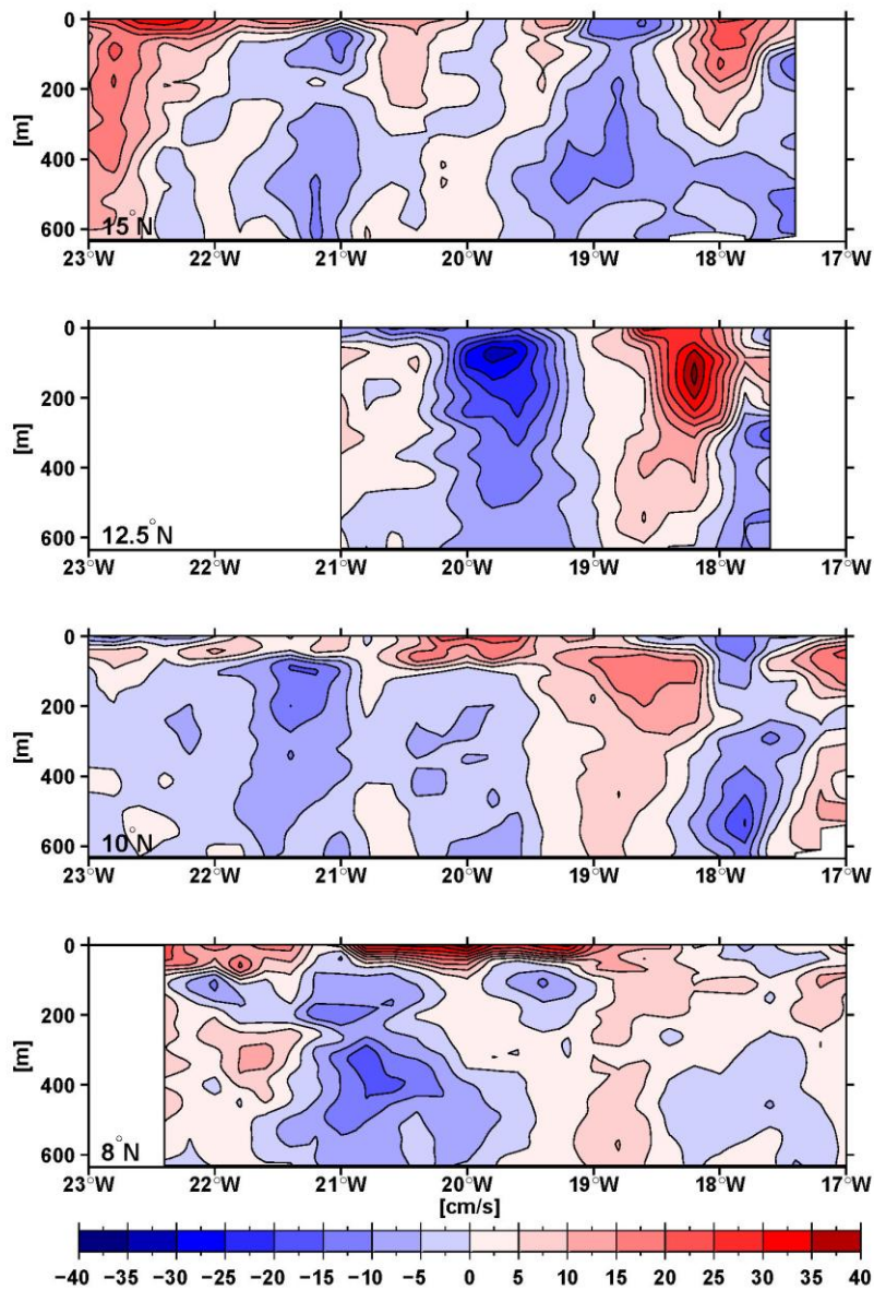
1 2 Figure 5. Meridional velocity component in \text{cm s}^{-1} (positive northward) at about 15^\circ\text{N} east of 3 23^\circ\text{W} , at 12.5^\circ\text{N} east of 21^\circ\text{W} at 10^\circ\text{N} east of 23^\circ\text{W} and at 8^\circ\text{N} east of 22.4^\circ\text{W} and west of 4 17^\circ\text{W} all measured in October 2010 (cruise tracks can be seen in Fig. 11).
