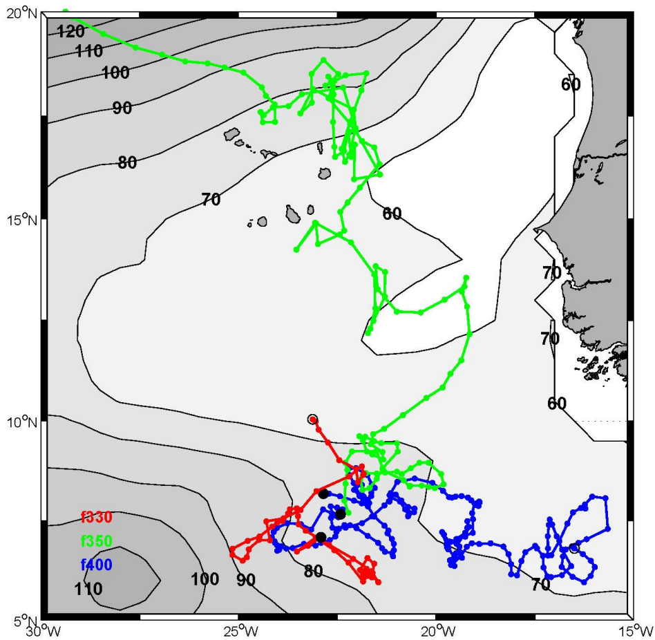
1 2 Figure 8. Annual mean climatological oxygen distribution (grey shaded contours, \mu\text{mol kg}^{-1} ) 3 at 350 m depth from CARS 2009 climatology (Ridgway et al., 2002) with trajectories (in 4 color) of three floats deployed in April 2008 (red 330 m (f330), green 350 m (f350), blue 400 5 m (f400)). First measurement cycle is shown as solid dot and the last cycle as open circle 6 (Table 1).
