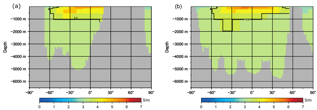
Figure 2. Meridional sections of sea-water conductivity distribution at 90° E (a) and 182° E (b) . Ocean depth is given in m. The black contour line indicates the mean conductivity of 3.5 \text{ S m}^{-1} .
