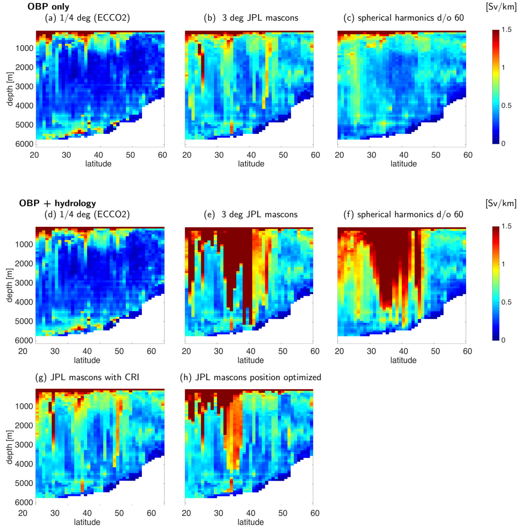
Figure 5. RMS errors for the computed transport-per-unit-depth T in [Sv/km] from eastern and western boundary OBP according to Eq. 3. OBP only (top row) and OBP + hydrology (second and third row) for each of the synthetic observation time series. Significant leakage errors are introduced with the GRACE-like resolutions (second row), CRI filtering of the mascons and optimizing their position in longitude can remove a major part of the leakage errors
