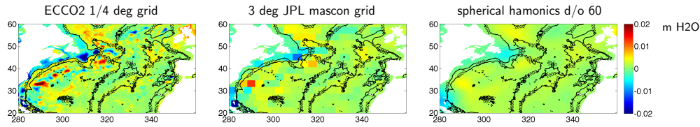
Figure 3. OBP snapshots for January 2012 for the different simulated OBP observation time series: left: 0.25^\circ ECCO2 resolution; center: GRACE JPL mascon resolution (approx. 3 deg); right: GRACE spherical harmonic resolution to spherical harmonic degree 60, smoothed with a 300 km Gaussian filter
