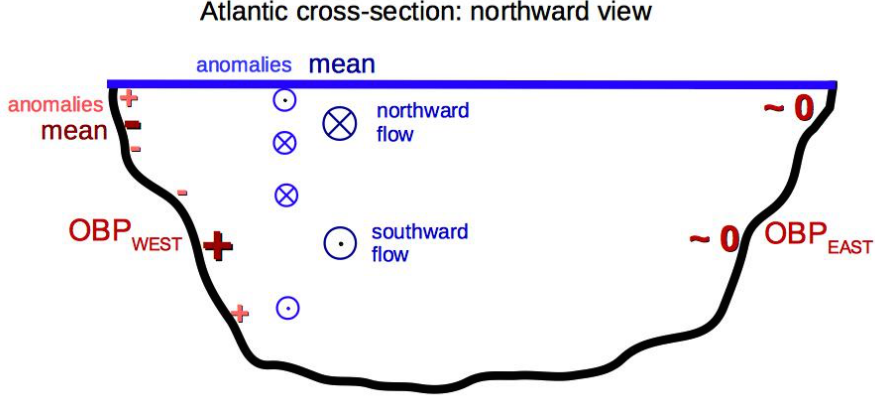
Figure 1. Cross-section of the North Atlantic with an illustration of north- and southward flow temporal mean and anomalies (blue) and associated ocean bottom pressure mean and anomalies (red) along the basin boundaries. Note that in the actual ocean, the bottom pressure signals are largest along the western boundary and the bottom pressure at the eastern boundary is very small and can be neglected. Ocean bottom pressure anomalies are observable with satellite gravimetry
