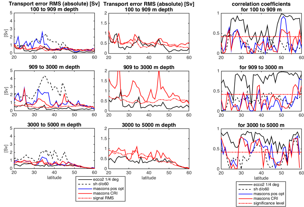
Figure 7. Error RMS and correlation coefficients for reconstructed net transport in three different depth layers and from different OPB resolutions (native ECCO2 grid vs. GRACE-like resolutions). Left: error RMS for the computed time series and RMS signal time series (red dashed); center: selection of two cases of error RMS and different scales on the plots; right: correlation coefficients of the derived time series versus the model truth, red dashed line indicates the 95% significance level
