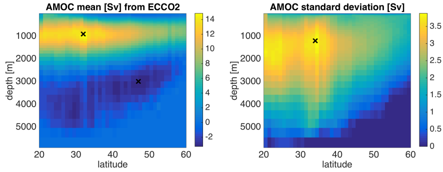
Figure 6. Left panel: Time mean of AMOC from ECCO2, with maximum at 32°N, 909 m depth, minimum at 47°N, 2990 m depth, both indicated marker X, right panel: variability of AMOC from ECCO2, maximum at 34°N, 1200 m depth, indicated by marker X
