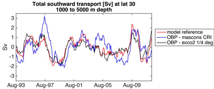
Figure 9. Comparison of AMOC transport anomalies at 30 N, reconstructed from OBP (blue and black lines) versus model baseline (red line; from velocities, RMS 0.92 Sv). The error RMS (relative to the baseline) for the mascon reconstruction is 0.90 Sv, and for the ECCO2 grid-OBP is 0.43 Sv. The correlation with the baseline transport is R=0.63 (mascon grid), and R=0.88 (ECCO2 grid-OBP)
