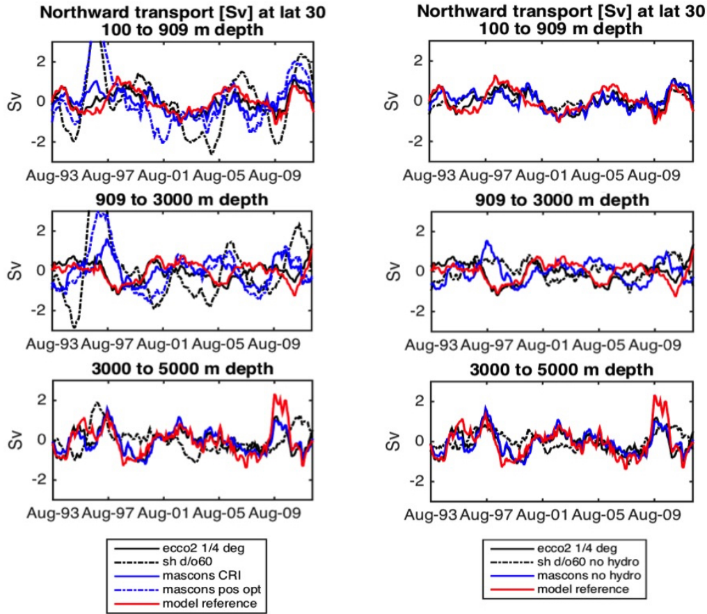
Figure 8. Transport time series anomalies at 30^{\circ}\text{N} , reconstructed from different OBP data sets versus the model baseline, left: including land hydrology signal, right: without land hydrology signal
