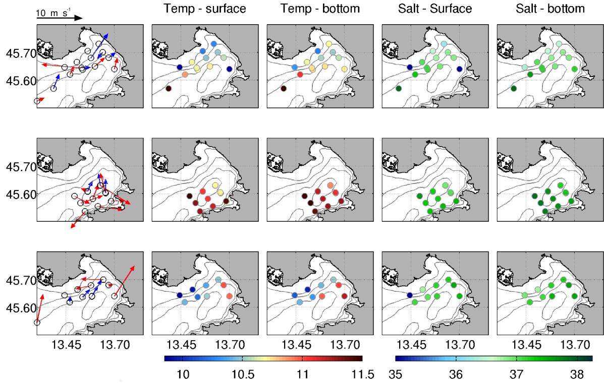
Figure 3: Bottom currents and values from CTD casts at surface and bottom are shown inside the GoT for January 30 th (top panels), January 31 st (central panels) and February 4 th (bottom panels). Panels on the left column show the ADCP bottom cell currents; red arrows are observations taken during rising tide, blue arrows during falling tide. Temperature (second and third columns) and salinity (fourth and fifth columns) values are shown for surface (0 and 2.5 m) and bottom layers (last 2.5m of cast) inside the GoT.
