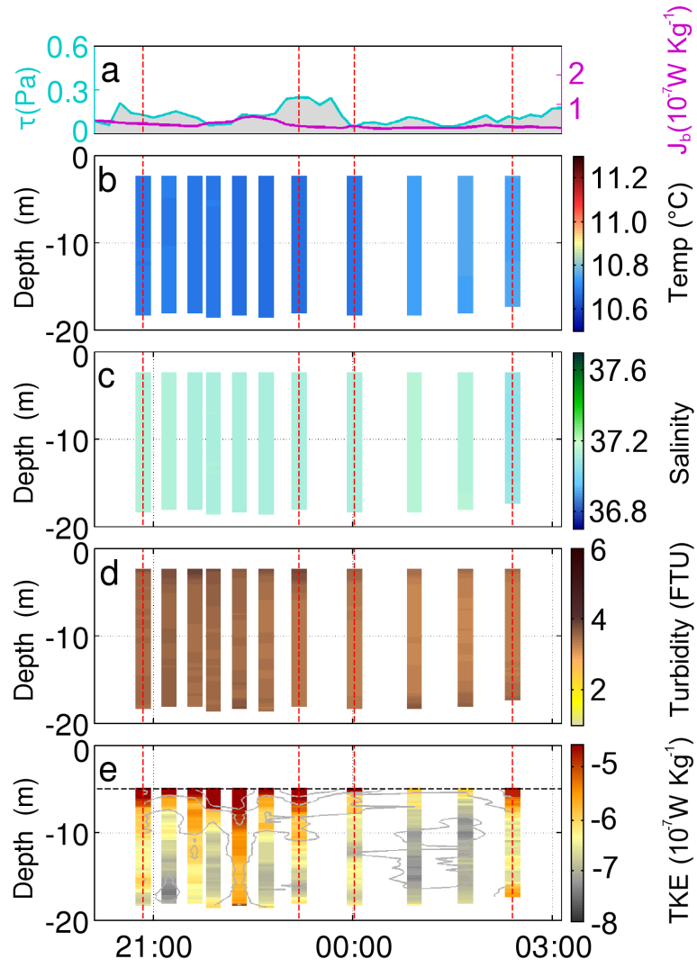
Figure 6: Hovmöller diagrams for Y01: a) wind stress and buoyancy flux during the Y01, b) temperature profiles; c) salinity profiles; d) turbidity profiles in FTU; e) turbulent kinetic energy dissipation rate in logarithmic scale (contours spaced in log of 1 \text{ W Kg}^{-1} ). Red dashed lines show the time of collection of the Y01 casts reported in top panels of Figure 8.
