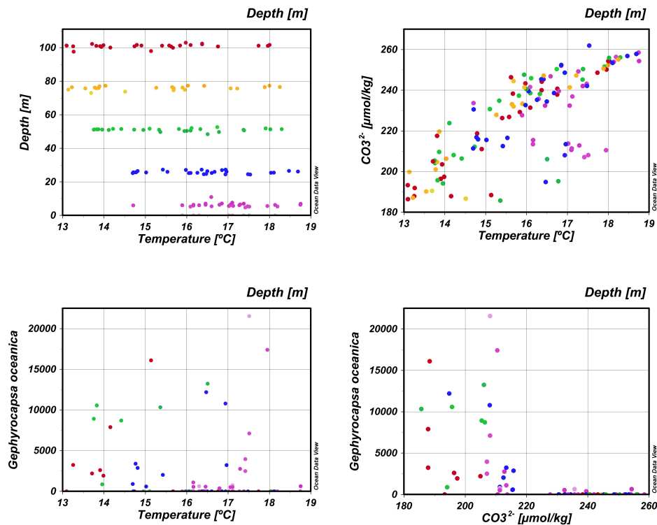
Fig. 1. Figure 1. Temperature against [CO 3 2- ] (upper-right) and G. oceanica cell density (cells/l) against [CO 3 2- ] and temperature (down). Colors indicate the depth of the sample as in the upper-left panel.
