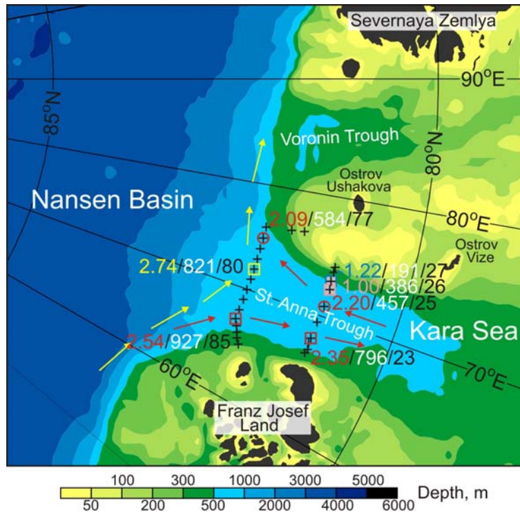
Fig. 2. A map of the northern Kara Sea with the St. Anna Trough ( ST ). Arrows show the Fram Strait branch of the AW inflow into the Arctic Ocean that recirculates in the ST (red arrows, SFSBW) and follows the continental margin (yellow arrows, FSBW). Crosses depict the positions of CTD stations taken in September 2009 at two sections crossing the ST at ~ 81°N and 82°N. Red squares and circles identify stations taken through the core of the SFSBW inflow and outflow to/from the ST , respectively. The yellow square identifies the station taken through the core of the FSBW boundary current. The pink square depicts the mooring position. The pink and blue squares with gray shading identify the stations used for estimates of uncertainty in the vertical heat flux due to spatial under-sampling of the AW jet. The first (yellow/red) number shows the FSBW/SFSBW core temperature (in °C) in September 2009. The first pink and blue numbers give the temperatures at 110 m. The second (white) number is heat content (in MJ m -2 ), computed relative to the freezing temperature, between 30 to 90 m depth. The third (black) number denotes the station number.
