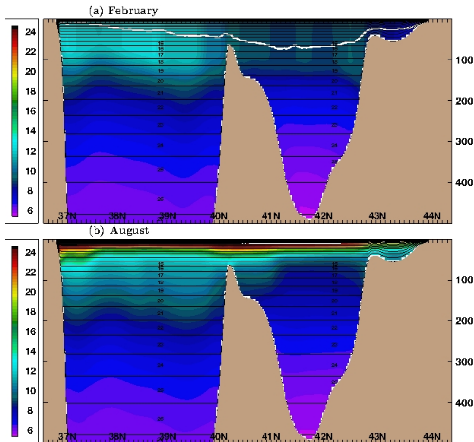
Fig. 1. Model derived monthly mean temperature at 50^{\circ}\text{E} (a) February (b) August
