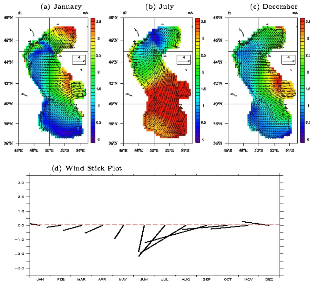
Fig. 2. Satellite derived wind pattern over the Caspian Sea from (Gunduz 2014).
