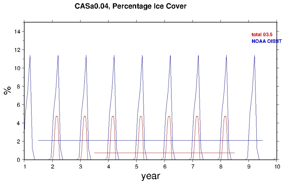
Fig. 3. Climatological ice concentration from model results vs observation.
