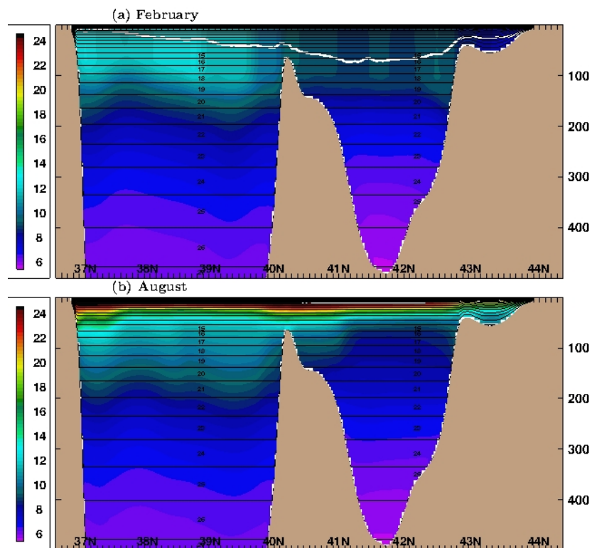
Fig. 1. Model derived monthly mean temperature at 50°E (a) February (b) August
