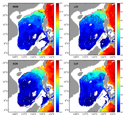
Figure A2. Seasonal variation of salinity (PSU) on 25.0 \sigma_0 surface from HYCOM data. The pink and black contours indicate the location of the 34.68 PSU contour and 34.6 PSU contour, respectively.
