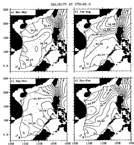
Figure A1. Seasonal variation of salinity (psu) on 25.0 \sigma_\theta surface.
