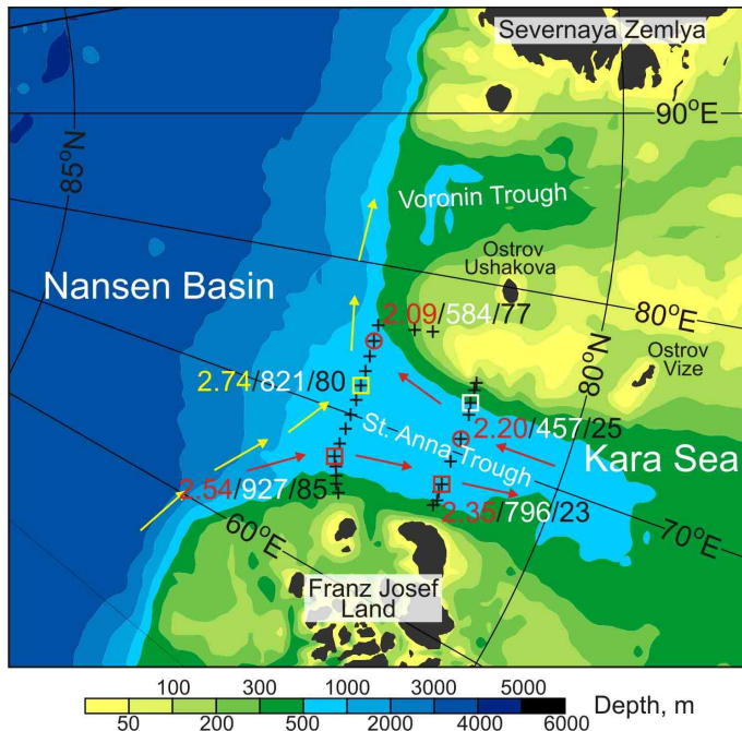
Fig. 2. A map of the northern Kara Sea with the St. Anna Trough (SAT). Arrows show the Fram Strait branch of the AW inflow into the Arctic Ocean that recirculates in the SAT (red arrows, SFSBW) and follows the continental margin (yellow arrows, FSBW). Crosses depict the positions of CTD stations taken in September 2009 at two sections crossing the SAT at \sim 81^\circ N and 82^\circ N. Red squares and circles identify stations taken through the core of the SFSBW inflow and outflow to/from the SAT, respectively. The yellow square identifies station taken through the core of the FSBW boundary current. The white square depicts mooring position. The first (yellow/red) number shows the FSBW/SFSBW core temperature ( ^\circ\text{C} ) in September 2009. The second (white) number is heat content ( \text{MJ m}^{-2} ) computed relative to the freezing temperature between 30 to 90 m depth. The third (black) number denotes station number.
