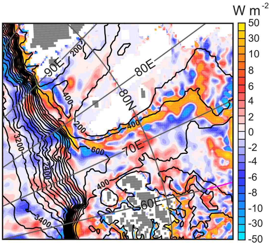
Fig. 8. The 7-year mean (2003–2010) simulated vertical heat fluxes ( \text{W m}^{-2} ) across the upper SFSBW interface at 75 m showing enhanced heat loss over the SAT eastern flank as well as over the Nansen Basin continental margin. Positive numbers indicate upward heat flux. The bathymetry is in meters.
