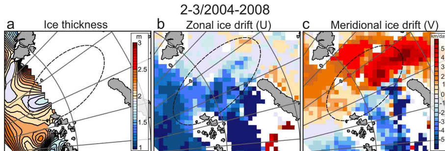
Fig. 9. The 2004–2008 winter mean (February–March) (a) seaice thickness (m) and (b) zonal and (c) meridional seaice drift ( \text{km day}^{-1} ) derived from AMSR data. The dashed oval highlights the SAT region.
