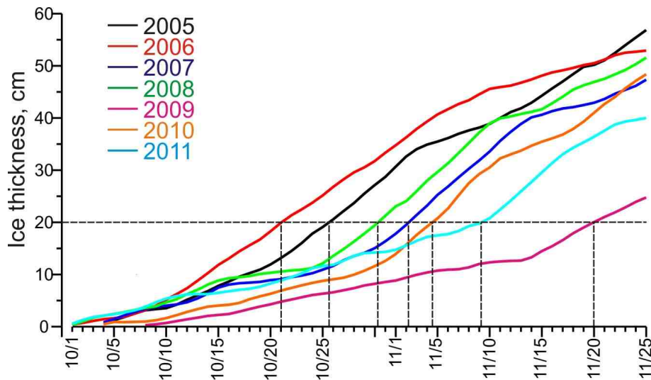
Fig. 11. Time series of accumulated thermodynamic seaice growth (cm) computed for October–November 2005–2011. Dashed lines indicate days in October–November when seaice thickness reached 20 cm.
