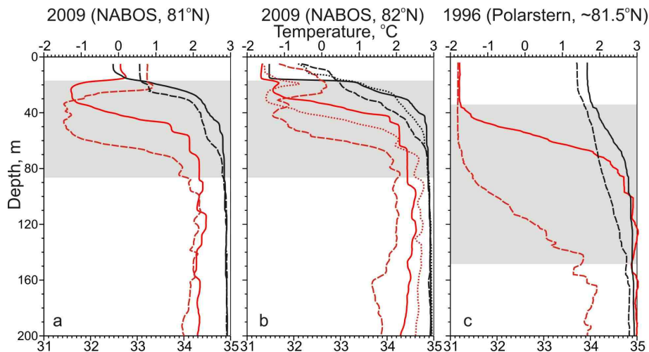
Fig. 4. Vertical profiles of temperature (red, °C) and salinity (black, psu) in the upper 200 m layer taken in July 1996 and September 2009 through the core of SFSBW inflow (solid line, left – st. 23, center – st. 85, right – 81^{\circ}27' \text{ N} , 65^{\circ}51' \text{ E} ) and outflow (dashed line, left – st. 25, center – st. 77, right – 81^{\circ}17' \text{ N} , 72^{\circ}01' \text{ E} ) to/from the SAT. (b) The dotted line depicts the CTD profile taken in September 2009 through the core of the FSBW boundary current (st. 80). For station positions in 2009 see Fig. 2. Gray shading highlights outflow from the SAT modified by vertical mixing.
