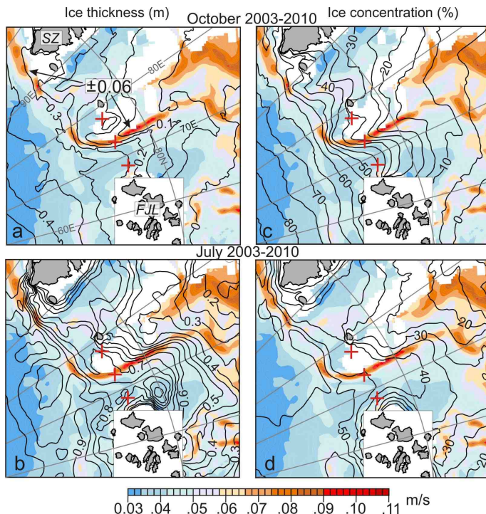
Fig. 7. The 7-year mean (2003–2010) simulated velocity difference ( \Delta V ) in the 0–75 m layer ( \text{m s}^{-1} ) in the northern Kara Sea with overlaid simulated mean ( a , b ) sea-ice thickness (m) and ( c , d ) concentration (%) for ( a , c ) October and ( b , d ) July. Crosses depict locations along 81^\circ\text{N} where the measured June–November time series of sea-ice concentration are compiled in Fig. 10. ( a ) Arrowed number shows \pm one standard deviation for the \Delta V maximum over the SAT eastern flank and Kara Sea continental margin obtained using monthly mean velocity data.
