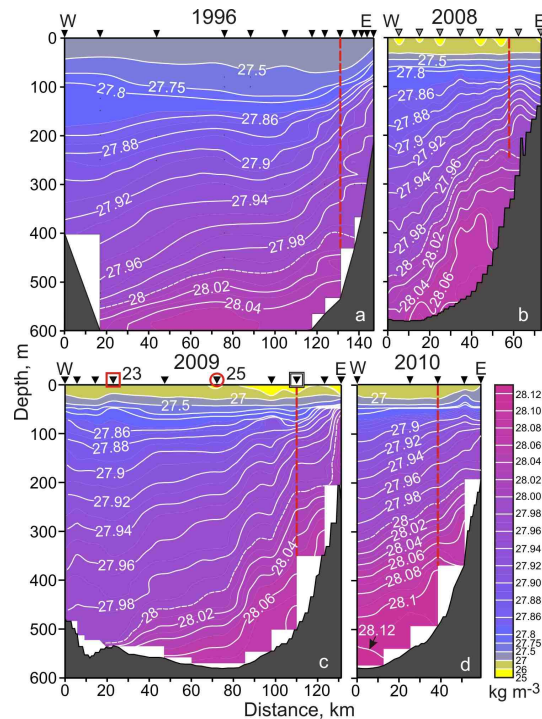
Fig. 5. 10 m binned cross-trough sections of potential density ( \sigma -zero, \text{kg m}^{-3} ) along 81^\circ \text{N} for (a) July 1996, (b) September 2008, (c) September 2009 and (d) October 2010. Black and gray triangles on the top identify positions of CTD and XCTD stations, respectively. Following Fig. 2, the red square and circle and the white square identify stations taken through the core of the SFSBW inflow and outflow to/from the SAT and mooring position, respectively, with their reference numbers on the top. Red dashed lines identify locations of the geostrophic velocity profiles shown in Fig. 6a. The white dashed line highlights \sigma -zero = 28 \text{ kg m}^{-3} that roughly corresponds to the core of the cooler fraction of BSBW (Dmitrenko et al., 2008, 2009).
