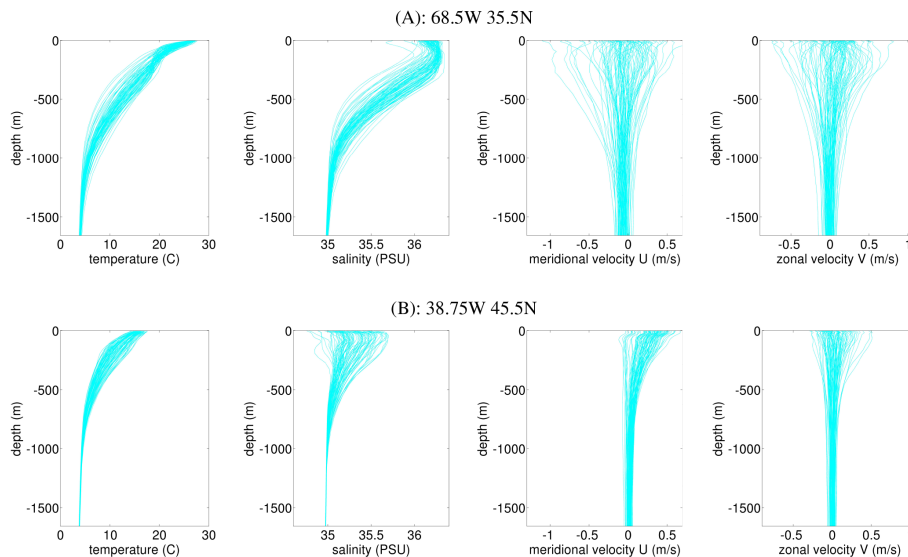
Figure 3. Local profiles, 96-member ensemble for temperature (1st column), salinity (2nd column), meridional (3rd column) and zonal (4th column) velocity, 9 July 2005.
