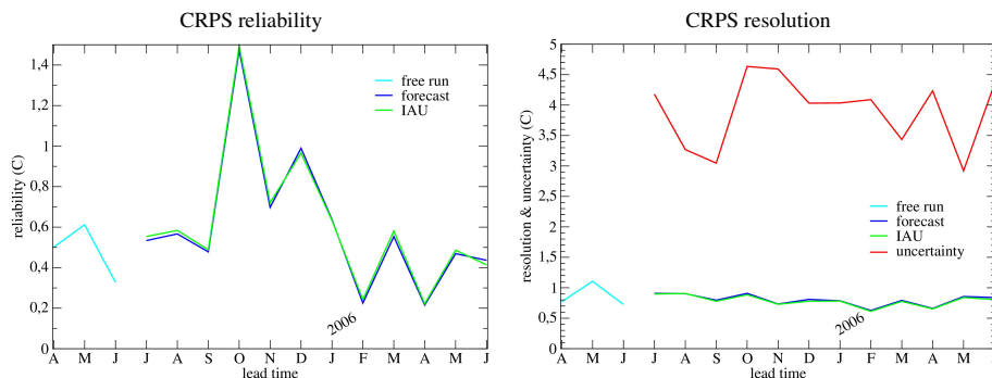
Figure 12. T profiles, reliability (left panel) and resolution component of the CRPS compared to the uncertainty (right panel).
