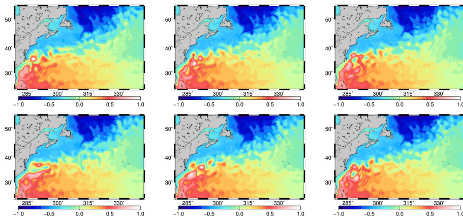
Figure 1. 6 members from the free run 96 member ensemble SSH (in m); snapshots for 9 July 2005.
