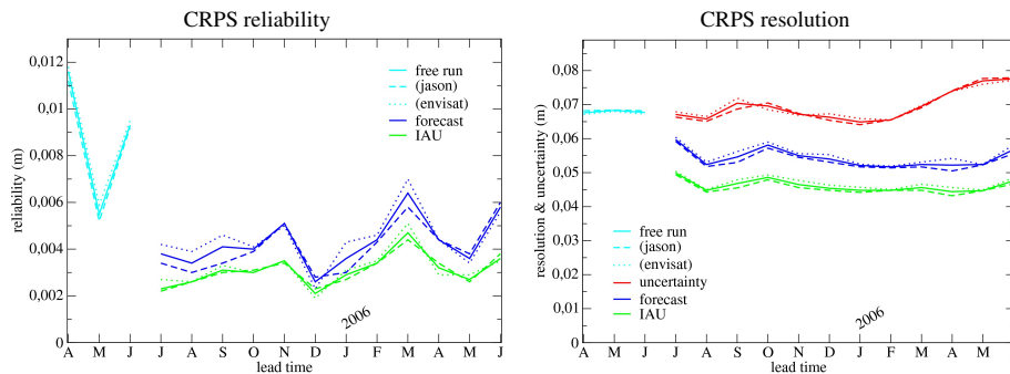
Figure 10. SSH: reliability (left panel) and resolution component of the CRPS compared to the uncertainty (right panel).
