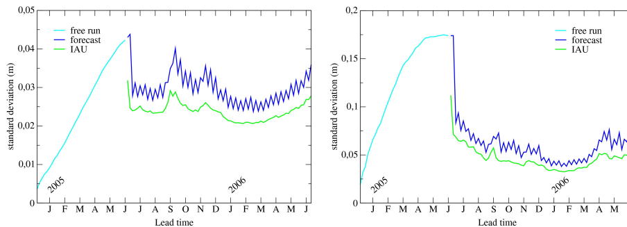
Figure 7. SSH time series of SDs for free run, forecast and IAU ensembles over the Gulf Stream verification area (left panel) and the Z-focus area (right panel).
