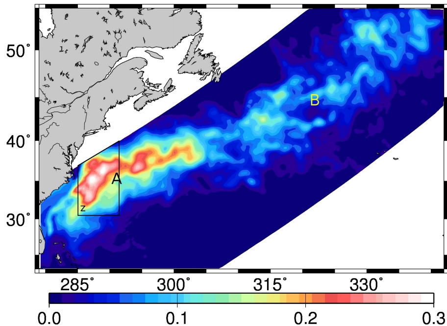
Figure 2. SSH SD (in m) for 9 July 2005. The figure also shows the verification area (in colour) used for the numerical diagnostics together with the smaller focus area Z. Points A and B are particular locations used for diagnostics discussed elsewhere in the paper.
