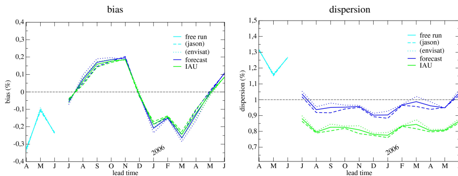
Figure 9. SSH bias (left panel) and dispersion (right panel) from RCRV.
