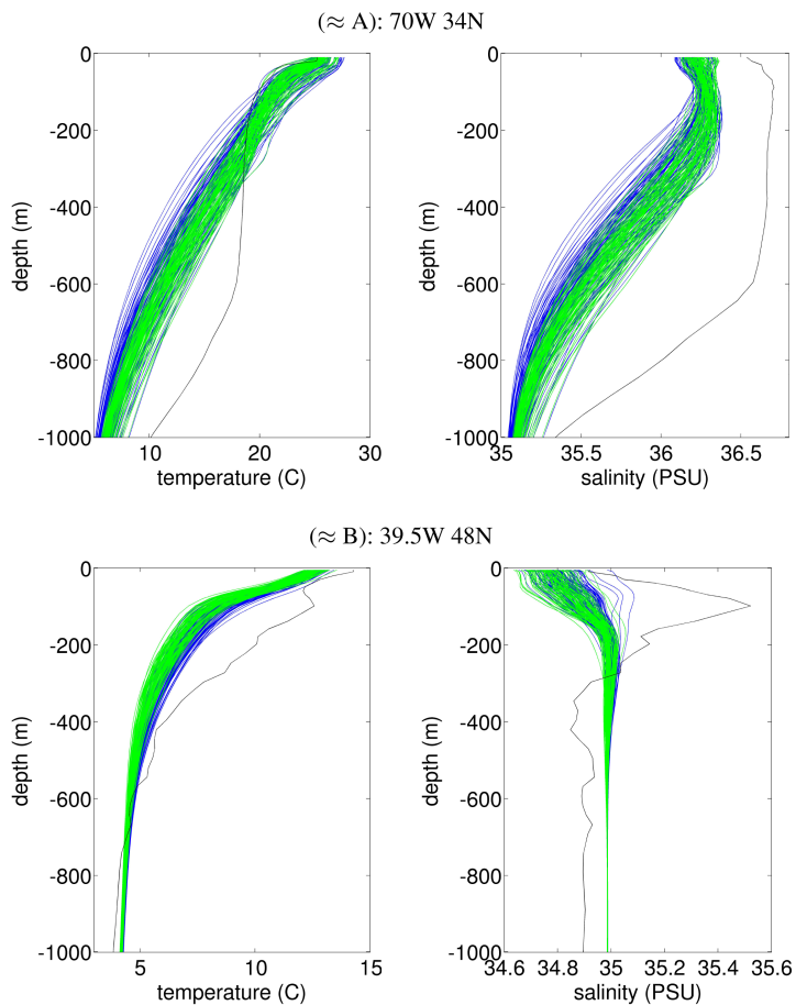
Figure 11. Impact of the altimetric correction on local T/S profiles ensembles during the first assimilation cycle: 3 July 2005 (top row) and 9 July 2005 (bottom row). Forecast ensemble (blue), IAU ensemble (green) and ARGO observation (black).
