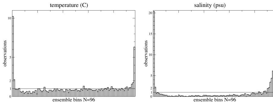
Figure 5. Global rank histogram of 0–200 m layer for temperature (left panel) and salinity (right panel); same period and same area as in Fig. 4.
