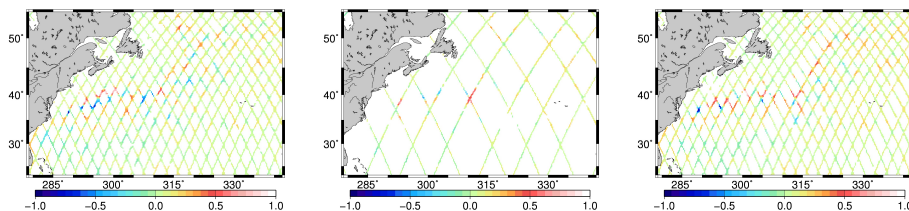
Figure 8. Jason-tracks coverage for 3 successive 10 day cycles from 7 September to 7 October 2005.
