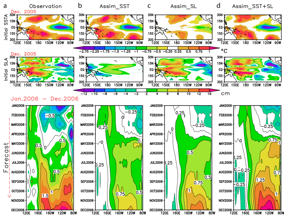
Figure 1. Initial conditions of anomalous sea surface temperature (SST; top row), sea level (SL; middle row), and forecasted SST anomalies (bottom row) from the (a) observations, (b) Assim_SST results, (c) Assim_SL results, and (d) Assim_SST + SL results, respectively. The initial fields are from December 2005, and the 12 month forecasts start in January 2006.
