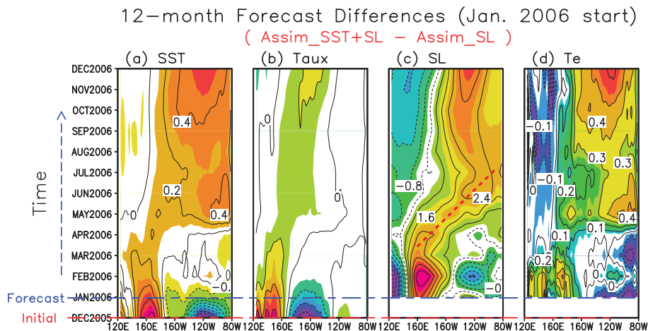
Figure 2. Initial and forecasted differences between the Assim_SST + SL hindcast and the Assim_SL hindcast for (a) sea surface temperature (SST), (b) zonal wind stress (Taux), (c) sea level (SL), and (d) temperature of the subsurface water entrained into the mixed-layer ( T_e ), illustrating the effects of the initial surface states, SST and Taux on predicting the 2006–2007 El Niño event. The dashed red line in (c) represents the propagation of the downwelling Kelvin wave. The contour interval is 0.2^\circ\text{C} in (a) , 0.08\text{ dyn cm}^{-2} in (b) , 0.8\text{ cm} in (c) , and 0.1^\circ\text{C} in (d) .
