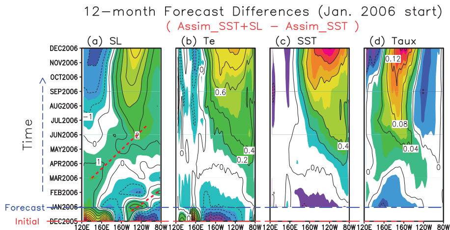
Figure 3. Initial and forecasted differences between the Assim\_SST + SL hindcast and Assim\_SST hindcast for (a) sea level (SL), (b) temperature of the subsurface water entrained into the mixed-layer ( T_e ), (c) sea surface temperature (SST), and (d) zonal wind stress ( Taux ), illustrating the effects of the initial subsurface states, SL and T_e on predicting the 2006–2007 El Niño event. The dashed red line in (a) represents the propagation of the downwelling Kelvin wave. The contour interval is 1.0 cm in (a) , 0.2 °C in (b) and (c) , and 0.04 \text{dyn cm}^{-2} in (d) .
