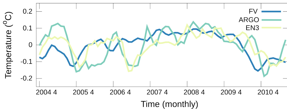
Fig. 1. Temperature, detrended and mean removed, for the domain used: 26-36oN, upper 800m. We show ARGO (green), EN3 (yellow) and our FV case (blue).
