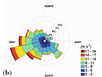
Gwynt Y Mor: cup anemometer at 64 m: Sept 05 - Apr 08
