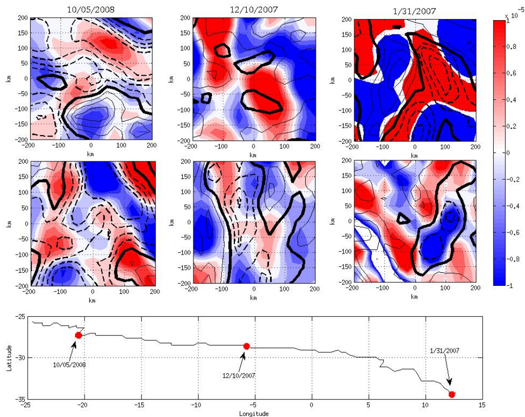
Fig. 2. Snapshots of (upper row) (color contours) and (black contours – c. i. 5 \times 10^{-6} °C per 100km), and (middle row) (color contours) and (black contours – c. i. 5 \times 10^{-6} °C per 100km). The thick black lines repr
