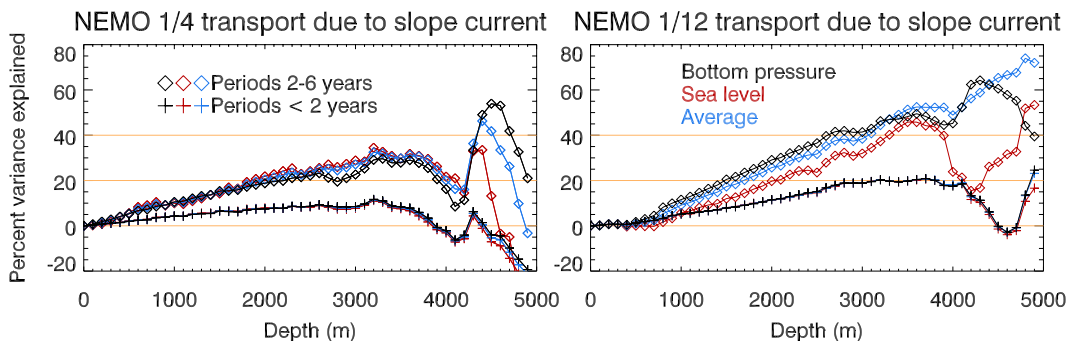
Fig. 5. Estimate of the percentage of total transport variance which is accounted for by flows on the continental slope, plotted as a function of the outermost depth contour to which the continental slope flow is integrated. The calculation is made for periods shorter (pluses) and longer (diamonds) than two years, and the currents are estimated by assuming they are barotropic flows associated with the circum-Antarctic average bottom pressure (black), sea level (red) or the average of the two (blue) along each depth contour. Left panel shows results from the 1/4^\circ model, and right panel the 1/12^\circ model.
