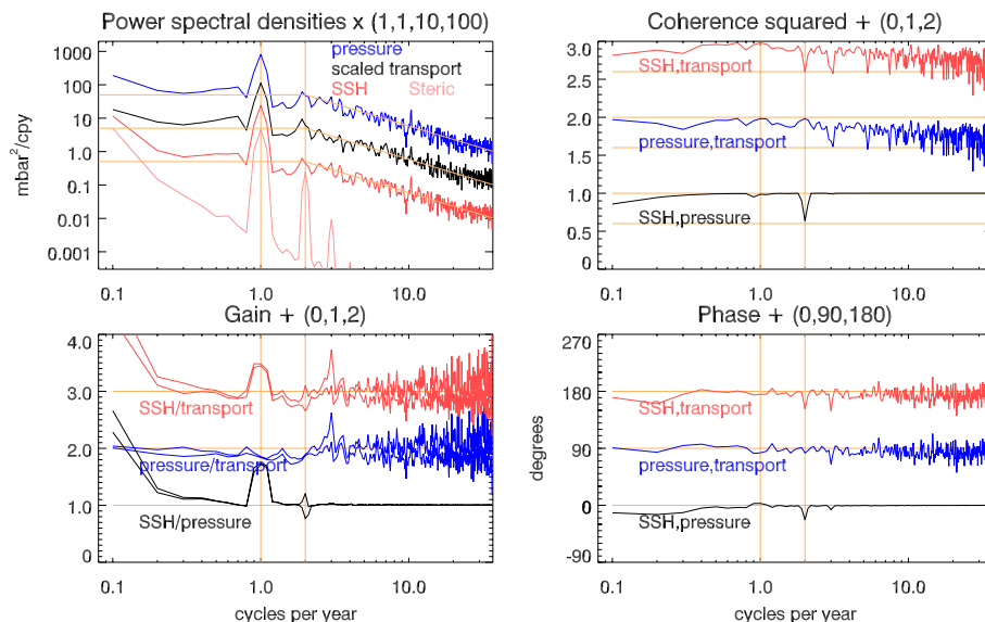
Fig. 3. Spectra and cross-spectral analyses based on time series from the 1/4^\circ model. Top left: power spectra for depth-averaged southern boundary pressure (blue), the analogous sea level (sub-surface pressure) time series (red), the difference sub-surface minus bottom pressure (pink), and Drake Passage transport divided by -3.69 \text{ Sv mbar}^{-1} . Other panels show the squared coherence, gain, and phase lag between pairs of these time series as described in the legends. Orange lines are for guidance and show the offsets applied to the different curves, as well as the annual and semiannual frequencies and, in the case of squared coherence, the value representing significance at the 95% level. Two versions of the gain are shown, representing ratios derived from regressions of a on b , and from b on a , where a and b are the two time series. When both time series contain noise, the true relationship between them tends to lie between these two estimates.
