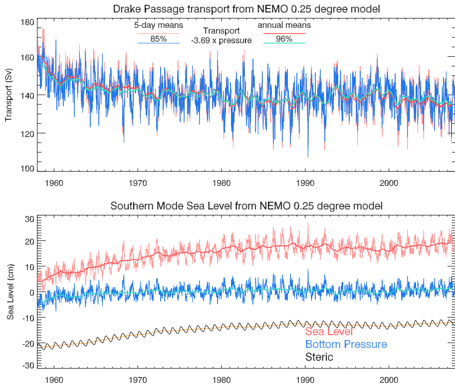
Fig. 2. Time series from the 1/4^\circ model. Top: flow through Drake Passage before (pink) and after (red) applying a running 12 month smoother, and -3.69 \text{ Sv mbar}^{-1} \times depth-averaged southern boundary pressure anomaly (blue and cyan), with a vertical offset applied to match. Bottom: the pressure time series used to plot the upper panel (blue and cyan), converted to equivalent sea level units, together with the analogous sea level time series (pink and red), and the difference sea level – bottom pressure (black and orange). Note, the curves are shown with trend, annual, and semiannual cycles included, although these are removed when calculating correlations etc.
