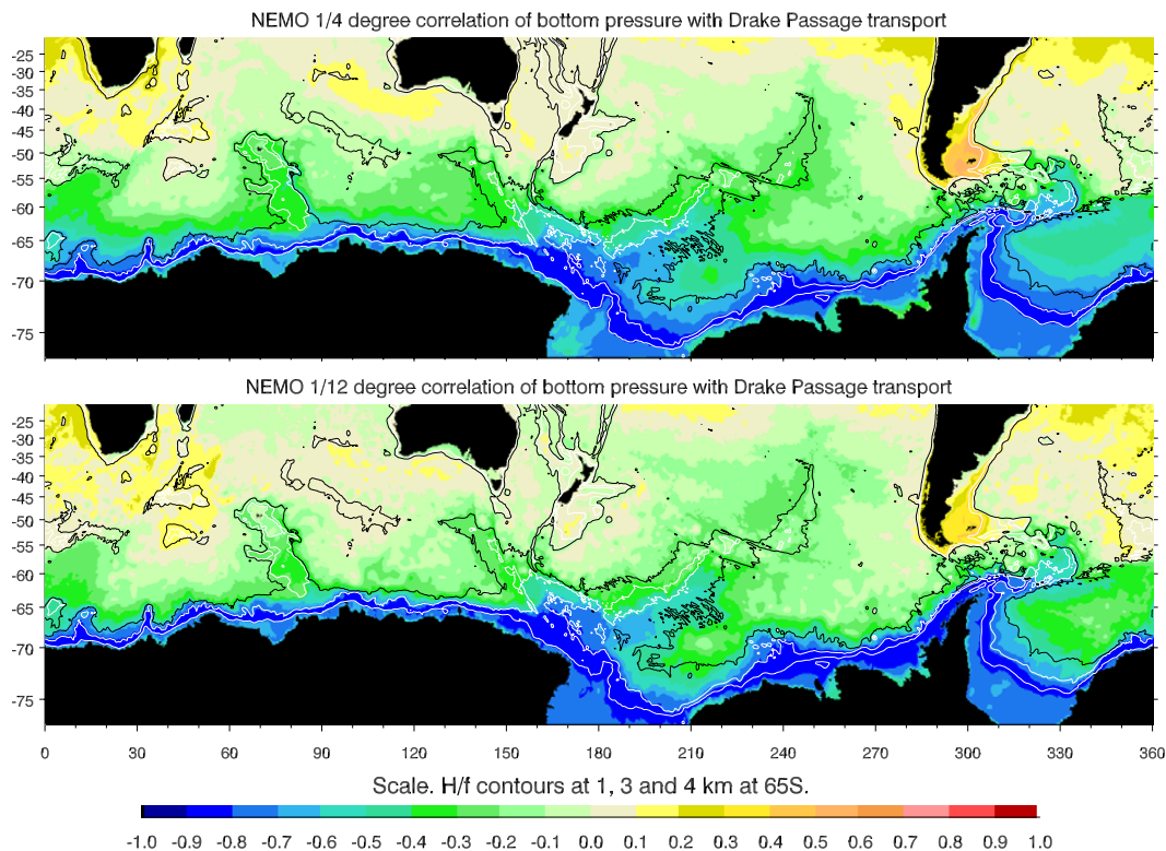
Fig. 1. Correlation between bottom pressure at each point and total flow through Drake Passage, based on (top) 50 yr of 5 day means in a 1/4^\circ resolution model, and (bottom) 20 yr of 5 day means in a 1/12^\circ resolution model. All time series have had annual, semiannual and trend removed beforehand. Contours highlight the H/f contours which, at 65^\circ S, correspond to depths of 1 km, 3 km (white) and 4 km (black).
