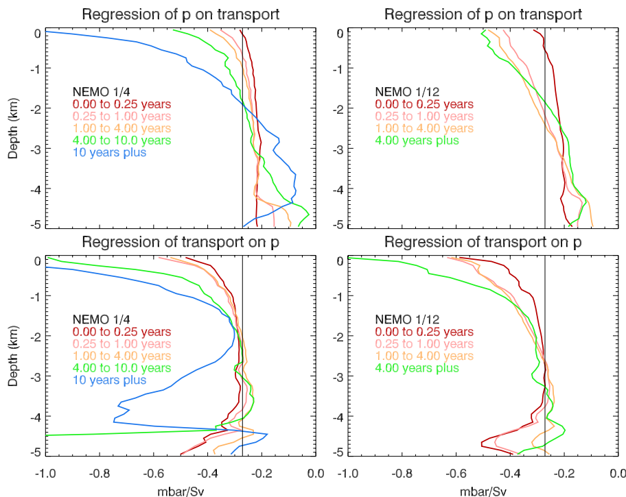
Fig. 4. Ratio of pressure p over transport \psi derived from linear regression of one on the other after applying various band pass filters given in the legends. Upper panels show a from the regression p = a\psi + b + \text{noise} , and lower panels show 1/A from the regression \psi = Ap + B + \text{noise} . When both time series contain noise, the true relationship tends to lie between these two estimates. Left hand panels are for the 1/4^\circ model and right hand panels for the 1/12^\circ model. The black line shows the kinematic estimate for the depth-average coefficient: (-3.69 \text{ Sv mbar}^{-1})^{-1} .
