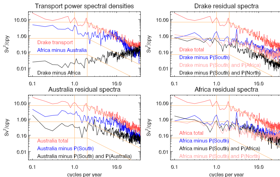
Fig. 6. Power spectra associated with variations in transport through Drake Passage, south of Africa, and south of Australia, from the 1/4^\circ model. The top left panel shows the spectrum of Drake Passage transport (red), that of the difference between Drake Passage transport and transport south of Africa (black), and that of the difference between transports south of Africa and Australia (blue). Other panels show the spectrum of transport through each section (red), of the residual after subtracting the transport accounted for by southern boundary pressure (blue) and of the residual after subtracting the transport accounted for by southern boundary pressure and the corresponding northern boundary pressure (black). Pink curves are like the black curves but use a northern boundary pressure from a different section. Orange lines are for guidance only and show representative spectra separated by factors of ten, together with the annual and semiannual frequencies.
