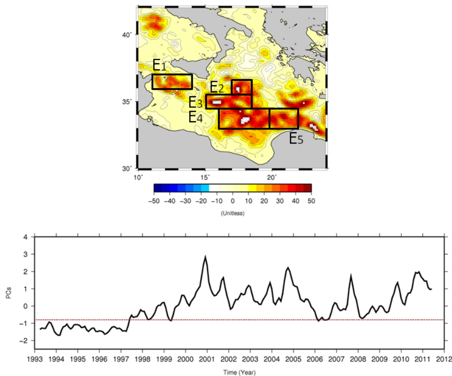
Fig. 14. Mode 1 spatial distribution of the 1993–2011 mean low-frequency EKE EOF decomposition in the Ionian region (top panel) and its associated temporal component (bottom panel). This mode explains 12.0% of the total variance. The level corresponding to -0.9 has been mentioned in order to differentiate phases of weak/strong LF-EKE intensities in relation with the absence/presence of the MIJ, respectively. Five boxes are localized on top panel: E1 = [11\text{--}14^\circ \text{ E}, 36\text{--}37^\circ \text{ N}] , E2 = [17\text{--}18.5^\circ \text{ E}, 35.5\text{--}36.5^\circ \text{ N}] , E3 = [15\text{--}18.5^\circ \text{ E}, 34.5\text{--}35.5^\circ \text{ N}] , E4 = [16\text{--}19.5^\circ \text{ E}, 33\text{--}34.5^\circ \text{ N}] and E5 = [19.5\text{--}22^\circ \text{ E}, 33\text{--}34.5^\circ \text{ N}] .
