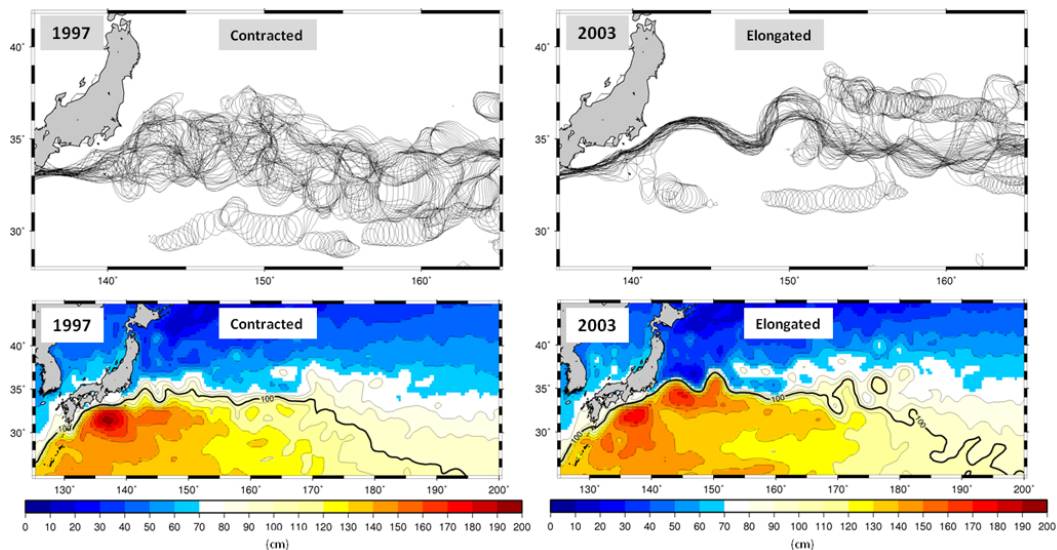
Fig. 3. Upper panels: yearly paths defined by the 100 cm contours in the weekly ADT (Absolute Dynamic Topography) fields for the 1997 contracted state (left) and the 2003 elongated state (right). Lower panels: yearly averaged ADT with a 10 cm contour interval and a thick line denoting 100 cm in the KE region during year 1997 (left) and year 2003 (right).
