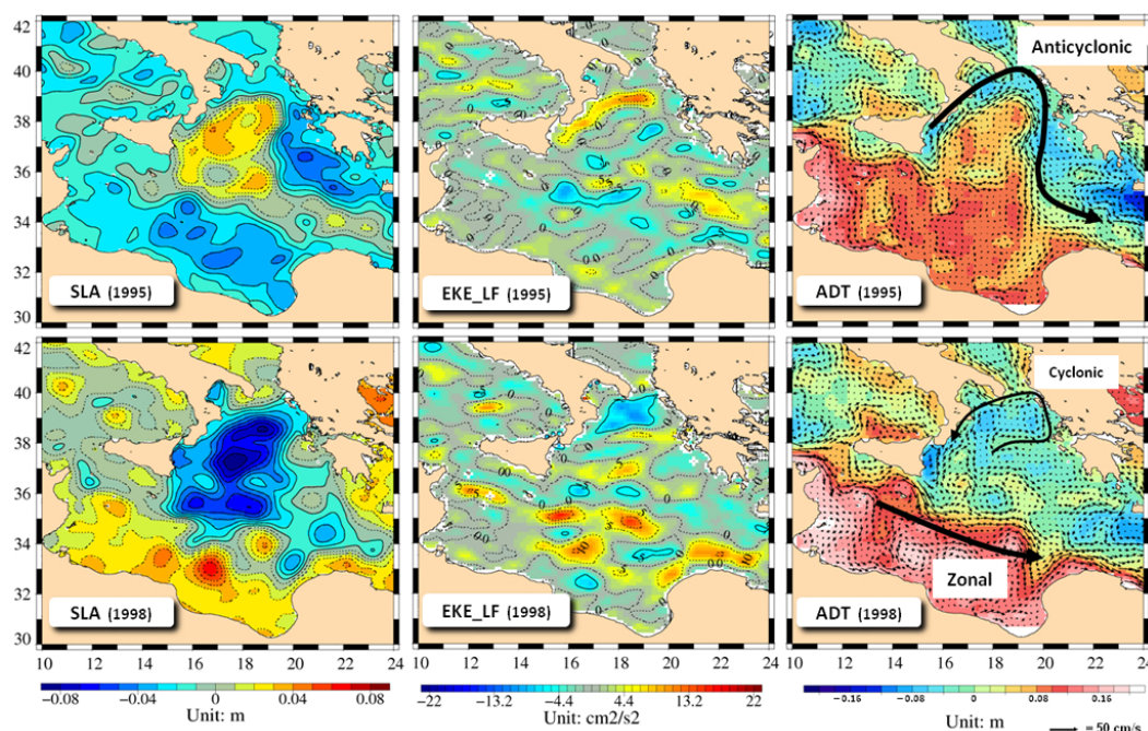
Fig. 9. Yearly averaged SLA, centered low-frequency EKE (LF-EKE) and ADT with overlaid total velocity field (left, middle and right panels, respectively) in the Ionian region during year 1995 (top panels) and year 1998 (bottom panels). Units respectively in m, \text{cm}^2 \text{s}^{-2} and m. Vector field scale: 50 \text{ cm s}^{-1} .
