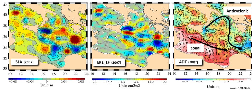
Fig. 13. Yearly averaged SLA, centered LF-EKE and ADT with overlaid total velocity field (left, middle and right panels, respectively) in the Ionian region during year 2007. Units respectively in m, \text{cm}^2 \text{s}^{-2} and m. Vector field scale: 50 \text{ cm s}^{-1} .
