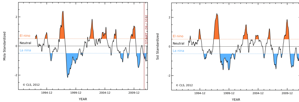
Fig. 1. Time series of SLA (left) and SST (right) divided by the respective standard deviation over the area and referenced to the 1993–2006 base period. In blue are La Ni a events, in red El Ni o.
