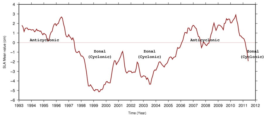
Fig. 11. Time series in the Ionian region during the period 1993–2011 of mean SLA in box S1 as defined in Figure 10 (top panel), units in cm. The red level is shown in order to differentiate the NIG phases: the “anticyclonic” phases (above red level) and the “cyclonic” phases (under red level).
