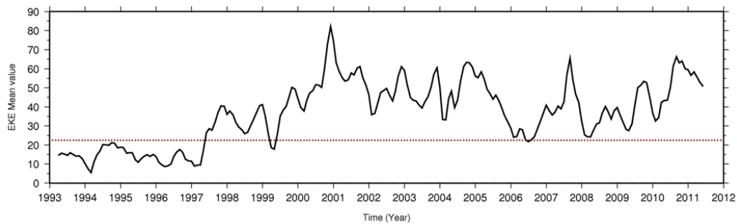
Fig. 15. Time series of mean LF-EKE in boxes E1 + E2 + E3 + E4 + E5 as defined in Fig. 14 during the period 1993–2011. Units in \text{cm}^2 \text{s}^{-2} .
