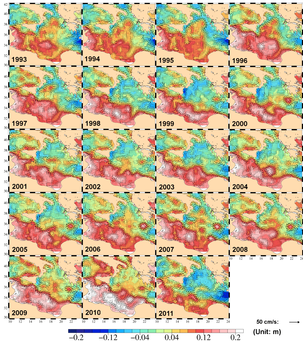
Fig. 12. Yearly averaged ADT with overlaid total velocity field in the Ionian region from year 1993 (upper left panel) to year 2011 (lower right panel). Units in m, vector field scale: 50 \text{ cm s}^{-1} .
