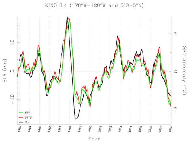
Fig. 2. Time evolution of SLA in black referenced to the 1993–2006 base period. In green the SST anomaly from Reynolds fields also referenced to the 1993–2006 base period, and in red the SST anomaly from NOAA ERSST.v2 fields referenced to the 1971–2000 base period. The latter is plotted from the ascii file obtained at ftp://ftp.cpc.ncep.noaa.gov/wd52dg/data/indices .
