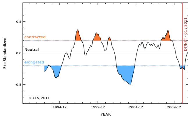
Fig. 6. Mean standardized HF-EKE defined in box B1 in the KE region during the period 1993–30 November 2011 (see Fig. 5 for B1 spatial location). Blue shaded areas correspond to elongated state periods, while orange shaded areas fit contracted state periods. The vertical red line indicates the transition between the Delayed Time (DT) and the Near Real Time (NRT) production modes of the SLA used for the HF-EKE calculation.
