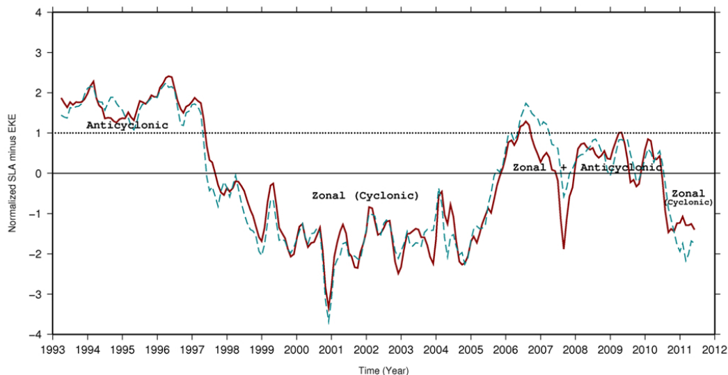
Fig. 16. Time series of mean standardized SLA minus mean standardized LF-EKE in previously defined respective boxes in the Ionian region during the period 1993–2011: average in boxes S1 and E1 + E2 + E3 + E4 + E5 (red line) and average in S1 and E2 + E3 + E4 (blue dashed line). Level 0 and level 1 have been mentioned in order to differentiate surface circulation phases.
