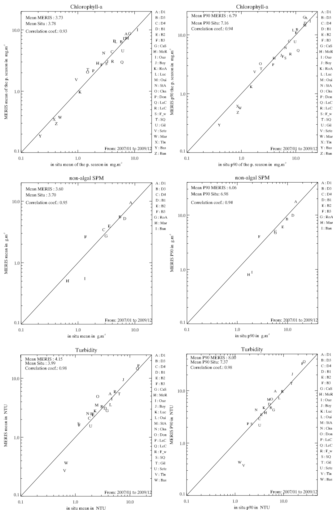
Fig. 16. Average and P90 of MERIS and in-situ Chl (productive period), non-algal SPM, and turbidity (annual).
