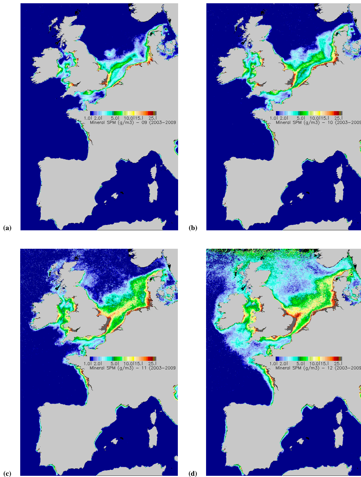
Fig. B3. Monthly non-algal SPM in September (a), October (b), November (c) and December (d).
