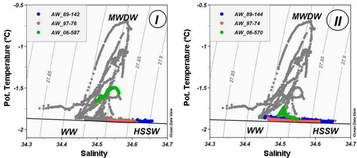
Fig. 3. Austral winter \theta/S -characteristics on the shallow (<500 m) northwestern Weddell Sea continental shelf for cruises AW_89, AW_97, and AW_06, in gray, together with selected stations from the areas I and II (Fig. 1b), sampled during austral winters of 1989 (blue), 1997 (red), and 2006 (green). The lower line represents the surface freezing temperature as a function of salinity. Isopycnals are drawn relative to surface pressure ( \sigma_0 ). MWDW = Modified Warm Deep Water, WW = Winter Water, HSSW = High Salinity Shelf Water.
