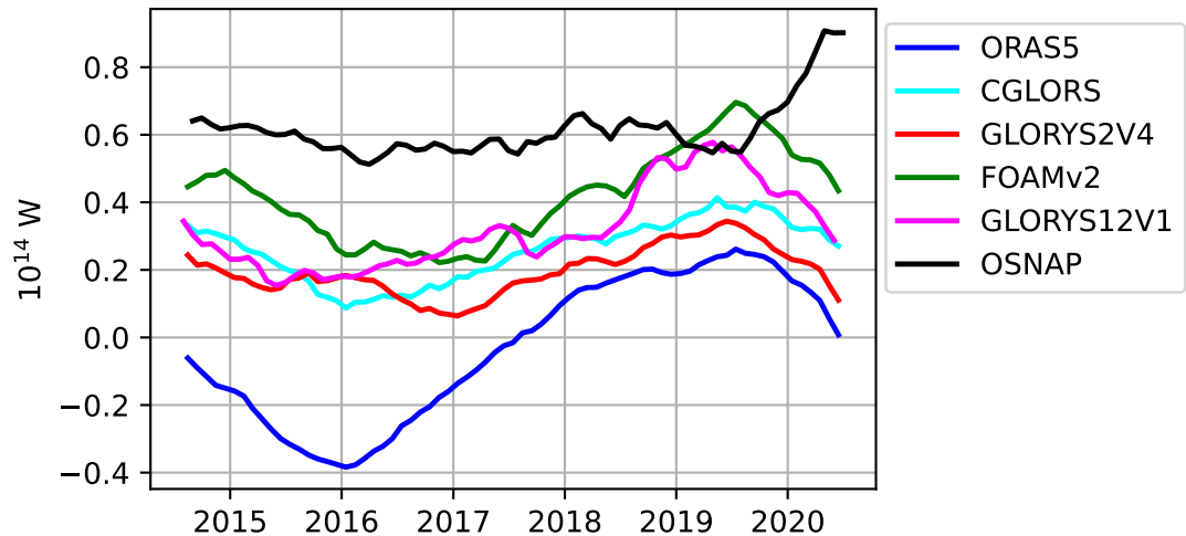
(b) Gyre heat transport
