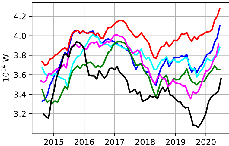
(a) Overturning heat transport
