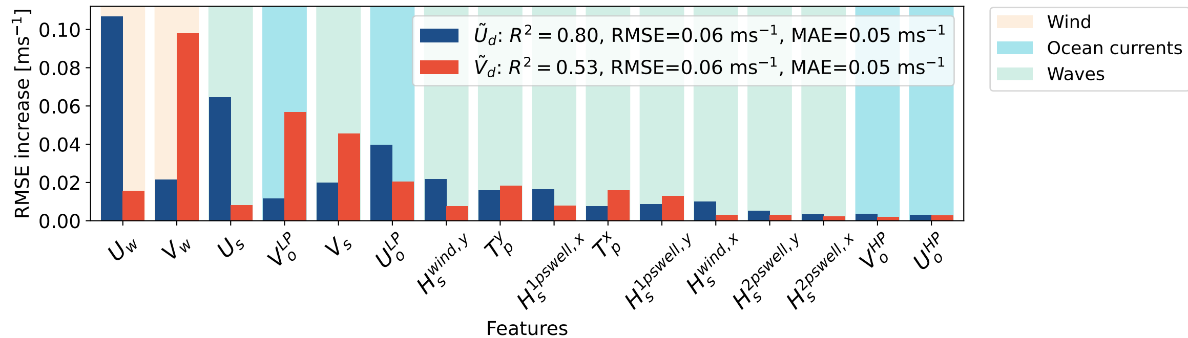
Random forest model
