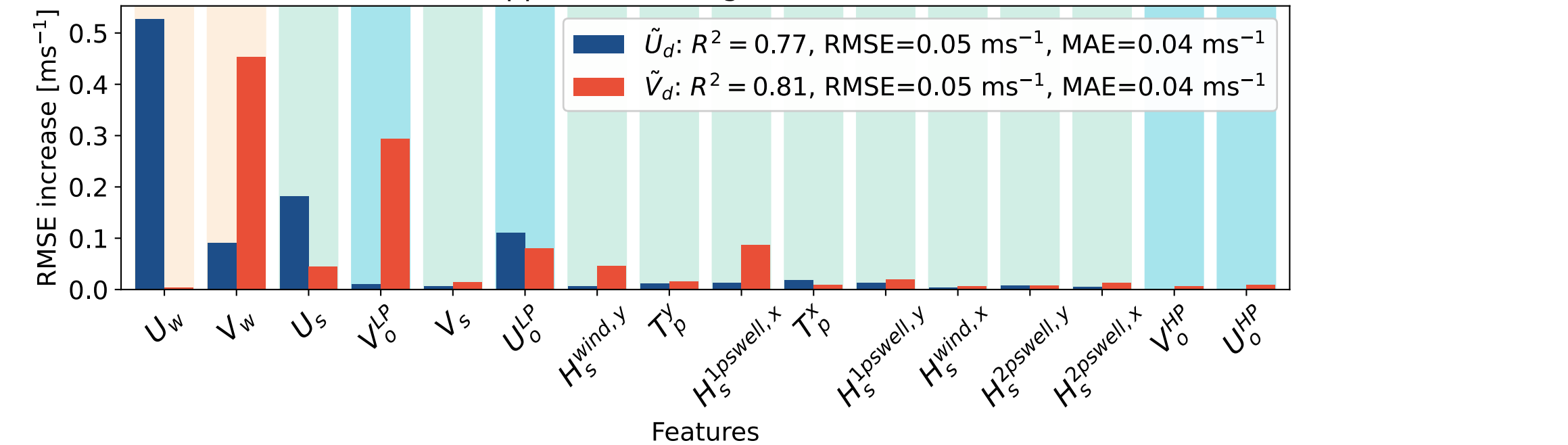
Support vector regression model
