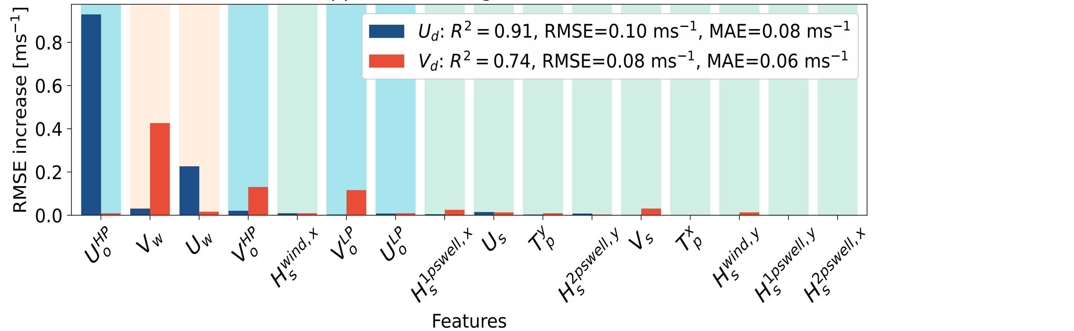
Support vector regression model
