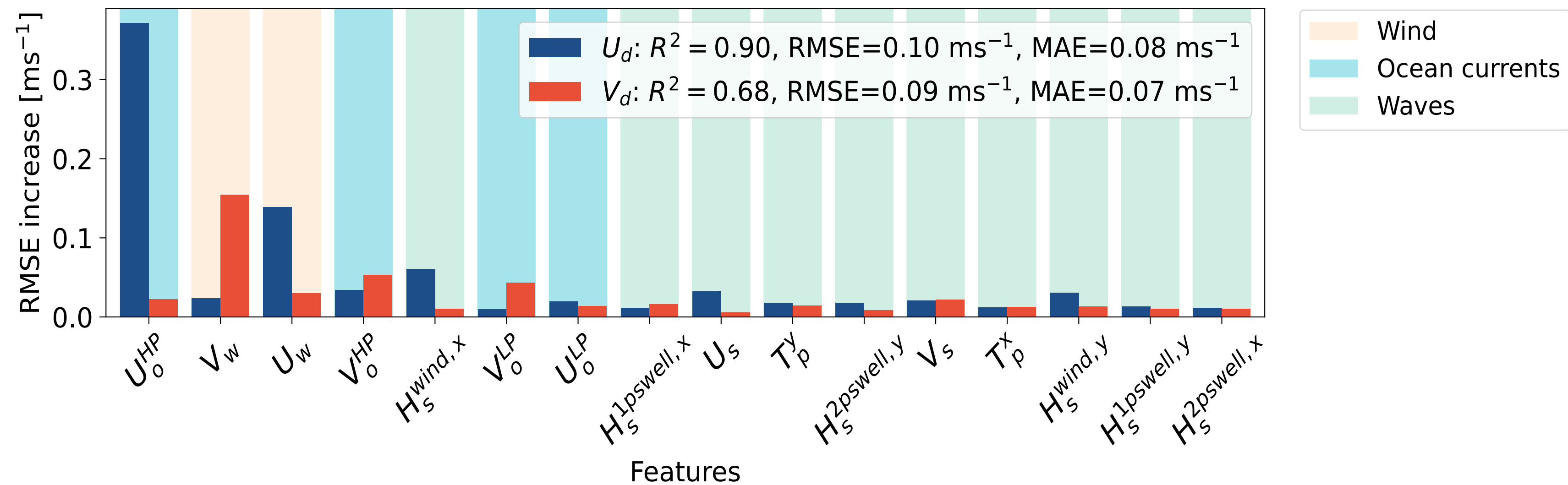
Random forest model
