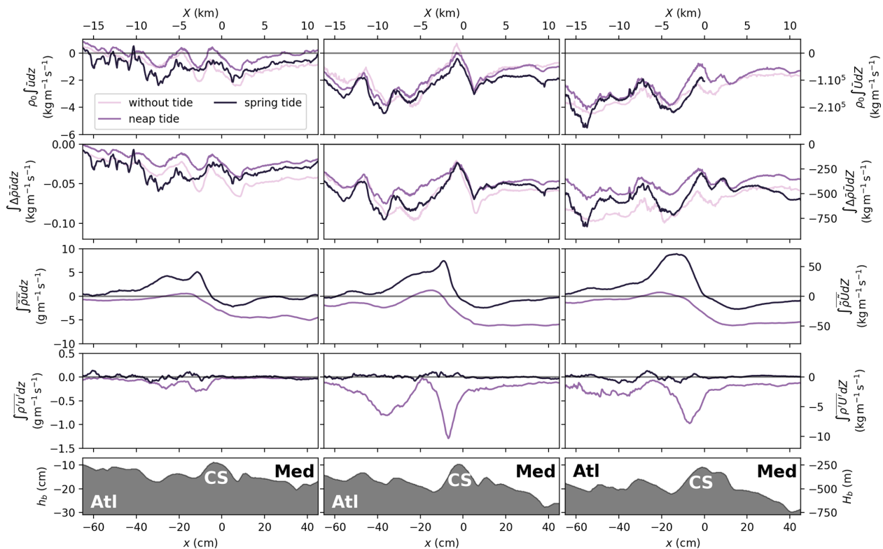
Figure 15. Mean transport contributions (per width unit) for the three transects (from left to right: northern, middle and southern transects), for tidal forcing cases (Without tide, Neap tide and Spring tide). Volume transport (first line), buoyancy transport (second line), tidal transport (third line) and turbulent transport (fourth line).
