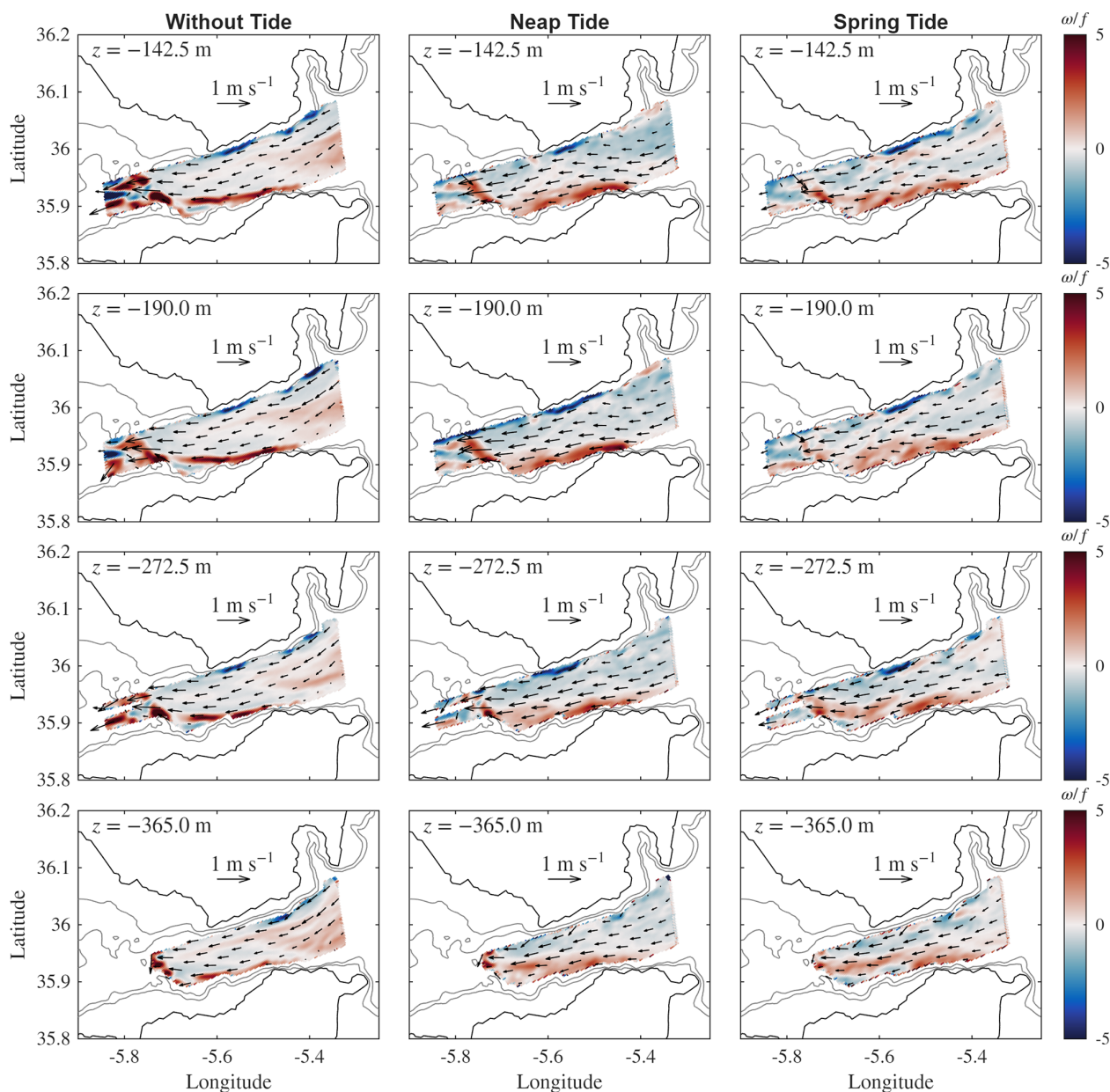
Figure 5. Averaged (over four tidal cycles) in-plane horizontal velocities with superposed relative vorticity field (colormap) in the Strait of Gibraltar at various depths for the three tidal forcings: without tide (left column), neap tide (center column), and spring tide (right column).
