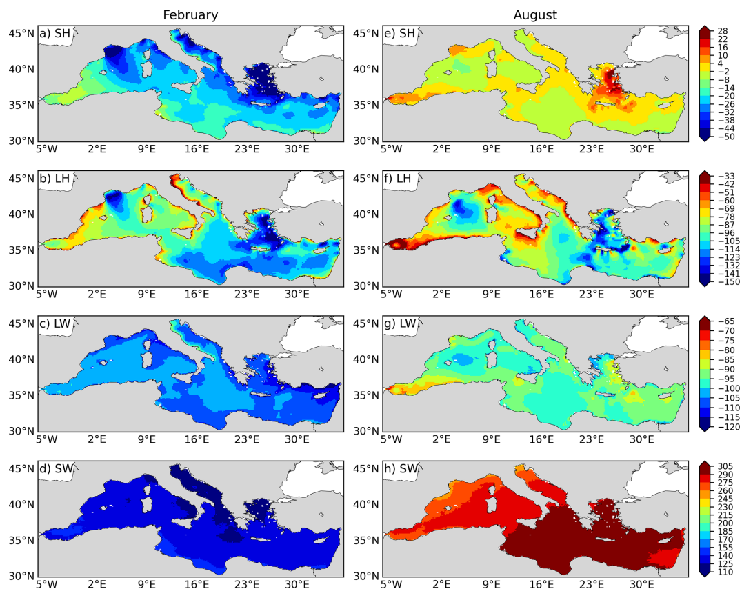
Figure 2. Seasonal variations of heat flux components: left column is the monthly average values for February and right column shows the average for August for the period 2006–2020 (ECMWF data).
