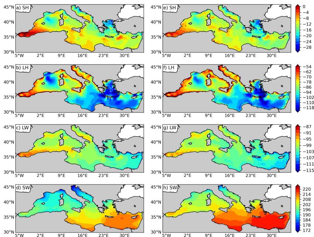
Figure 1. Annual means of heat flux components for the period of 2006–2020, computed from ECMWF (left panels) and ERA5 (right panels) daily time series. The corresponding ECMWF time series is shown in Supplement, Figs. S1 and S2.
