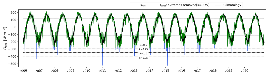
Figure 7. Time series of the basin averaged Q_{\text{net}} mean, Q_{\text{net}} extremes removed mean, and long-term yearly climatology and four lower quantile boundary line marked with dashed lines using different k values [ k = 1.25, 1, 0.75, 0.5 ].
