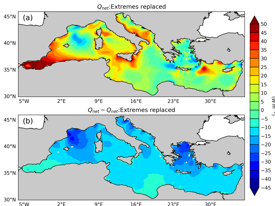
Figure 8. (a) Long term mean net heat flux after the removal of extremes ( Q_{\text{net}} : extremes replaced) using threshold of -289 \text{ W m}^{-2} ( K = 0.75 ). (b) The time mean distribution computed from the difference between Q_{\text{net}} (Fig. 3a) and “ Q_{\text{net}} : extremes replaced” time series. It shows a significant reduction of heat losses in the Gulf of Lion, Adriatic Sea and Aegean Sea regions.
