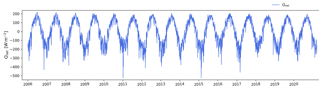
Figure 6. Basin averaged time series of the computed daily Q_{\text{net}} (units \text{W m}^{-2} ) from the ECMWF computed heat fluxes, for the period 2006–2020.
