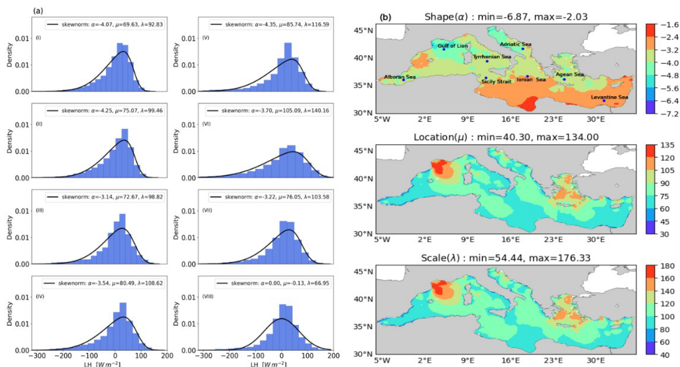
Figure 5. (a) The single grid point histograms for LH flux anomalies at the eight sampling locations for the period of 2006002020, (b) the skew-normal PDF parameter ( \alpha , \mu , \lambda ) distributions for computed LH flux anomaly for the observation period – sampling points: (I) Alboran Sea, (II) Gulf of Lion, (III) Tyrrhenian Sea, (IV) Sicily Strait, (V) Adriatic Sea, (VI) Ionian Sea, (VII) Aegean Sea, (VIII) Levantine Sea.
