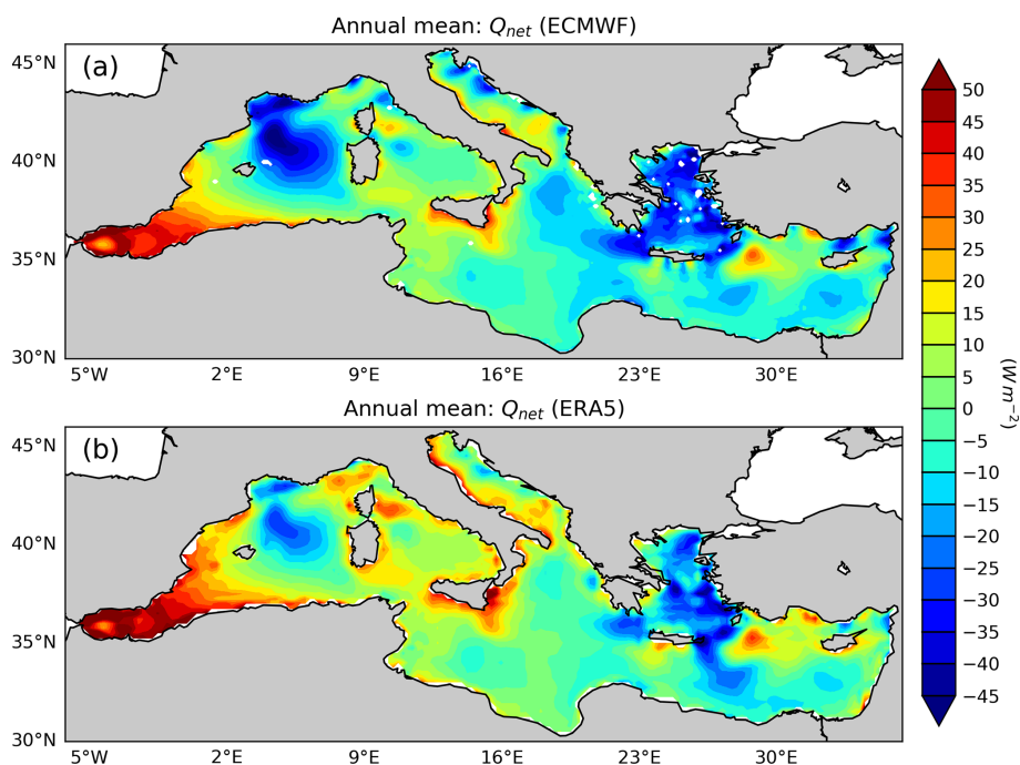
Figure 3. Comparison of the annual Q_{\text{net}} ( \text{W m}^{-2} ) mean, computed from (a) ECMWF and (b) ERA-5 input datasets.
