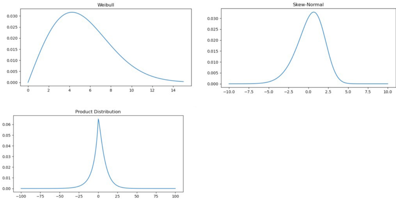
Figure A1. Histograms presenting the two original distributions, Q(v) (upper left quadrant, units wind speed) and R(DT) (upper right quadrant, units ^{\circ}\text{C} ) and the combined distribution for SH flux in units of \text{W m}^{-2} . The parameters used for the two original distributions are: k = 2.0 for the Weibull shape, \lambda = 6.0 for the Weibull scale; \alpha = -2.0 for the Skew Normal shape, \mu = 2.0 for the Skew Normal location and \omega = 2.5 for the Skew Normal scale.
