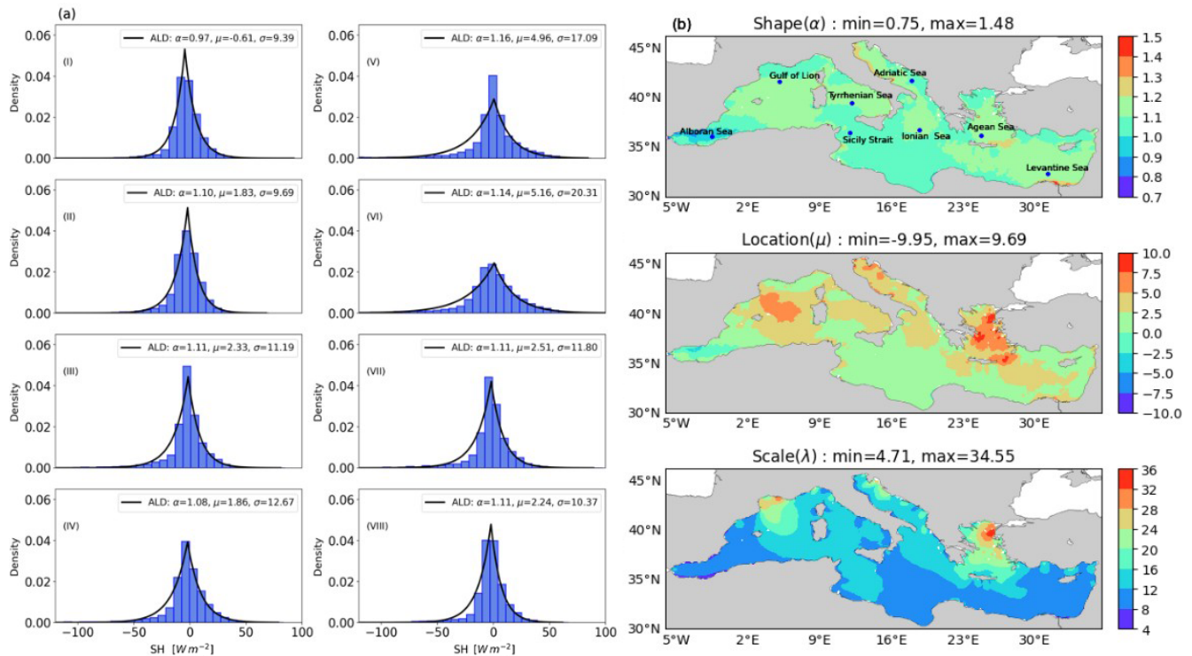
Figure 4. (a) The single grid point histograms for SH flux anomalies from the eight sampling locations for the period of 2006–2020, (b) the Asymmetric Laplace PDF parameter ( \alpha , \mu , \lambda ) distributions from computed SH flux anomaly for the observation period. Sampling points: (I) Alboran Sea, (II) Gulf of Lion, (III) Tyrrhenian Sea, (IV) Sicily Strait, (V) Adriatic Sea, (VI) Ionian Sea, (VII) Aegean Sea, (VIII) Levantine Sea.
