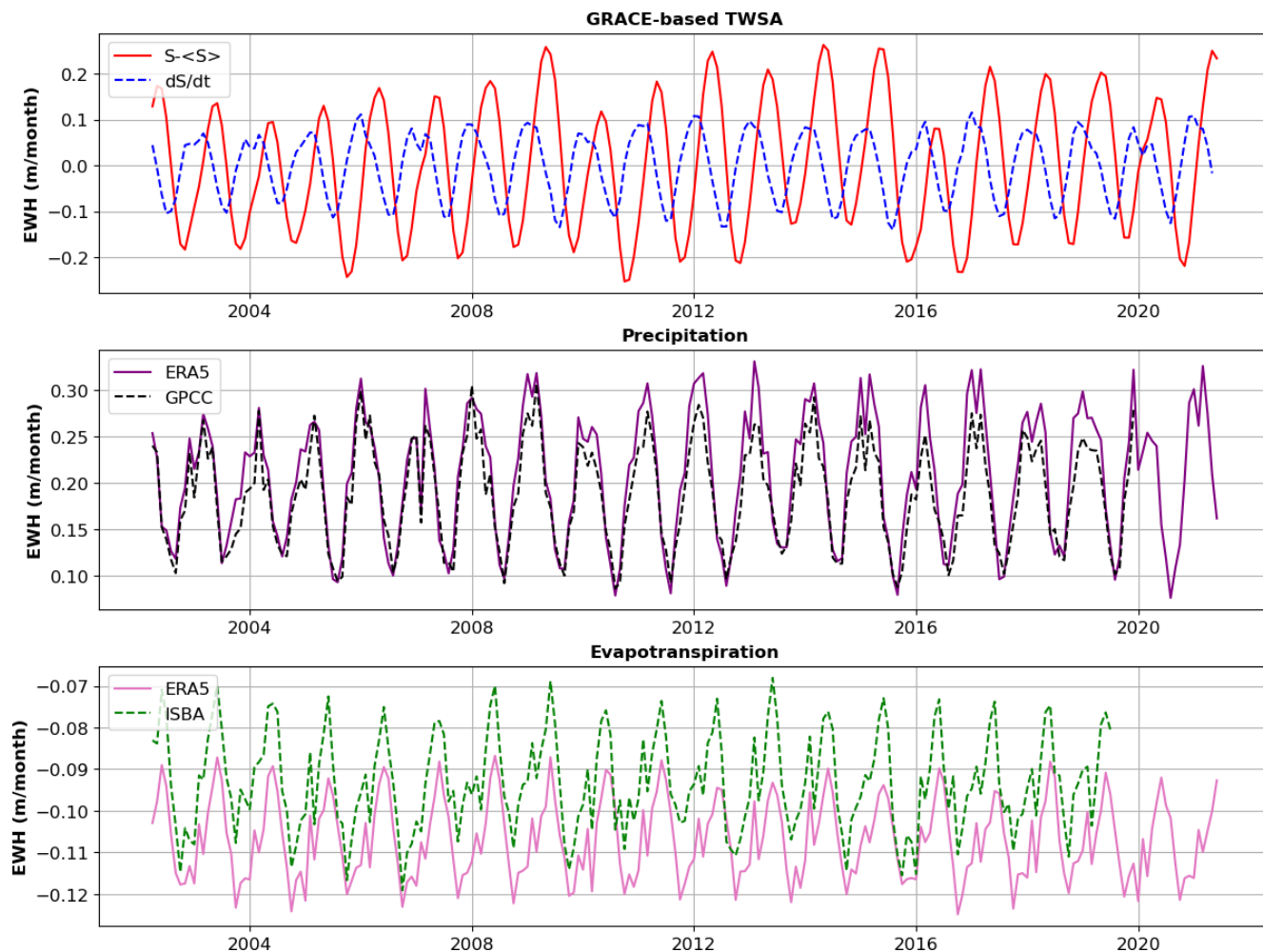
Figure A1. Decomposition of the Water Mass Balance equation for WMB1 and WMB2 at the Obidos station. The monthly time series are expressed as Equivalent Water Height in m/month over the station drainage area. From top to bottom: total water storage anomaly and first time derivative from GRACE, precipitation from ERA5 and GPCC, evapotranspiration from ERA5 and ISBA.
