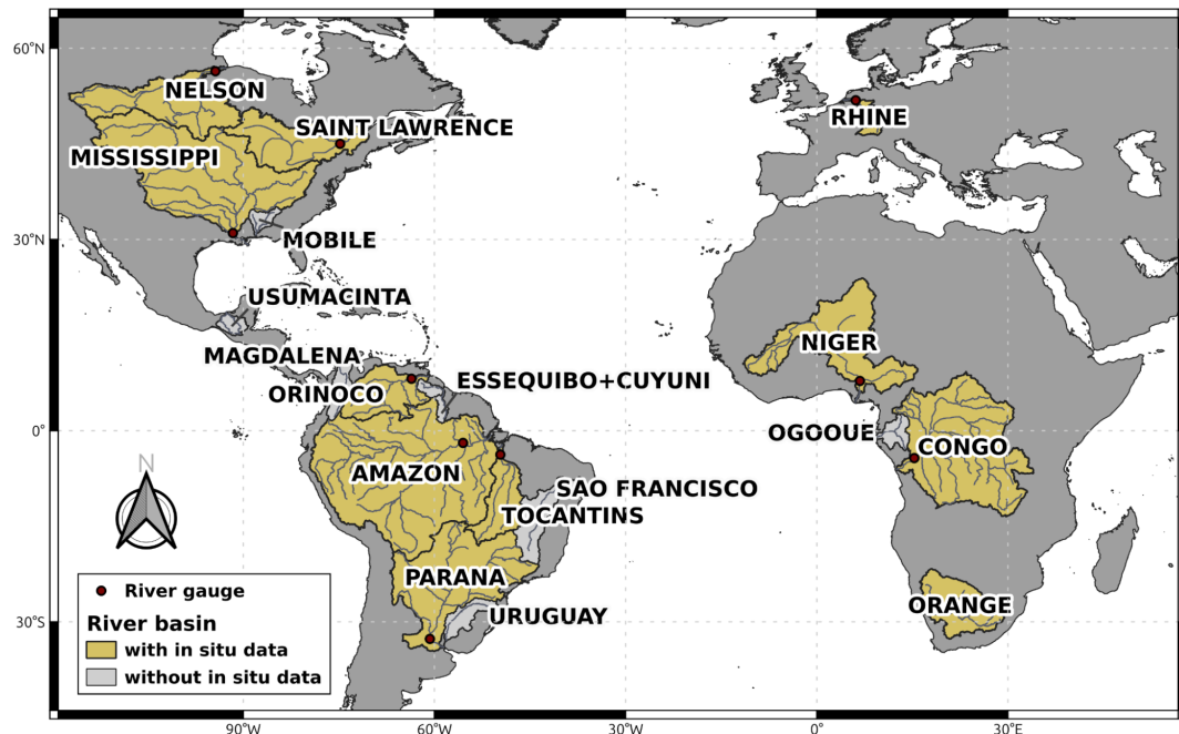
Figure 1. Map of the 18 selected rivers with their associated catchment areas. The yellow areas represent river basins where in situ data have been used for quality assessment, with the locations displayed of the river gauges shown as red dots. Light grey areas represent river basins where no in situ measurements were available over the observation period (January 2003–December 2020).
