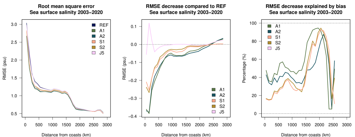
Figure 7. RMSE metrics (2003–2020) as a function of the distance to coast in the North Atlantic Ocean. From left to right: RMSE of the experiments; their RMSE decrease compared to REF; the percentage of RMSE reduction explained by bias reduction.
