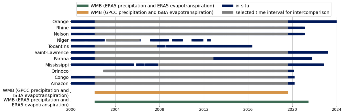
Figure 2. Availability of river discharge measurements through time. Blue lines represent periods with available in situ discharge data. Grey lines indicate the longest continuous interval with monthly in situ data, used for comparison with WMB results. The orange line shows the time span covered by the WMB approach using GPCC precipitation and ISBA evapotranspiration, bounded by the launch of the GRACE satellites (start) and the availability of the ISBA-CTRIP model (end). The green line shows the WMB time span based on ERA5 precipitation and evapotranspiration.
