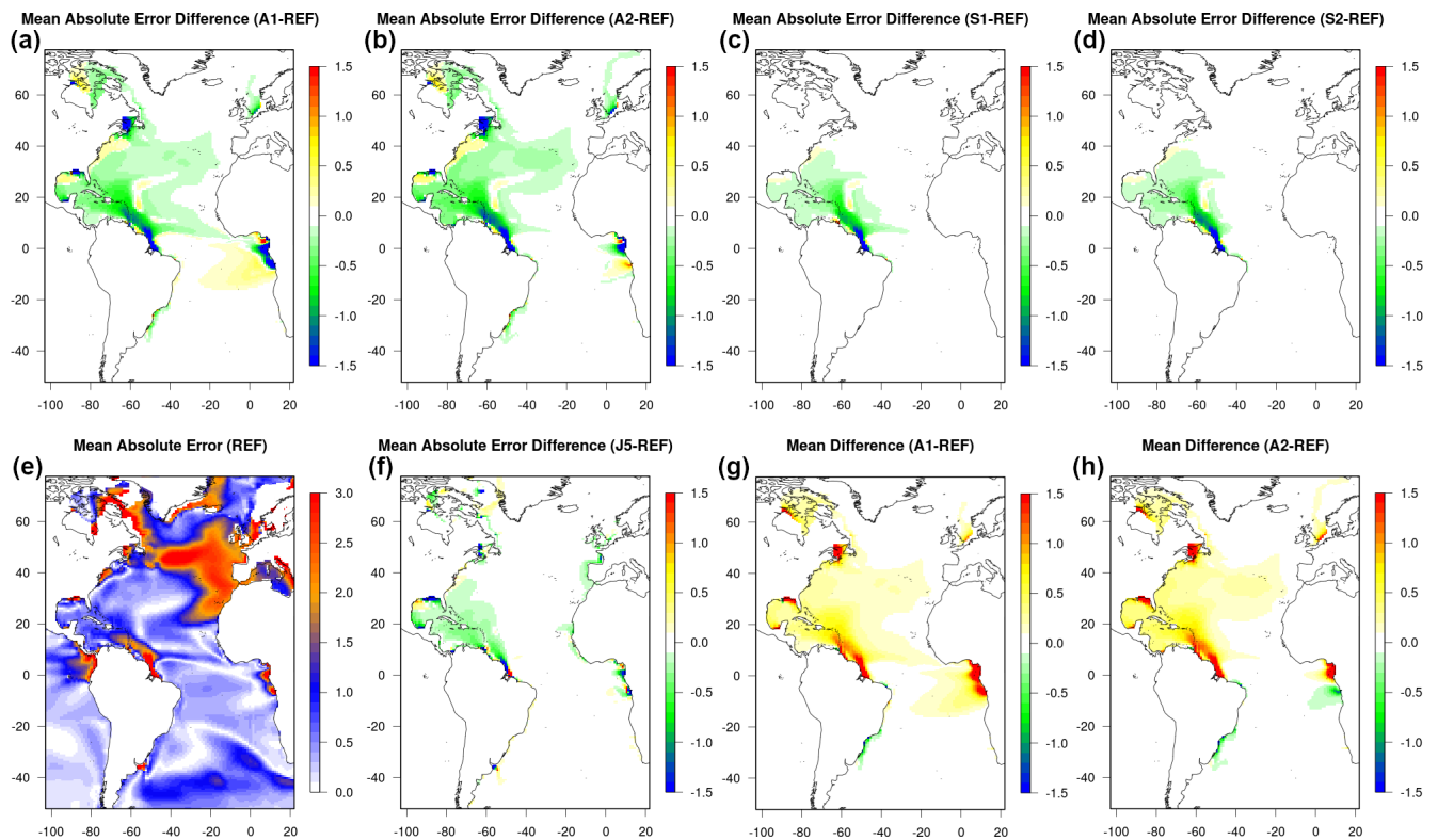
Figure 6. Difference in the mean absolute error (MAE) of sea surface salinity between each experiment (A1, A2, S1, S2, J5) and REF, i.e. MAE(\text{experiment vs. EN4}) - MAE(\text{REF vs. EN4}) , computed against EN4 objective analyses of salinity (Good et al., 2013). Negative values therefore indicate an error reduction with respect to REF. Panel e: MAE from the REF experiment; Panel g, h: time-mean difference of SSS between A1 or A2 and REF. The period is 2003–2020. Units are psu.
