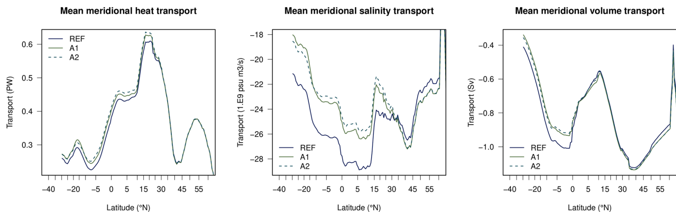
Figure 10. Meridional volume, heat, and salinity transports across the Atlantic Ocean, for the A1, A2, and REF experiments over the 2003–2020 period.
