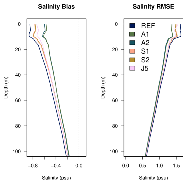
Figure 8. Salinity bias and RMSE profiles for the experiments presented in the text, calculated against EN4 objective analyses of salinity (Good et al., 2013), for the period 2003–2020. Only grid-points closer than 500 km to the shoreline are used.
