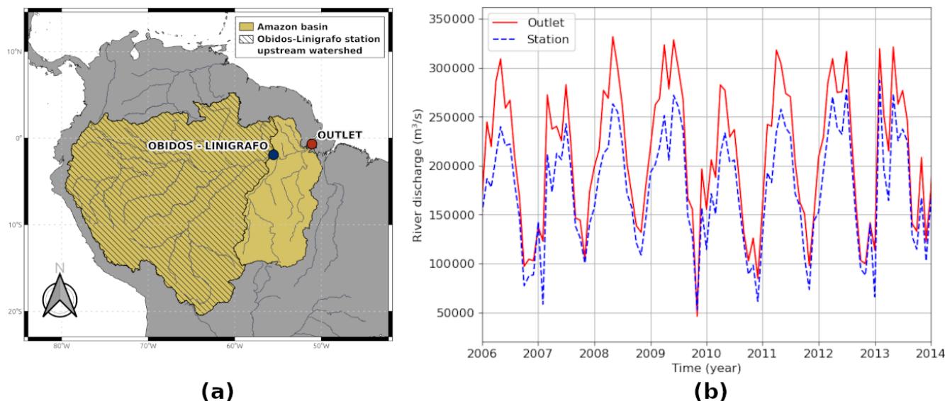
Figure 4. Comparison between discharge values at the Obidos-Linografo station located furthest downstream of the Amazon and at the river outlet. Figure (a) shows the location of the Obidos-Linografo station as a blue dot and the river outlet as a red dot. The complete river basin is represented in yellow, and the hatched area corresponds to the Obidos-Linografo station upstream watershed. Figure (b) displays estimated discharge values using the WMB approach with ERA5 precipitation and evapotranspiration data. The red curve represents the estimation at the outlet location (using the whole river basin), and the blue curve represents the estimation at the Obidos-Linografo station (using the station's upstream watershed).
