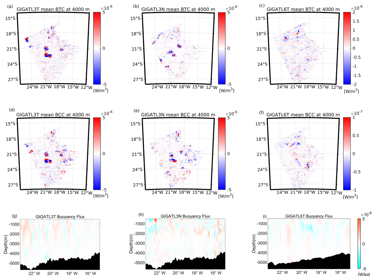
Figure A4. Monthly mean of BTC (a–c) and BCC (d–f) at the depth of 4000 m in GIGATL3T, GIGATL3N and GIGATL6T. Profiles (g–i) of 5 d averaged buoyancy flux along 21°S.
