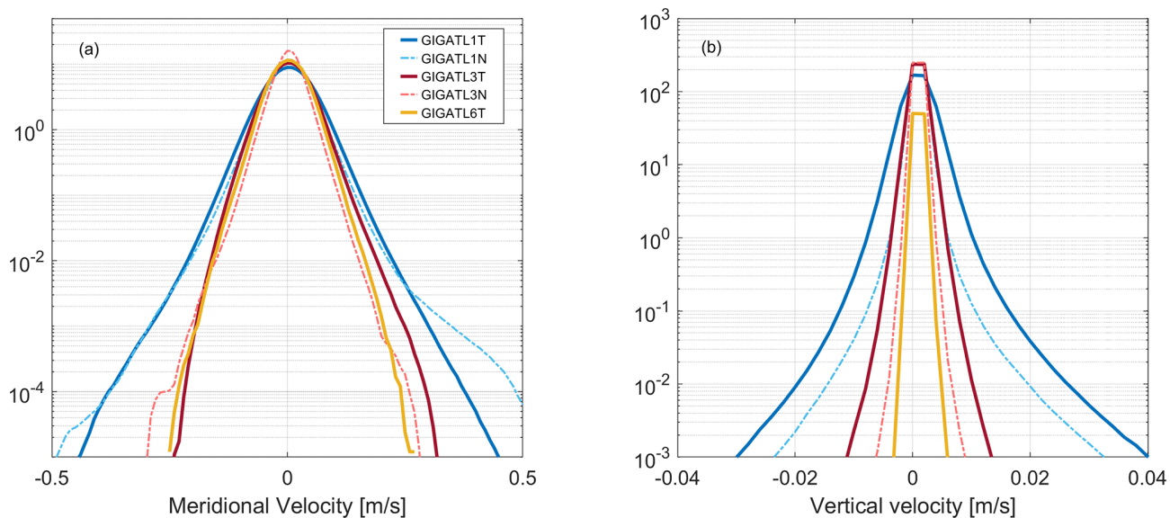
Figure A2. The probability density functions of (a) meridional velocity in \text{m s}^{-1} , (b) vertical velocity at the top of the BBL in \text{m s}^{-1} .
