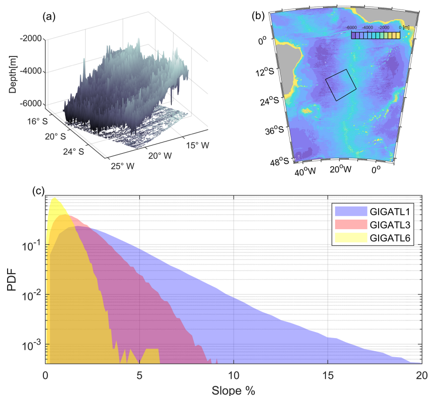
Figure 1. Study region and context in the abyssal Brazil Basin. (a) The bathymetry of the model study region. (b) Map of the Brazil Basin showing the model study region (black box). (c) Probability density function of slope distribution of GIGATL1 (1 km resolution), GIGATL3 (3 km resolution) and GIGATL6 (6 km resolution) simulations in the black box.
