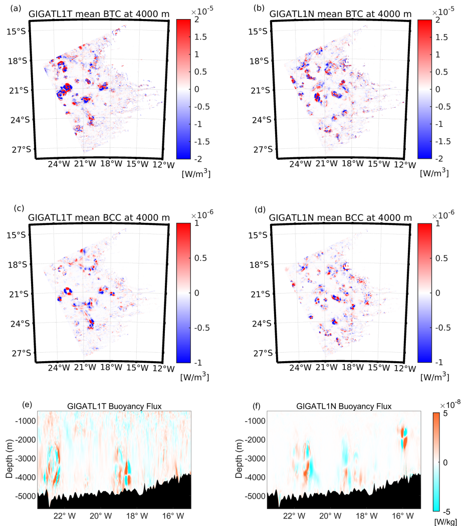
Figure 3. Monthly mean of BTC ( \text{W m}^{-3} ) (a–b) and BCC ( \text{W m}^{-3} ) (c–d) at the depth of 4000 m in GIGATL1T and GIGATL1N. Profiles of 5 d averaged buoyancy flux along 21^\circ\text{S} in (e) GIGATL1T and (f) GIGATL1N.
