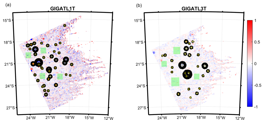
Figure A1. Particle release locations in the GIGATL1T (a) and GIGATL3T (b) simulations at 4000 m depth. Relative vorticity is shown in color in the background. Yellow crosses mark the centers of detected eddies. Black circular regions indicate particle releases surrounding coherent eddies, while green boxes indicate releases in background-flow regions without detected eddies.
