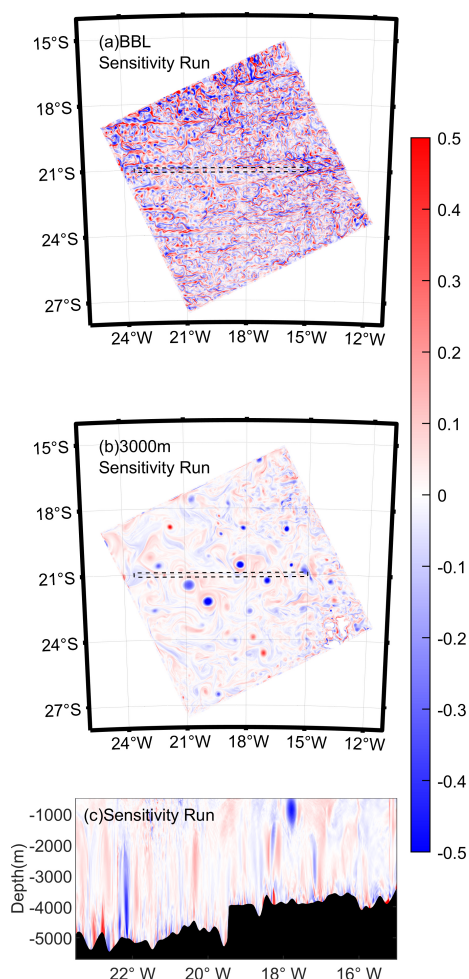
Figure A6. A 5 d averaged vorticity field of the sensitivity run at 3000 m and at the top of BBL; vorticity profiles along 21° S (dashed square in a and b ).
