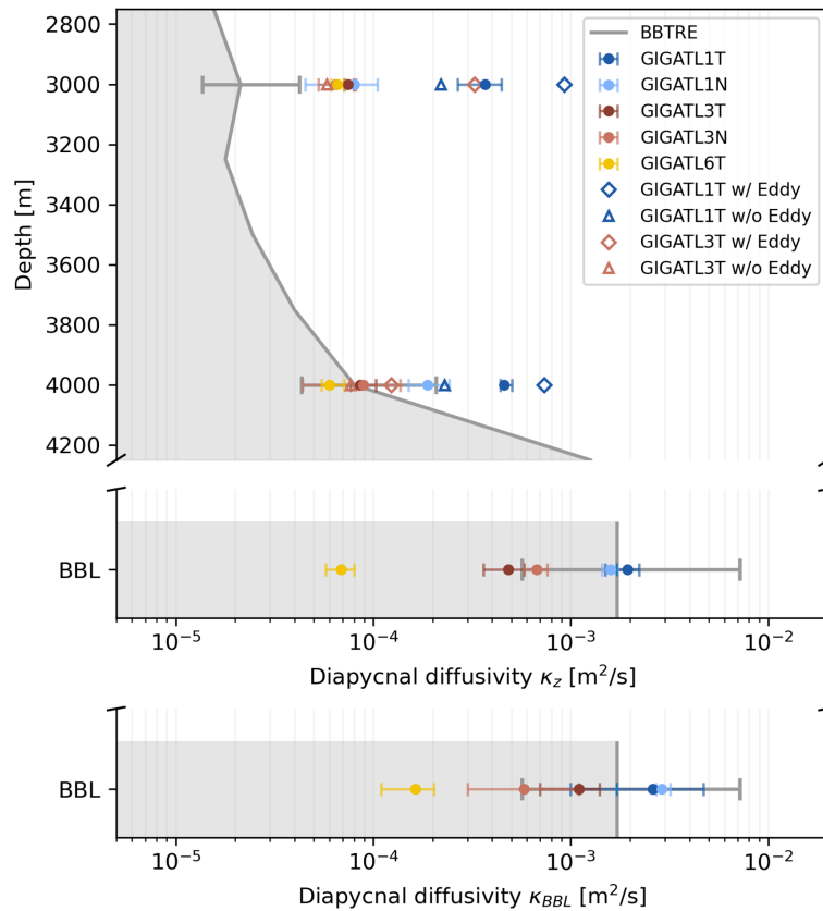
Figure 4. Diffusivities in the abyssal Brazil Basin in the observations and the five GIGATL simulations: vertical diapycnal diffusivity K_z , and BBL diffusivity K_{BBL} . Gray shading and lines represent BBTRE observations. Horizontal bars indicate ranges (max-min) across sampled patches and the depths at which tracer particles were released in the CROCO simulations. Values from releases around eddies or in the background flow at 3000 and 4000 m depth are also indicated.
