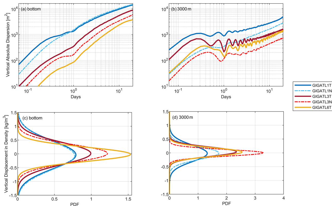
Figure A5. Vertical absolute dispersion ( \text{m}^2 ) (a, b); Vertical diapycnal displacement of tracer particles at Day 20 after release (c, d).
