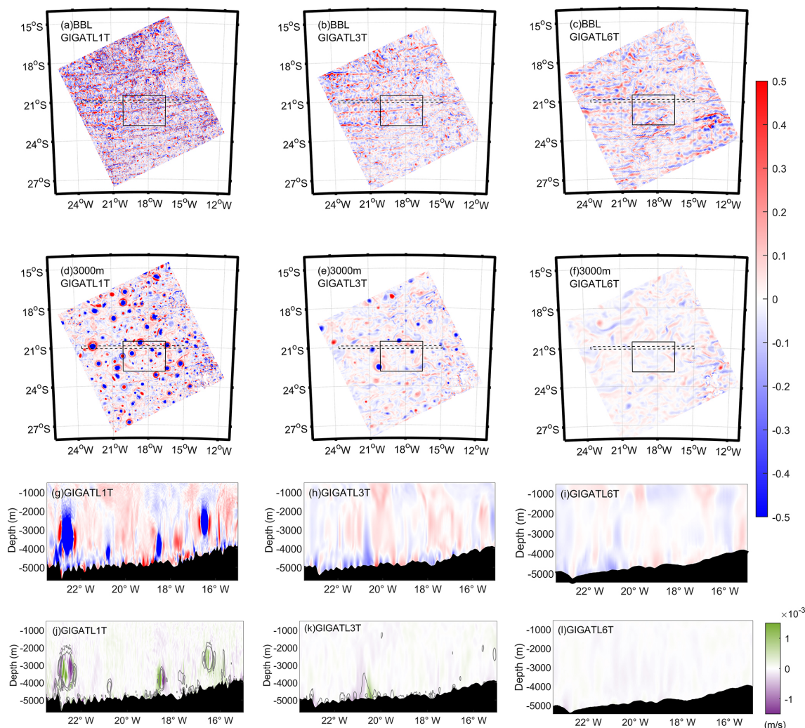
Figure 2. 5 d averaged vorticity field in GIGATL1T (a,d), GIGATL3T (b,e) and GIGATL6T (c,f) at the top of the BBL (a–c) and at 3000 m (d–f); vorticity profiles along 21° S (dash square in a–f) in the GIGATL1T (g), GIGATL3T (h) and GIGATL6T (i) simulations and vertical velocity across the same transect (j–l). In (j, k), contour lines represent vertical vorticity normalized by the Coriolis parameter ( \zeta/f ), with specified levels at -0.5 , -0.25 , 0.25 , and 0.5 in the GIGATL1T case (j), and at -0.25 , -0.125 , 0.125 , and 0.25 in the GIGATL3T simulation (k).
