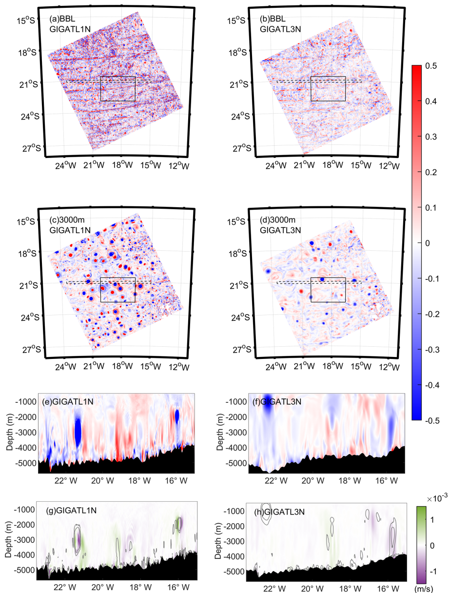
Figure A3. A 5 d averaged vorticity field of GIGATL1N ( a, c ), GIGATL3N ( b, d ) at 3000 m and at the top of BBL; vorticity profiles along 21° S (dash square in a–d ) in the GIGATL1N ( e ) and GIGATL3N ( f ) simulations and corresponding vertical velocity slices ( g, h ). Contour lines represent vertical vorticity normalized by the Coriolis parameter ( \zeta/f ), with specified levels at -0.5 , -0.25 , 0.25 , and 0.5 in the GIGATL1N cases ( g ), and at -0.25 , -0.125 , 0.125 , and 0.25 in the GIGATL3N simulations ( h ).
