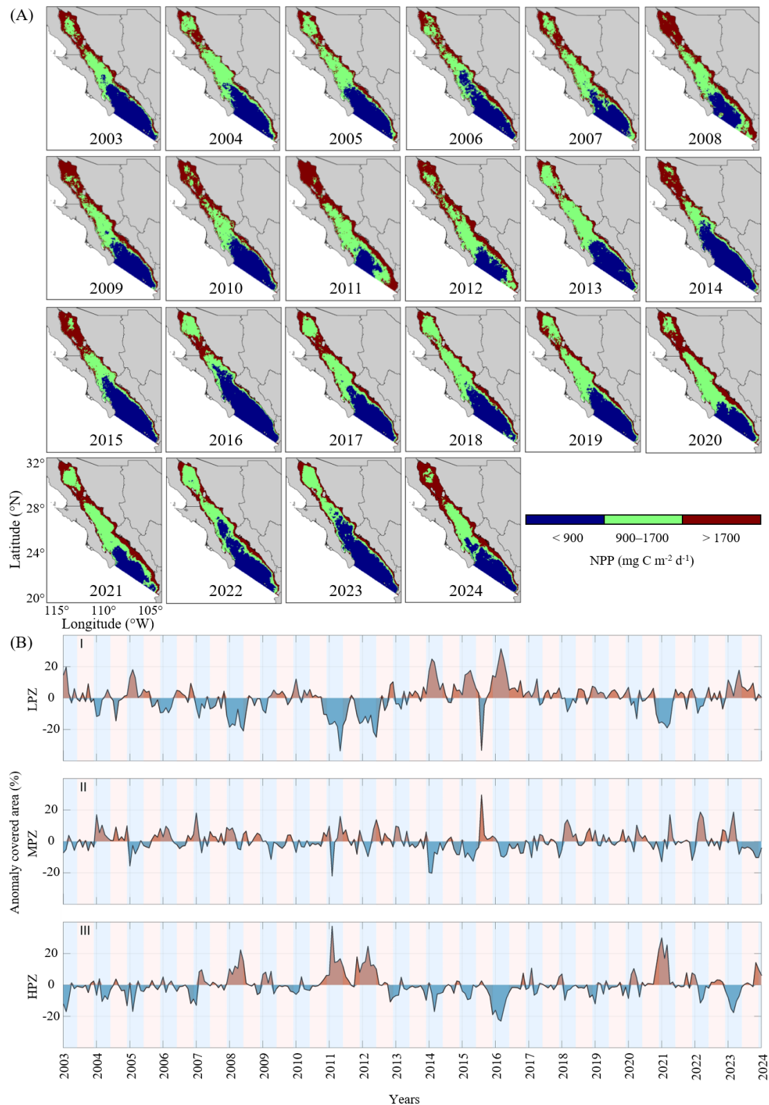
Figure 5. (A) NPP annual maps showing low-productivity (LPZ), mid productivity (MPZ), and high productivity (HPZ) variability during 2003–2024; (B) anomalies in class coverage (%) through time for (A) low (LPZ), (B) mid (MPZ), and (C) high (HPZ). Cold (blue) represents a reduction in cover, and warm (red) represents an increase in cover relative to the historical average distribution.
