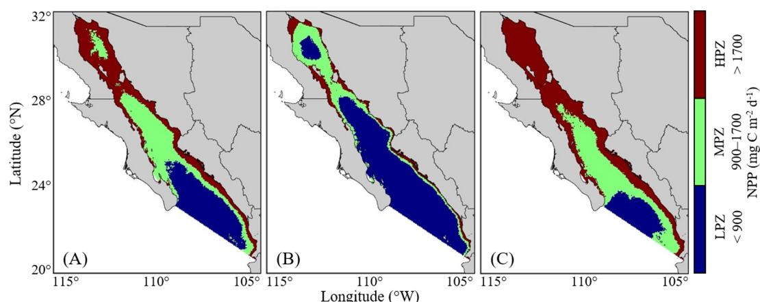
Figure 3. Regionalisation of net primary productivity (NPP) based on (A) the k-means ++ clustering of the January 2003–December 2024 global climatology, (B) warm seasonal (June–November), and (C) cold seasonal (December–May). NPP classes: low-productivity (LPZ < 900 mg C m -2 d -1 ), mid-productivity (MPZ 900–1700 mg C m -2 d -1 ), and high-productivity (HPZ > 1700 mg C m -2 d -1 ).
