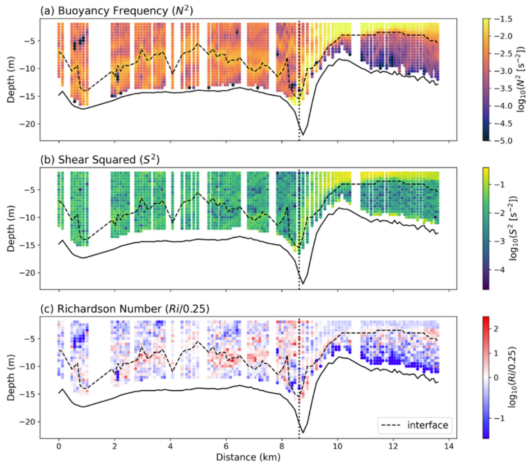
Figure 9. Spatial distributions of (a) buoyancy frequency ( N^2 , \text{s}^{-2} ), (b) squared vertical shear ( S^2 , \text{s}^{-2} ), and (c) gradient Richardson number normalized by its critical value ( Ri/0.25 ). The dashed line indicates the interface position between layers. The vertical dotted line marks the position of the mouth (inlet). Distance (km) is measured from the first upstream profile within the channel.
