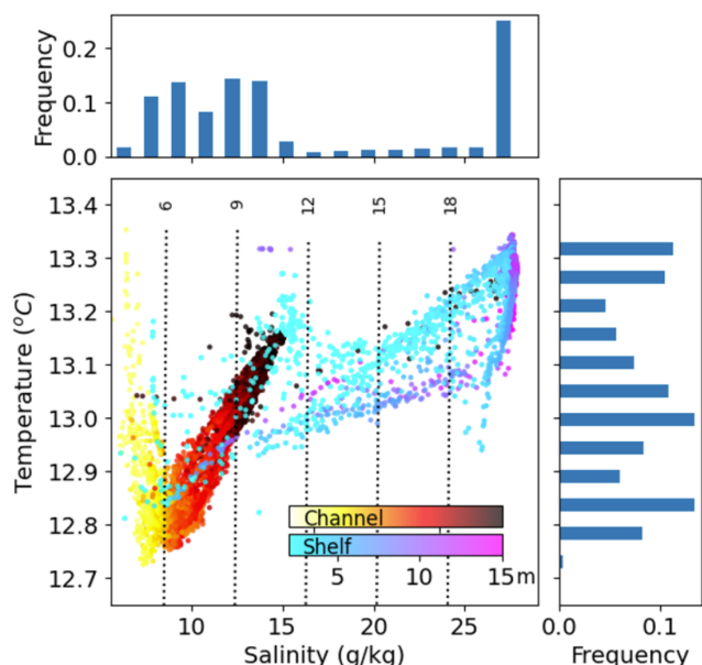
Figure 5. Temperature–Salinity ( T – S ) diagram and frequency histograms of salinity (top) and temperature (right) for the Drift segment. The central panel shows temperature ( ^{\circ}\text{C} ) versus salinity ( \text{g kg}^{-1} ), with dotted vertical lines indicating density anomaly ( \sigma_t ) values. The colour bar distinguishes data from the Channel (warm tones) and the Shelf (cold tones), with shading representing the sampling depth (m).
