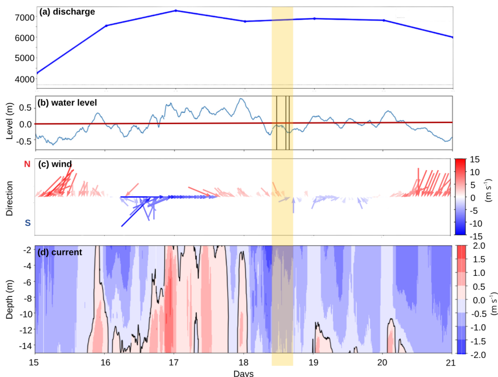
Figure 2. Environmental conditions between 15 and 21 July 2022, with the vertical yellow bar representing the survey period. (a) Gauged river discharge of the Patos Lagoon ( \text{m}^3 \text{s}^{-1} ). (b) Water level (m) measured in the channel, where the three vertical lines indicate the start moment of each section: Drift, Jetties, and Transect. (c) Vector plot of wind velocity ( \text{m s}^{-1} ) in meteorological notation, where blue represents southerly winds (blowing towards the north) and red represents northerly winds (blowing towards the south). (d) Hovmöller diagram of the along-channel current velocity ( \text{m s}^{-1} ) measured in the channel, where red indicates inflow (flood) and blue indicates outflow (ebb).
