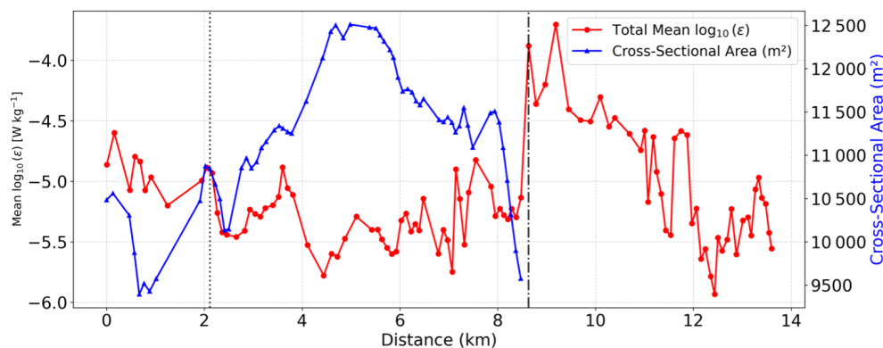
Figure 13. Longitudinal distribution of depth-average TKE dissipation rate ( \log_{10}(\epsilon) , \text{W kg}^{-1} ) and channel cross-sectional area ( \text{m}^2 ) as a function of distance. The red line (left y -axis) represents the average dissipation rate, while the blue line (right y -axis) indicates the cross-sectional area along the Drift segment. The dotted vertical line marks the initial channel widening, and the dash-dotted vertical line indicates the maximum constriction point (mouth) at the estuary–shelf interface.
