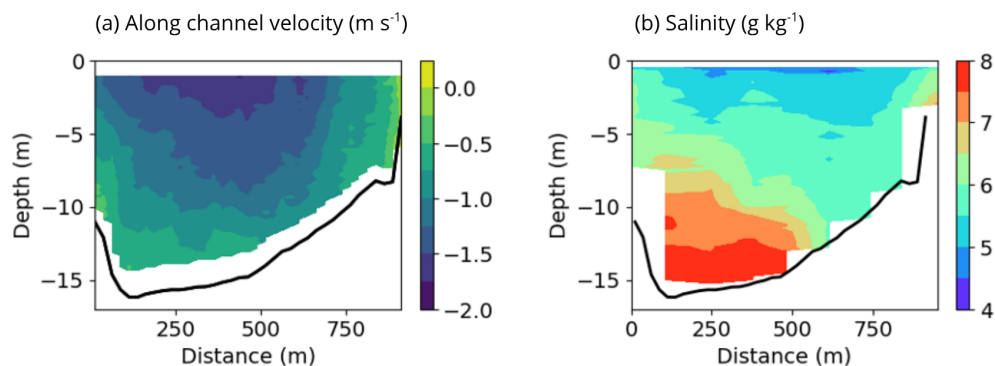
Figure 3. Cross-sectional distribution of (a) along channel current velocity ( \text{m s}^{-1} ; negative values indicate outflow) and (b) salinity ( \text{g kg}^{-1} ) at the Transect segment, characterizing the lagoon outflow during the survey.
