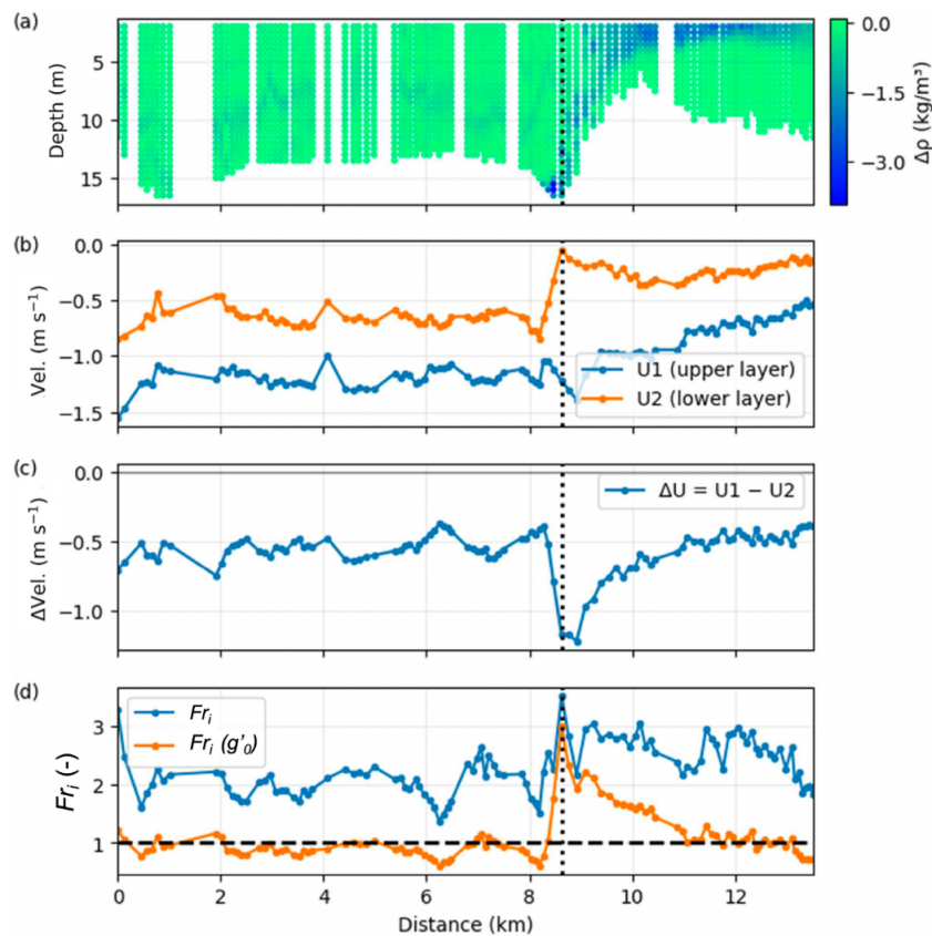
Figure 14. (a) Vertical density gradient ( \Delta\rho , \text{kg m}^{-3} ); (b) upper- and lower-layer horizontal velocities ( U , \text{m s}^{-1} ); (c) layer velocity difference ( \Delta U , \text{m s}^{-1} ); and (d) the Internal Froude Number calculated based on g' calculated for every vertical profile ( Fr_i ), and alternatively using a reference g'_0 . The dashed horizontal line in panel (d) indicates the critical threshold ( Fr_i = 1 ). The vertical dotted line marks the point of maximum constriction at the estuary–shelf interface.
