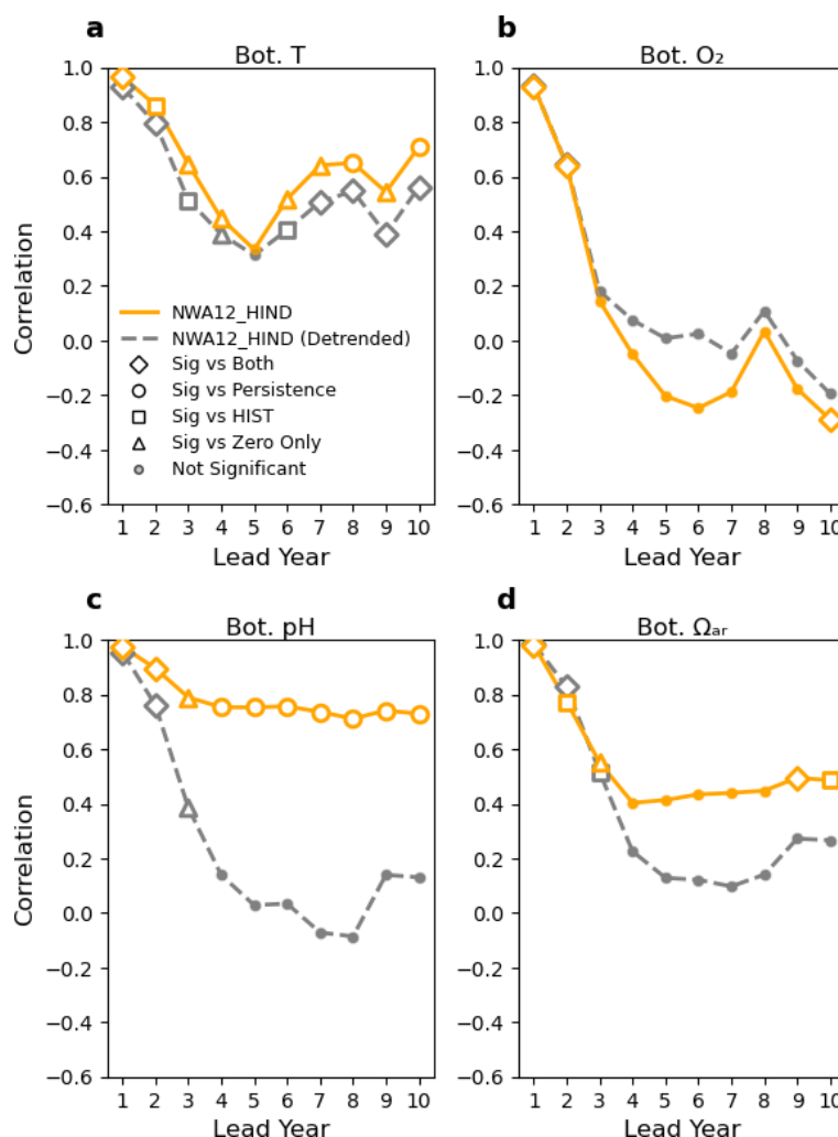
Figure 5. Decadal prediction skill. Anomaly correlation coefficient of the annual mean anomalies from the initialized regional downscaled model (NWA12_HIND) predictions. The symbols indicate statistically significant differences relative to alternative models of no correlation, persistence, and the uninitialized (historical) simulation (see Sect. 2). The correlation is calculated against the regional downscaled simulation (NWA12_EN4_NUDG)-derived annual mean anomalies (ensemble mean) for (a) bottom temperature, (b) bottom O 2 , (c) bottom pH and (d) bottom Ω ar over the GOM_EPU. The prediction and persistence skills are calculated for the common 1965–2024 period. The grey dashed lines show skill for the linearly detrended annual mean anomalies.
