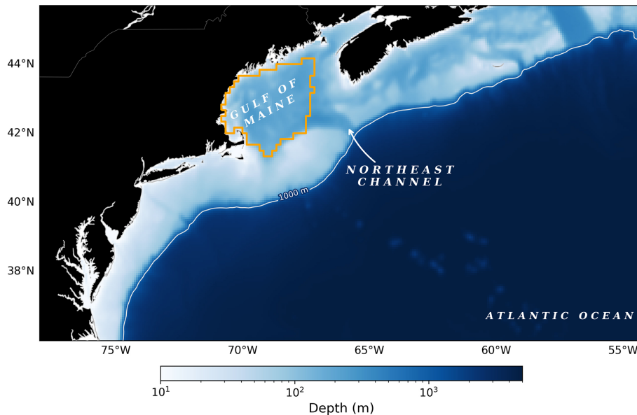
Figure 1. The study region and its characteristics. The locations of the Gulf of Maine Ecological Production Unit (GOM_EPU) and the Northeast Channel along the Northeast US continental shelf are shown along with the model bathymetry and the 1000 m isobath (white line).
