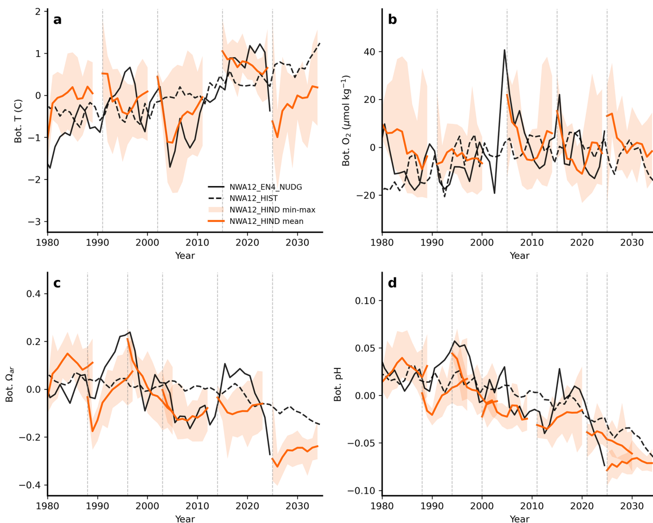
Figure 6. Physical and biogeochemical predictions in the GOM. Annual mean anomalies of (a) bottom temperature ( ^{\circ}\text{C} ), (b) bottom oxygen ( \mu\text{mol kg}^{-1} ), (c) bottom aragonite saturation state and (d) bottom pH in the GOM_EPU. The solid black lines show the anomalies from the ensemble mean of regional downscaled simulations (NWA12_EN4_NUDG, as in Fig. 2), the dashed black lines show the ensemble mean of uninitialized downscaled model simulations (NWA12_HIST) carried under historical anthropogenic forcing and SSP585 emissions scenario. The bold orange lines show the 10-yearlong initialized prediction (NWA12_HIND) and the vertical grey lines depict their year of initialization. The bold orange lines are the ensemble means of the respective 10-member ensemble, and the light shading is the min-max range of the ensemble members. A lead-time-dependent climatology was removed from each ensemble member to create anomalies. All anomalies are calculated with respect to the 1994–2023 mean.
