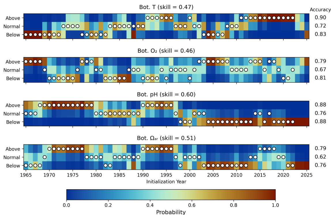
Figure 7. Probabilistic predictions for the GOM. Probability of the predicted lead 1–3 year mean anomalies (with respect to the 1994–2023 mean) of (a) bottom temperature, (b) bottom O 2 , (c) bottom pH and (d) bottom Ω ar from the regional downscaled decadal prediction model (NWA12_HIND). The corresponding classifications of the reference anomalies are shown as white circles from the regional down-scaled simulation (NWA12_EN4_NUDG). The tercile boundaries are calculated separately for the predictions and reference/observations. The x axis shows the initialization year and the 2025 forecast. The forecast accuracy, (True Positives + True Negatives)/Total forecasts, for each tercile is shown on the right. A random forecast that randomly picks one tercile as most likely for each forecast has an accuracy of 0.56 and the accuracy of a consistently negative (counter) prediction is 0.67. The forecast skill compared to persistence is given in the subtitle of each panel.
