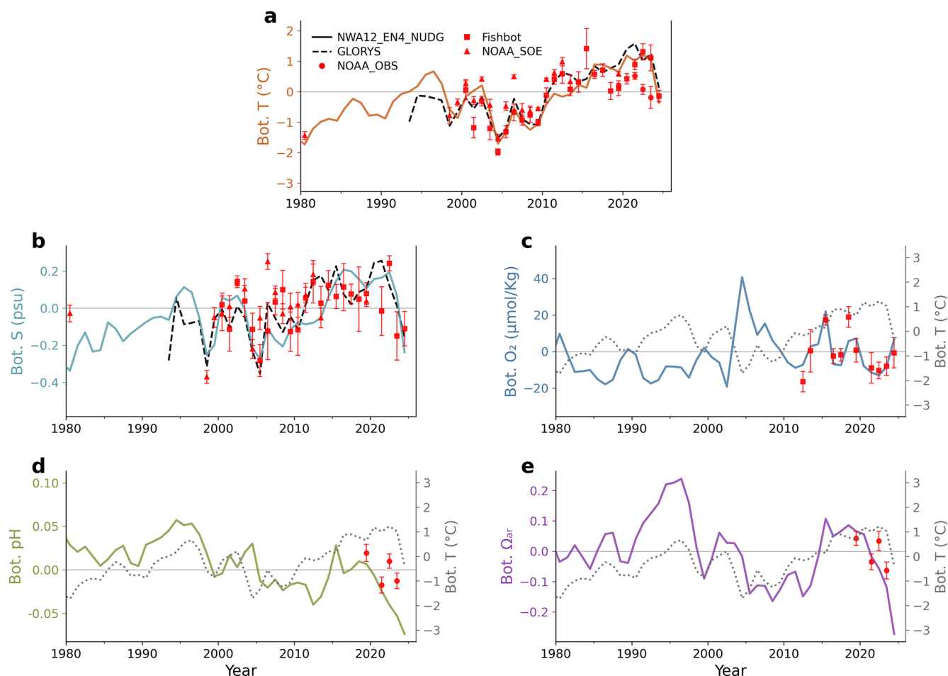
Figure 2. Physical and biogeochemical variability in the GOM. Annual mean anomalies of (a) bottom temperature ( ^{\circ}\text{C} ), (b) bottom salinity (psu), (c) bottom oxygen ( \mu\text{mol kg}^{-1} ), (d) bottom pH and (e) bottom aragonite saturation state in the GOM from the ensemble mean of the regional downscaled simulations (NWA12_EN4_NUDG, colored solid lines) and observations (markers with error bars). Observations from the NOAA SOE reports (NOAA_SOE, triangles), the Fishbot bottom data (squares) and the aggregated point observations from vessels and gliders (NOAA_OBS, circles) are also shown for available years. The error bars depict the uncertainty of the annual mean (see Sect. 2). The dashed black lines in (a) and (b) are from the GLORYS12 dataset. All anomalies are calculated with respect to the 1994–2023 mean. To highlight physical and biogeochemical co-variability, bottom temperature lines are shown as dotted grey lines in (c)–(e).
