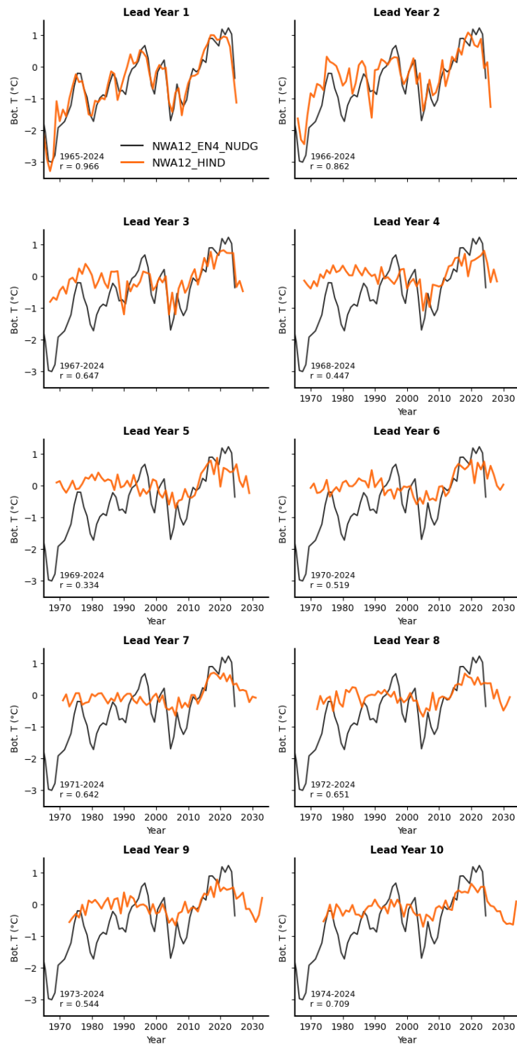
Fig. S9: Lead Year Predictions. Ensemble mean anomalies of predicted annual bottom temperature in the Gulf of Maine from the NWA12_HIND at each lead year (orange) and from the regional downscaled simulation (NWA12_EN4_NUDG, black). The time period of each lead year time series and its respective correlation with NWA12_EN4_NUDG is also shown.
