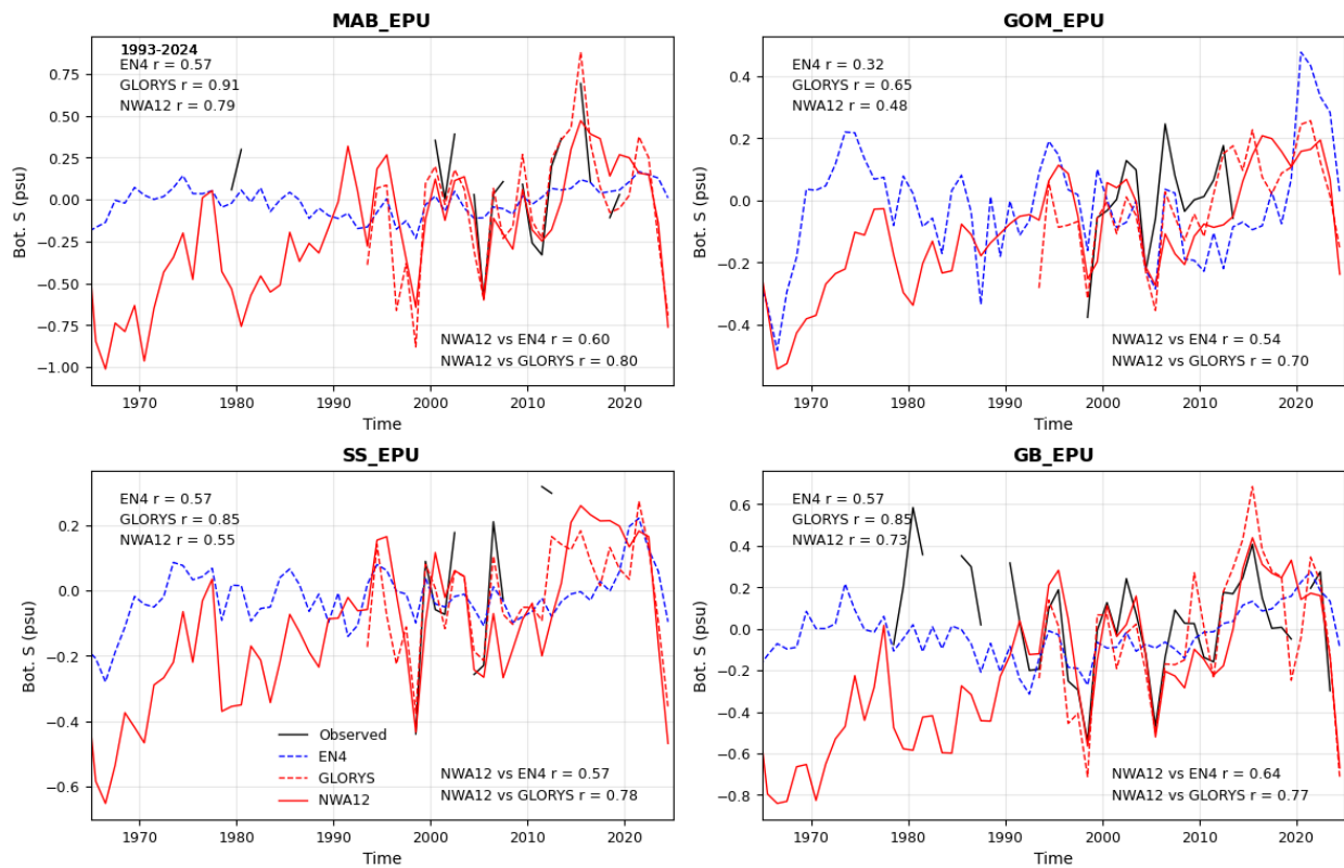
Fig. S2: Comparison of Bottom Salinity. Same as Fig. S1 but for bottom salinity.
