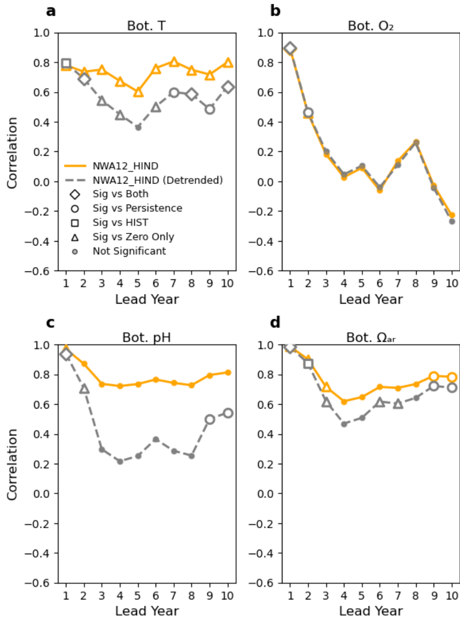
Fig. S4: Decadal prediction skill. Same as Fig 3 in the main text but for correlation skill verified against GLORYS12 reanalysis for (a) bottom temperature and against the regional downscaled simulation (NWA12_EN4_NUDG) for (b) bottom O 2 , (c) bottom pH and (d) bottom Ω ar all computed over the period 1993-2024.
