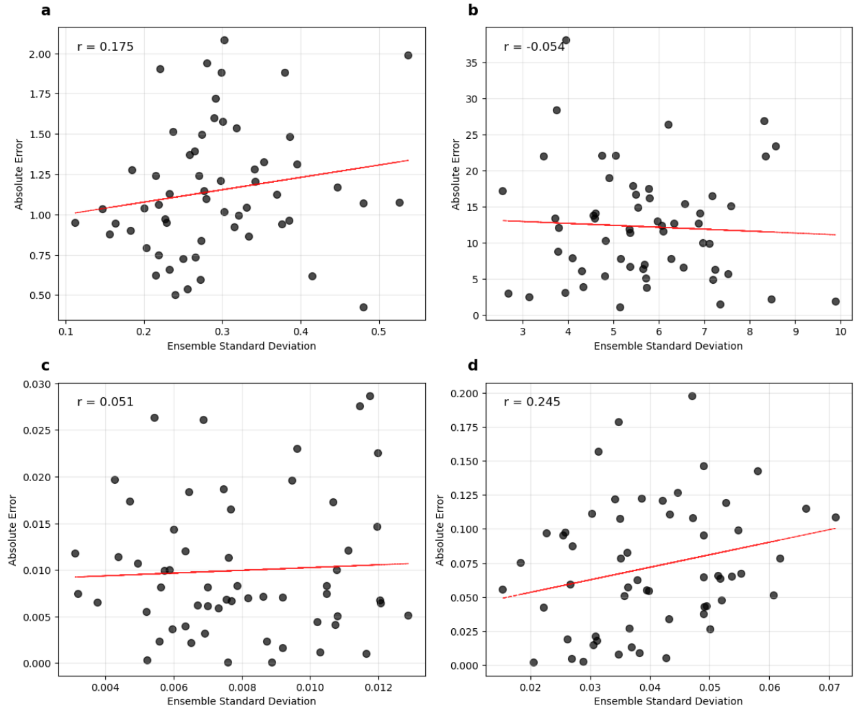
Fig. S8: Lead 1-3 Mean Ensemble Standard Deviation vs. Absolute Error. Ensemble standard deviation plotted against the absolute error of the ensemble mean (averaged over lead years 1-3) for bottom (a) temperature, (b) O_2 , (c) pH and (d) \Omega_{ar} . Red lines represent the best fit lines, and the correlation coefficients ( r ) quantify the strength of the relationship between the ensemble standard deviation and the absolute error.
