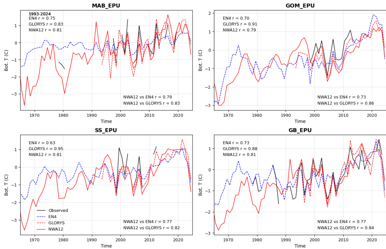
Fig. S1: Comparison of Bottom Temperature. Annual mean temperature anomalies of bottom temperature from the NWA12_EN4_NUDG, GLORYS12 reanalysis, the EN4 dataset and NOAA_SOE observations for the four EPUs—MAB_EPU, GOM_EPU, SS_EPU and GB_EPU. The correlation coefficients between the NOAA-SOE and NWA12/GLORYS12/EN4 datasets, and between the NWA12 and GLORYS12/EN4 datasets for the common 1993-2024 period are also shown.
