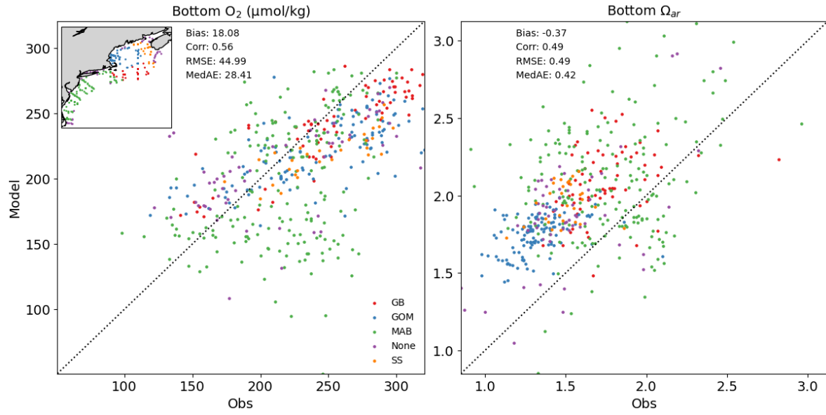
Fig. S7: Comparison with Point Observations. Pointwise comparison of bottom O 2 and bottom \Omega_{ar} from the regional downscaled model with NOAA_OBS in the various Ecological Processing Units (EPUs)—GOM_EPU, MAB_EPU, GB_EPU and SS_EPU.
