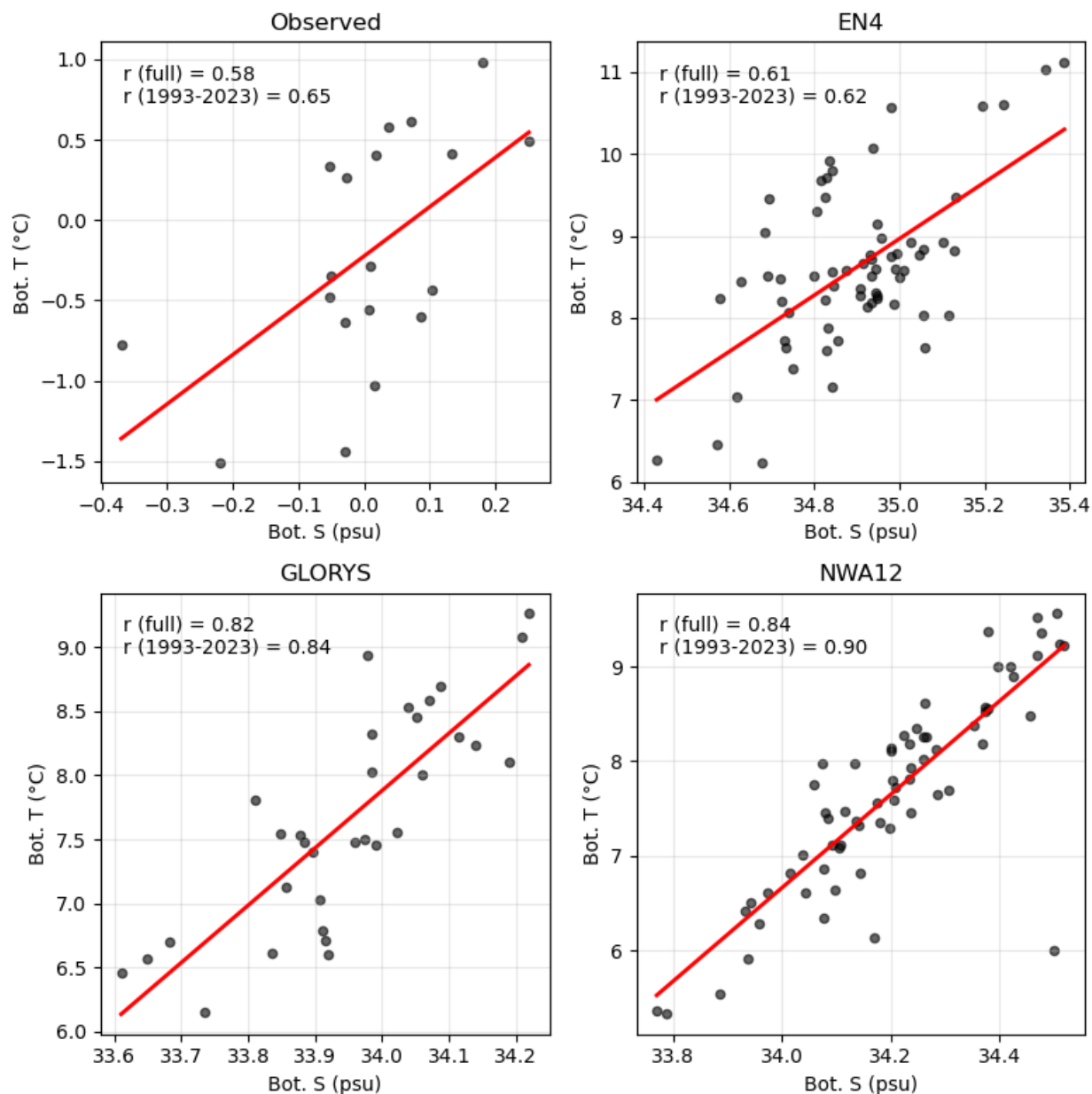
Fig. S3: Bottom temperature and bottom salinity in the GOM Correlation between bottom temperature and bottom salinity in the GOM_EPU for NOAA_SOE observations, EN4 dataset, GLORYS12 reanalysis and the regional downscaled model (NWA12_EN4_NUDG). Correlation values are shown for the common (1993-2023) and full period of the respective dataset.
