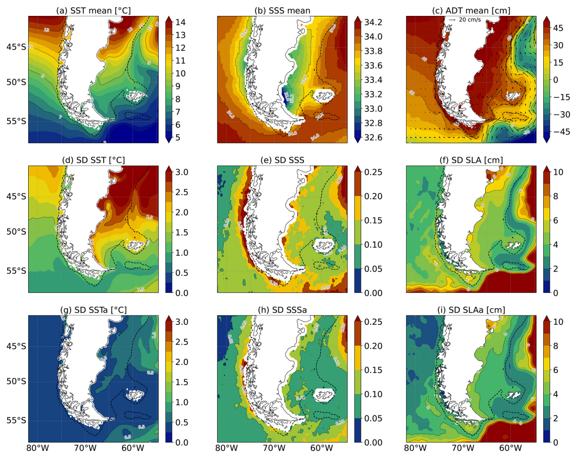
Figure 2. Mean fields of SST (a), SSS (b), and ADT (c) and their standard deviations. Panels (d), (e) and (f) show the standard deviation of the low-pass filtered time series with respect to the mean fields, thus including seasonal variability. Panels (g), (h), and (i) display the standard deviation of the anomalies after removing the annual signal. Colour intervals for the mean and standard deviations are 0.5 and 0.25 °C (SST), 0.1 and 0.05 (SSS), and 5 and 1 cm (ADT). The black arrows in panel (c) represent the mean geostrophic velocity vectors calculated from the ADT (scale shown in panel (c)). The black dashed line in all maps indicates the 200 m isobath.
