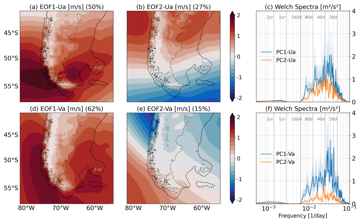
Figure 5. EOF patterns of zonal (Ua) and meridional (Va) wind anomalies. Panels (a) and (b) show EOF1 and EOF2 of zonal wind anomalies, while panels (d) and (e) show EOF1 and EOF2 of meridional wind anomalies. Colour intervals are 0.2\text{ m s}^{-1} . The black dashed line on the EOF maps indicates the 200 m isobath. Panels (c) and (f) display the power spectra of the corresponding principal component time series for zonal and meridional wind anomalies, respectively, estimated using Welch’s method. In the spectral plots, blue and orange curves represent the spectra of the first and second principal components, respectively. Spectra are displayed in a variance-preserving form to highlight the distribution of variance across frequency bands.
