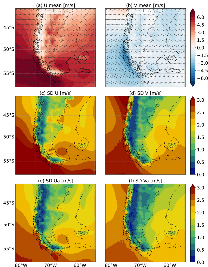
Figure 3. Mean fields of zonal ((a) \text{m s}^{-1} ) and meridional wind ((b) \text{m s}^{-1} ) components and their standard deviation. Panels (c) and (d) show the standard deviation of the low-pass filtered time series with respect to the mean fields, thus including seasonal variability. Panels (e) and (f) display the standard deviation of the wind anomalies, after removing the annual signal. The colour intervals are drawn every 0.5 \text{ m s}^{-1} in the mean fields and 0.25 \text{ m s}^{-1} in the standard deviation maps. The black arrows in panels (a) and (b) represent the mean wind vectors (scale shown at the top of panels). The black dashed line in all maps indicates the 200 m isobath.
