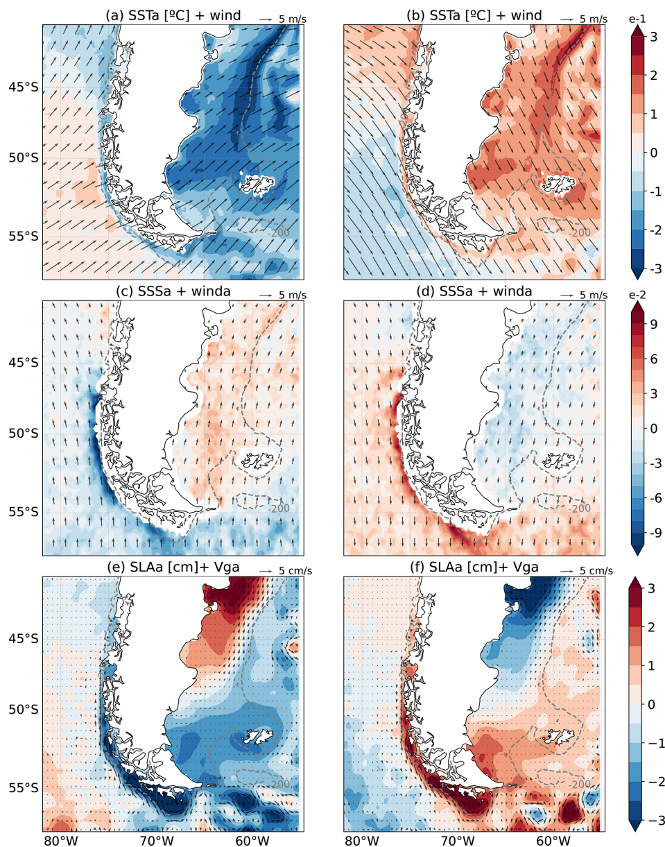
Figure 6. Composites for the positive (southerly winds) and negative (northerly winds) phases of the leading mode of the meridional wind. Panels (a), (c), and (e) show SST, SSS, and SLA anomalies for the positive phase, while panels (b), (d), and (f) show these anomalies for the negative phase. Black arrows represent wind composites in panels (a) and (b), wind anomalies in panels (c) and (d), and ocean geostrophic velocity anomalies in panels (e) and (f). Gray dashed lines indicate the 200 m isobath.
