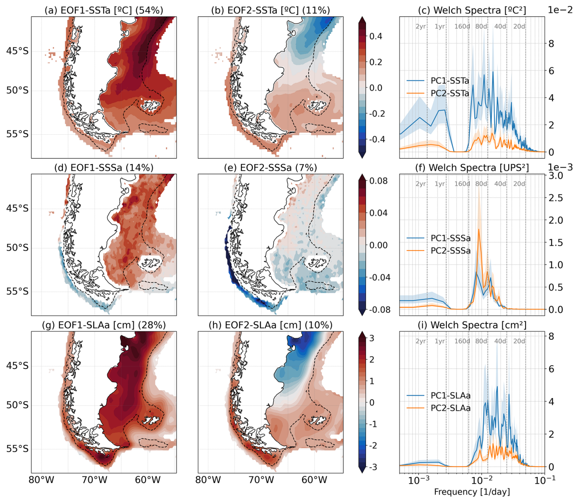
Figure 4. EOF analysis results for SSTa, SSSa, and SLAa. Panels (a) and (b) show the first and second EOF modes of SSTa, panels (d) and (e) show EOF1 and EOF2 of SSSa, and panels (g) and (h) show EOF1 and EOF2 of SLAa. Colour intervals are 0.05^{\circ}\text{C} for SSTa, 0.01 salinity units for SSSa, and 0.2\text{ cm} for SLAa. Black dashed lines in the EOF maps indicate the 200\text{ m} isobath. Panels (c), (f), and (i) display the power spectra of the corresponding PC time series for SSTa, SSSa, and SLAa, respectively, estimated using Welch's method. In the spectral plots, blue and orange curves correspond to the spectra of the first and second PCs, respectively. Spectra are shown in a variance-preserving form to emphasize the relative contribution of different frequency bands.
