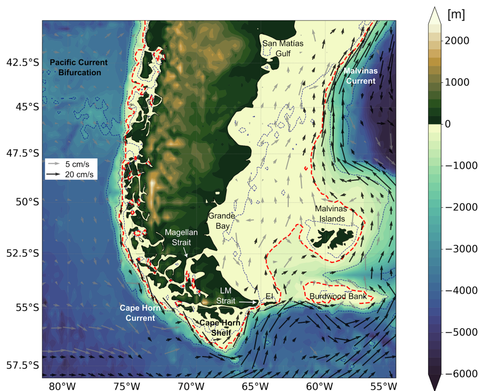
Figure 1. Mean circulation around South America inferred from the Mean Dynamic Topography for the period 1993–2022. Gray arrows indicate velocities lower than 8 \text{ cm s}^{-1} , and black arrows indicate velocities greater than 10 \text{ cm s}^{-1} . Note the different scales. Colours show bathymetry (yellow and blue) and land topography (green and brown), in meters. Bathymetry data are from GEBCO Bathymetric Compilation Group (2023). The red dashed line marks the 200 m isobath, close to the continental shelf break. Blue dashed lines indicate the 100, 1000, and 3000 m isobaths. LM: Le Maire Strait. EI: Estados Islands.
