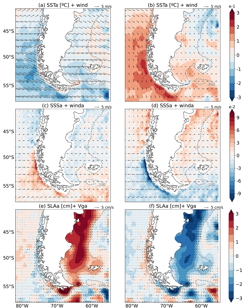
Figure 7. Composites for the positive (increased westerlies) and negative (decreased westerlies) phases of the leading mode of the zonal wind. Panels (a), (c), and (e) show SSTa, SSSa, and SLAa anomalies for the positive phase, while panels (b), (d), and (f) show these anomalies for the negative phase. Black arrows represent wind composites in panels (a) and (b), wind anomalies in panels (c) and (d), and ocean geostrophic velocity anomalies in panels (e) and (f). Gray dashed lines indicate the 200 m isobath.
