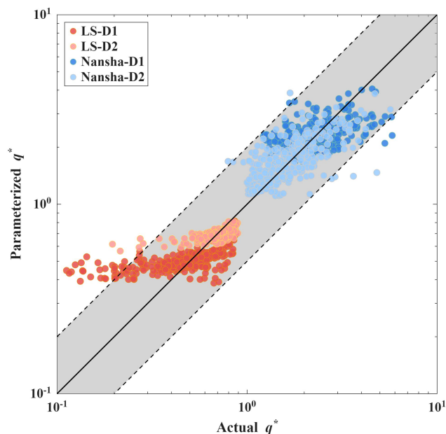
Figure 6. Scatter plot of parameterized q^* versus actual q^* for the LS and the Nansha Islands. The black line denotes the 1 : 1 reference line, and the two outer black dashed lines represent the 2 : 1 and 1 : 2 bounds.
