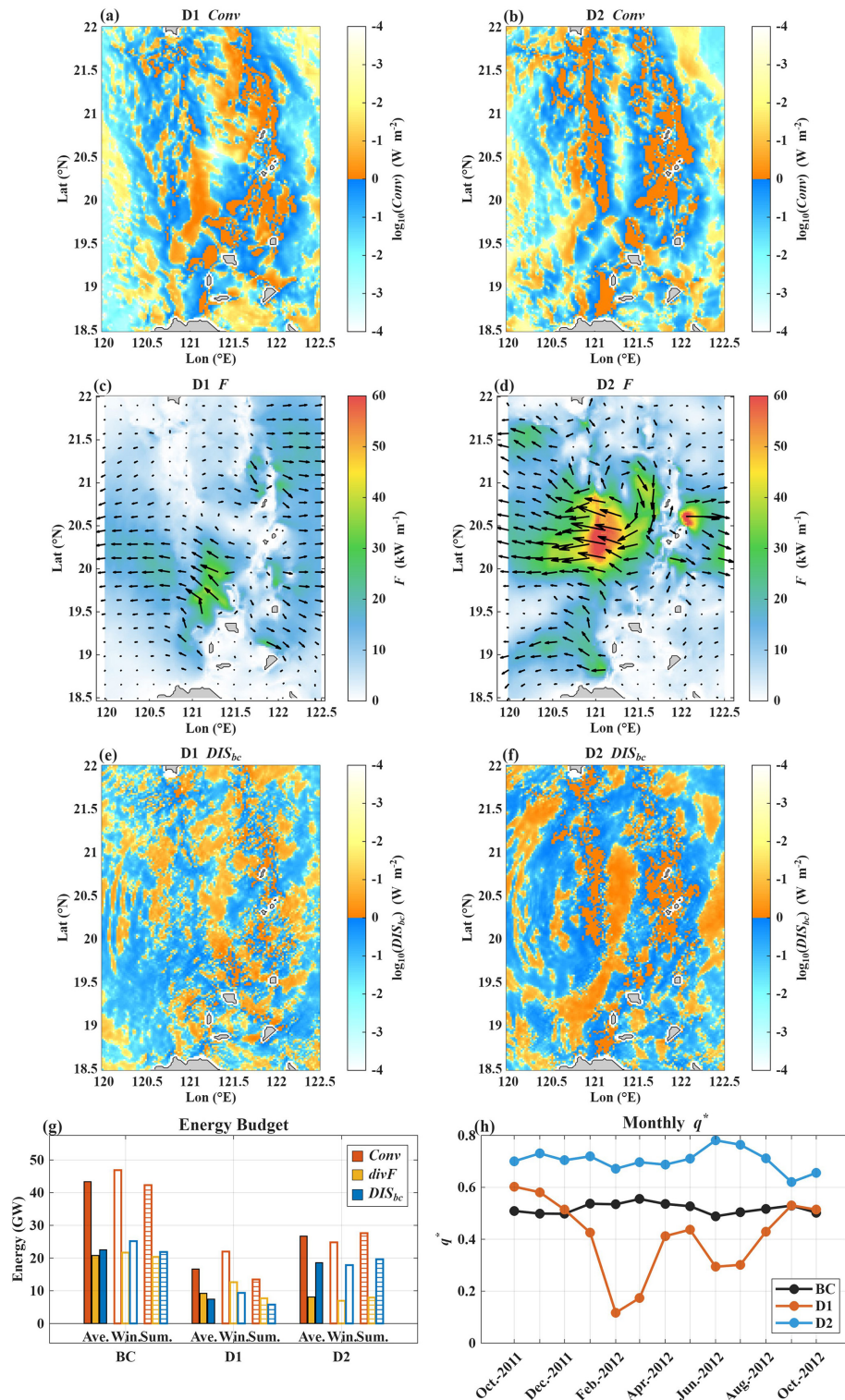
Figure 2. (a–f) Spatial distributions of the diurnal and semidiurnal internal tidal energy budget terms in the LS during summer. \langle \text{Conv} \rangle is the tidal-period mean depth-integrated barotropic-to-baroclinic energy conversion, \langle F \rangle is the tidal-period mean depth-integrated internal tidal energy flux, and \langle \text{DIS}_{bc} \rangle is the tidal-period mean depth-integrated local internal tidal dissipation. (g) Bar chart of the budget terms. \langle \text{div}F \rangle is the tidal-period mean divergence of the depth-integrated internal tidal energy flux. “Ave.”, “Win.”, and “Sum.” stand for the annual-, winter-, and summer-mean values, respectively. BC, D1, and D2 represent the total internal tide, diurnal tide, and semidiurnal tide, respectively. (h) Time series of the monthly-mean local internal tidal dissipation ratio, q^* . In (a), (b), (e) and (f), the units for \text{Conv} and \text{DIS}_{bc} are \text{W m}^{-2} , with orange (blue) representing positive (negative) values. In (c) and (d), the unit for F is \text{kW m}^{-1} , with colors representing magnitude and arrows indicating direction. In (g), the units for \text{Conv} , \text{div}F , and \text{DIS}_{bc} are GW.
