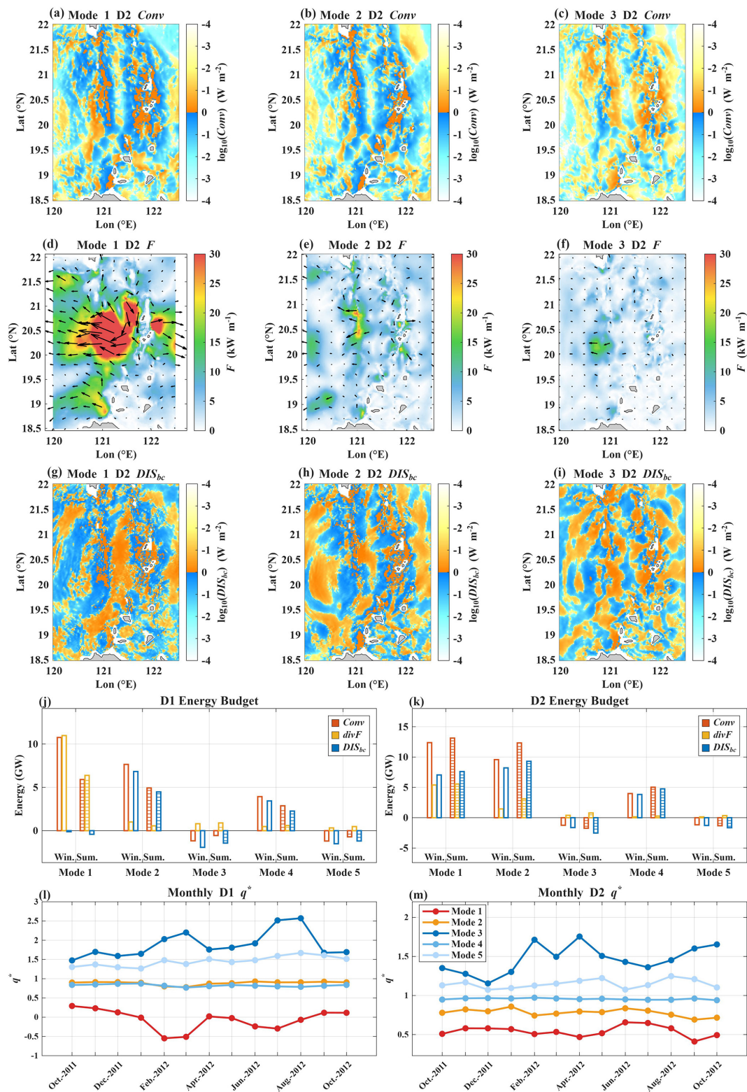
Figure 3. (a–i) Spatial distributions of the semidiurnal internal tidal energy budget terms for modes 1–3 in the LS during summer. (j, k) Bar charts of the energy budget terms for modes 1–5, and (l, m) time series of monthly-mean q^* for modes 1–5 for diurnal (D1) and semidiurnal (D2) tides, respectively. “Win.” and “Sum.” stand for winter and summer, respectively. In (a)–(c) and (g)–(i), the units for Conv and \text{DIS}_{bc} are \text{W m}^{-2} , with orange (blue) indicating positive (negative) values. In (d)–(f), the unit for F is \text{kW m}^{-1} , with colors indicating magnitude and arrows indicating direction. In (j) and (k), the units for Conv, \text{div}F , and \text{DIS}_{bc} are GW. In (l) and (m), monthly mean values of q^* outside the displayed y axis ranges are not shown for clarity.
