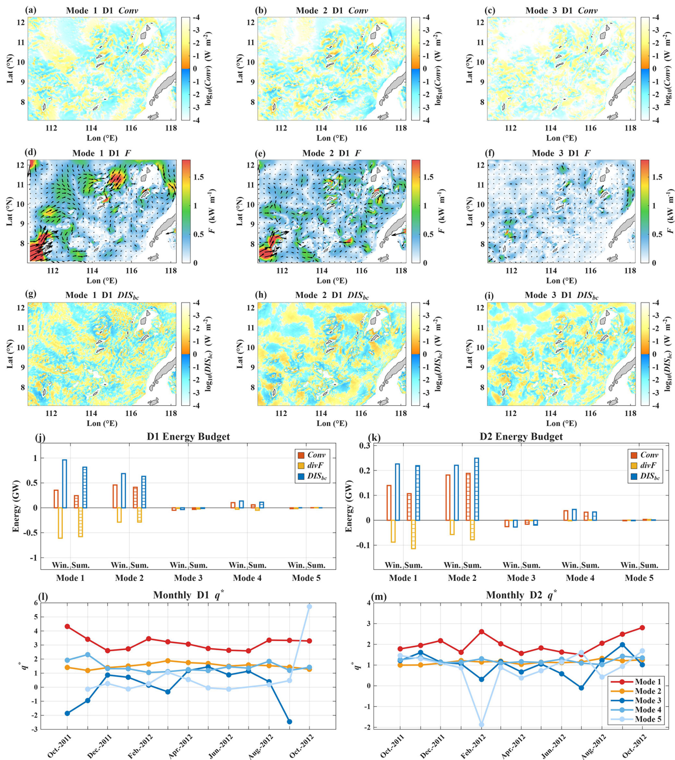
Figure 5. Same as Fig. 3, but for the Nansha Islands and (a–i) for diurnal internal tide.
