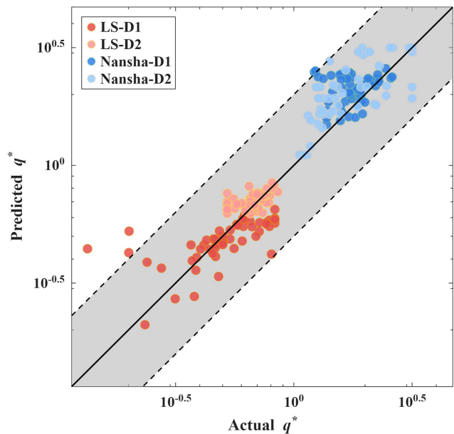
Figure 7. Scatter plot of the predicted q^* from the XGBoost model versus the actual q^* for the LS and the Nansha Islands. The black line represents the 1 : 1 reference line, and the two outer black dashed lines represent the 2 : 1 and 1 : 2 bounds.
