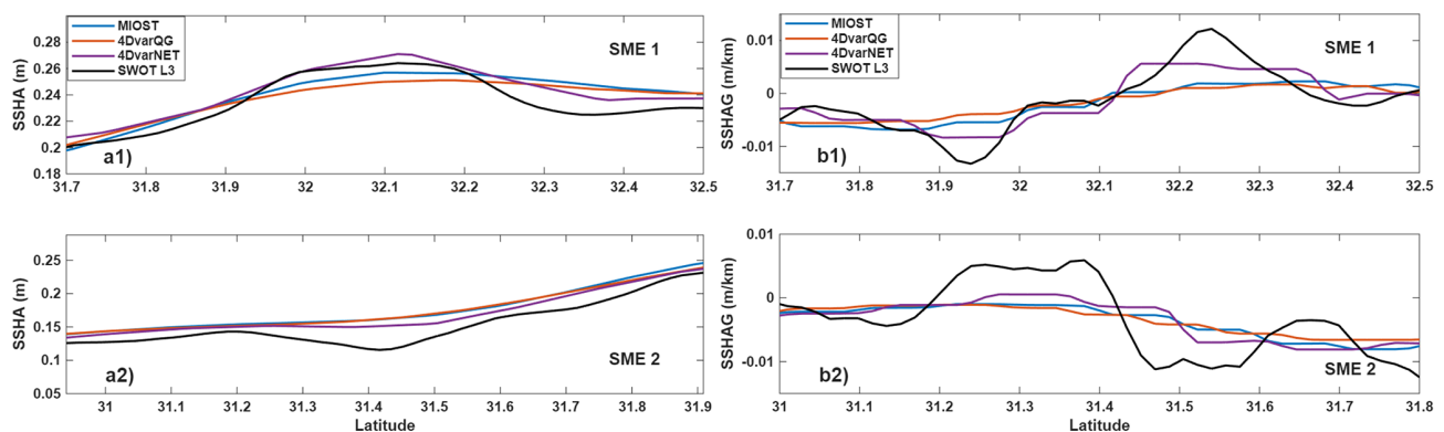
Figure 14. Cross-sectional SSHA and gradient profiles across the eddy core in Case 3 (section indicated in Fig. 12a1), same as Fig. 9.
