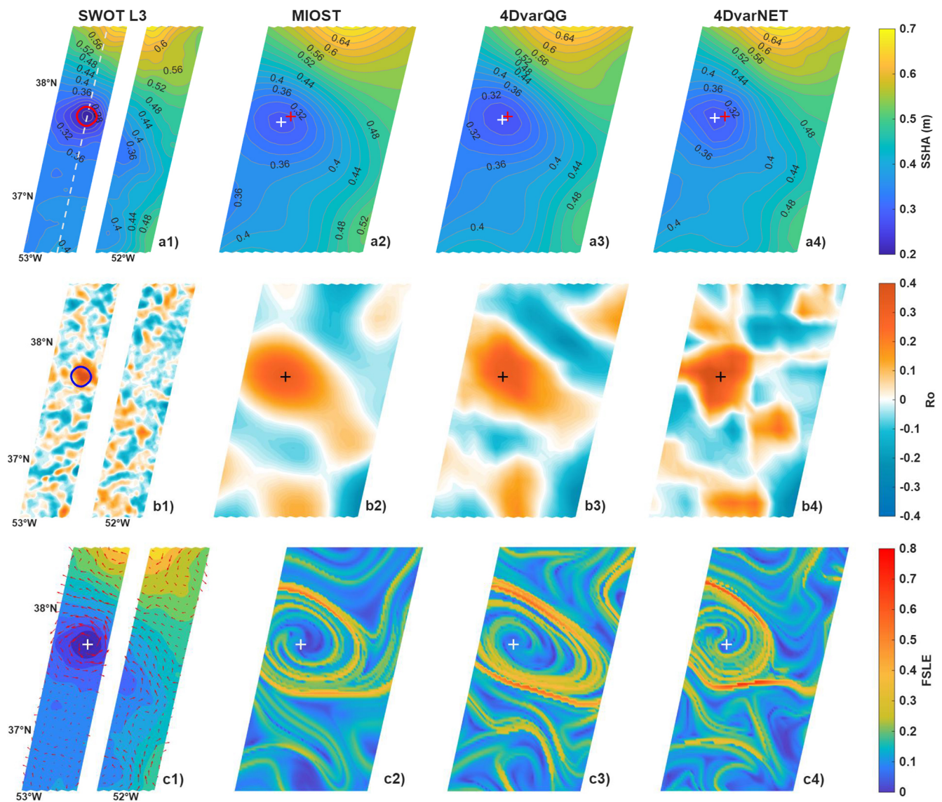
Figure 11. Case 2 (SWOT L3 cycle 002, pass 089; 14 August 2023), presented with the same layout and diagnostics as Fig. 8.
