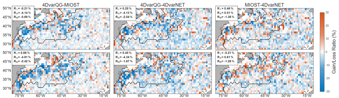
Figure 4. Pairwise comparison of RMSE gain / loss ratio R computed on 1^\circ \times 1^\circ grids. Columns correspond to comparisons between different L4 products, and rows correspond to meridional (top) and zonal (bottom) velocity components. Blue shading indicates negative R values, corresponding to reduced RMSE and superior performance of the first product in each comparison; red shading indicates increased RMSE. Region-averaged gain / loss ratios for total velocity RMSE within each dynamic regime are indicated in the upper-left annotation of each panel.
