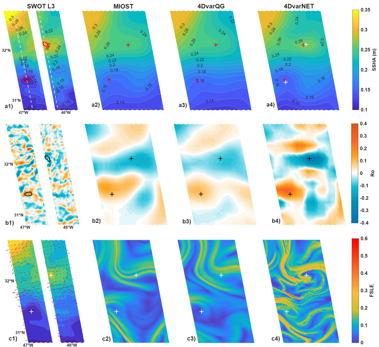
Figure 13. Case 3 (SWOT L3 cycle 001, pass 324; 1 August 2023), presented with the same layout and diagnostics as Fig. 8.
