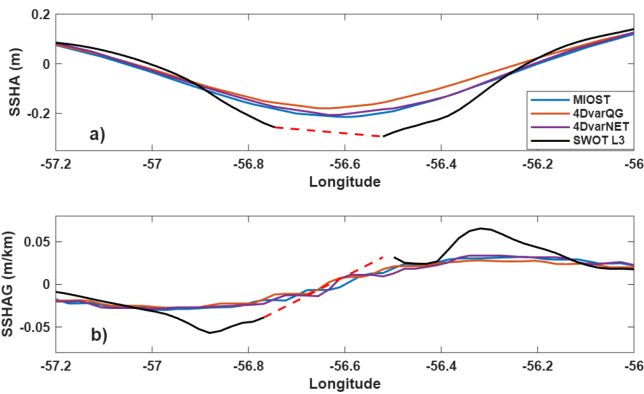
Figure 10. Cross-sectional comparison of SSHA and its along-track gradient across the eddy core in Case 1 (section indicated in Fig. 8a1). (a) SSHA profiles and (b) corresponding SSHAG gradients from SWOT L3 and L4 products. Differences in amplitude and gradient sharpness highlight the products’ varying ability to reconstruct eddy intensity and frontal structure.
