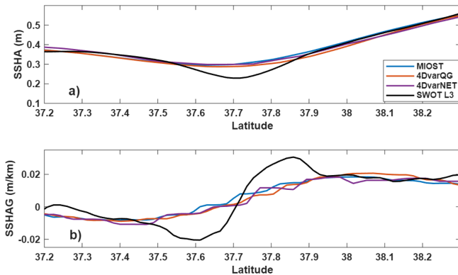
Figure 12. Cross-sectional SSHA and gradient profiles across the eddy core in Case 2 (section indicated in Fig. 10a1), same as Fig. 9.
