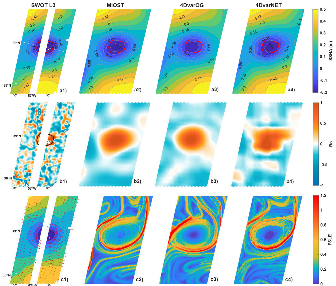
Figure 9. Case 1 (SWOT L3 cycle 002, pass 145; 16 August 2023). Spatial comparison of: (a) sea surface height anomaly (SSHA), (b) Rossby number ( R_o ), (c) Geostrophic current of SWOT L3 (left column) and FSLE derived from three L4 products (MIOST, 4DvarQG, 4DvarNET). White crosses mark SWOT-identified eddy cores; colored crosses indicate reconstructed cores from each product. Note that R_o color scales differ to account for sharper gradients and higher amplitudes in SWOT L3 relative to L4 reconstructions.
