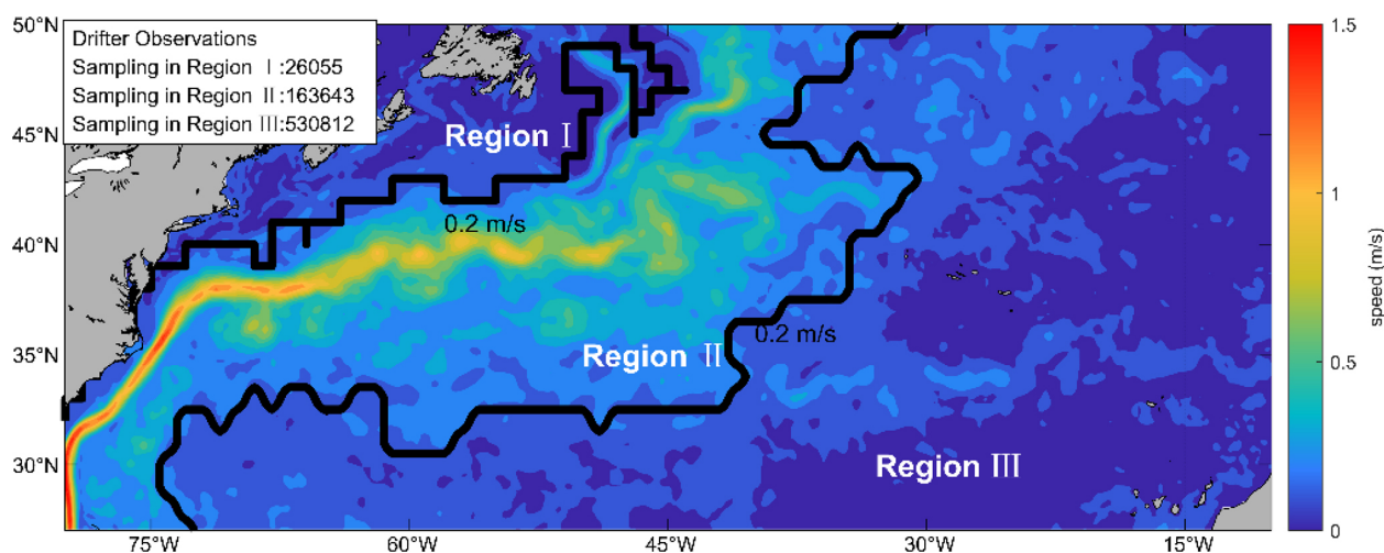
Figure 2. Mean surface velocity and dynamic regime partition derived from DUACS geostrophic velocity fields over 27 July 2023–20 April 2024. Black contours delineate the boundaries of the three dynamic regimes, broadly following the 0.2 \text{ m s}^{-1} speed contour. Moderate spatial smoothing was applied to ensure coherent regime boundaries. The number of drifter samples within each regime is annotated in the upper-left corner.
