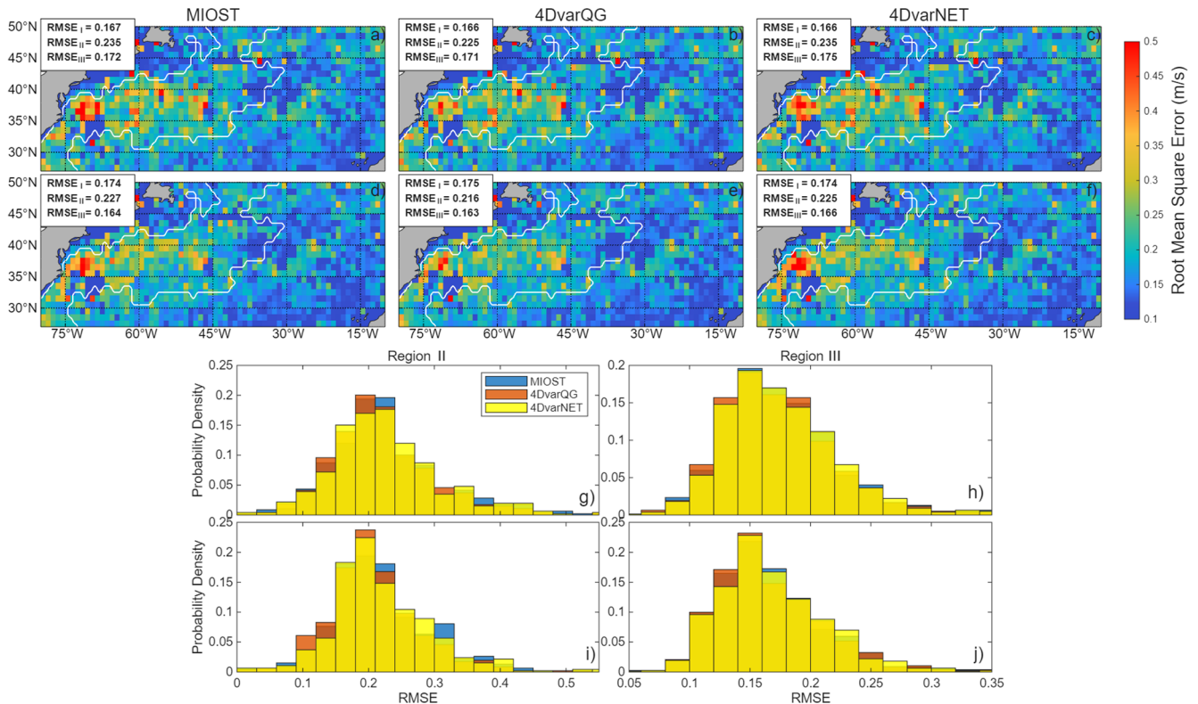
Figure 3. (a–f) The RMSE of L4 products computed on 1^\circ \times 1^\circ grids. Columns correspond to different L4 products, and rows correspond to meridional (top) and zonal (bottom) velocity components. Region-averaged velocity RMSE within each dynamic regime are indicated in the upper-left annotation of each panel. (g–j) PDFs of the RMSE in Regions II and III, for zonal and meridional velocity components.
