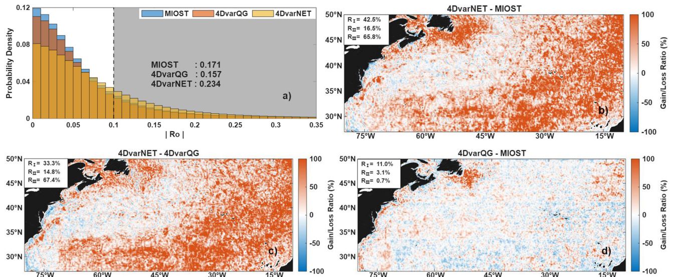
Figure 7. (a) PDFs of the absolute Rossby number |Ro| for the three L4 products. Mean |Ro| values are annotated. (b–d) Spatial distributions of the |Ro| gain / loss ratio between pairs of products. Warm colors indicate regions where the first-listed product exhibits larger |Ro| relative to the reference product, while cold colors indicate regions where it exhibits smaller |Ro| . Insets report region-averaged gain / loss ratios ( R ) over the three predefined dynamical regimes.
