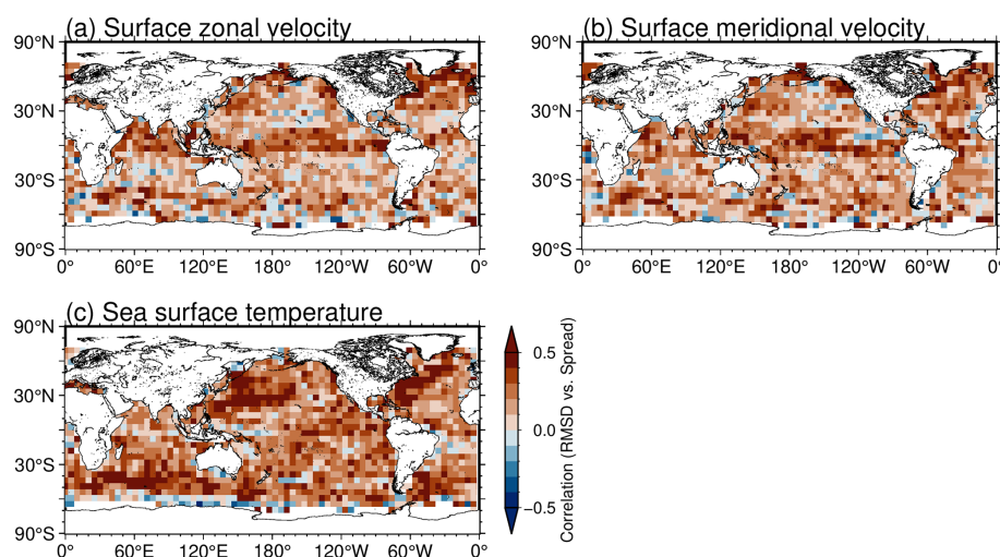
Figure 19. Temporal correlation coefficients between monthly analysis ensemble spread and analysis RMSDs of LORA-QG relative to drifter buoys in 5^\circ longitude \times 5^\circ latitude bins for the surface (a) zonal and (b) meridional velocities and (c) SST fields.
