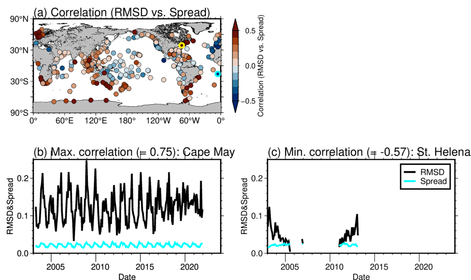
Figure 20. (a) Temporal correlation coefficients between monthly analysis ensemble spread and analysis RMSDs of LORA-QG relative to sea level anomalies from tide gauge observations. Time series of the monthly analysis ensemble spread (cyan) and analysis RMSDs (black) at (b) Cape May and (c) St. Helena with the maximum and minimum correlation coefficients (yellow and cyan circles in Fig. 20a, respectively).
