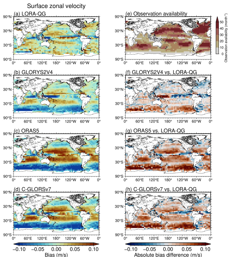
Figure 8. (a–d) Same as Fig. 7a–d, but for temporally averaged analysis biases. (e) The observation availability of the surface drifter buoys. (f–h) Same as Fig. 7f–h, but for the absolute bias differences relative to LORA-QG. In (f)–(h), red and blue colors denote that the absolute biases in LORA-QG are smaller and larger than those of the other datasets, respectively; dot marks indicate statistically significant differences in the absolute biases at the 99 % confidence level.
