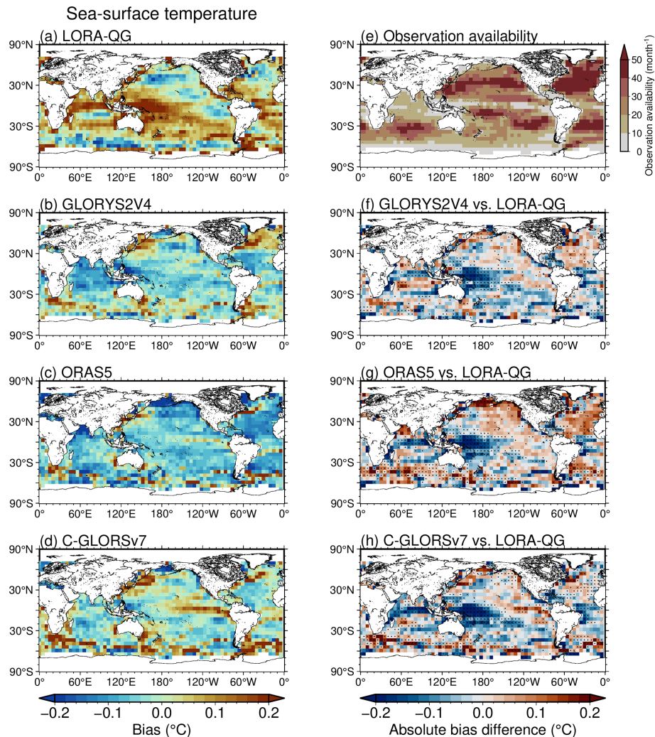
Figure 10. Same as Fig. 8, but for SST.
