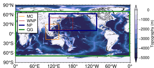
Figure 1. Domains of the local ensemble transform Kalman filter (LETKF)-based Ocean Research Analysis (LORA): the Maritime Continent (orange), western North Pacific (red), North Pacific (blue), and quasi-global (green) domains. Colors indicate topography derived from a 1 arcmin global relief model of Earth's surface (ETOPO1; Amante and Eakins, 2009).
