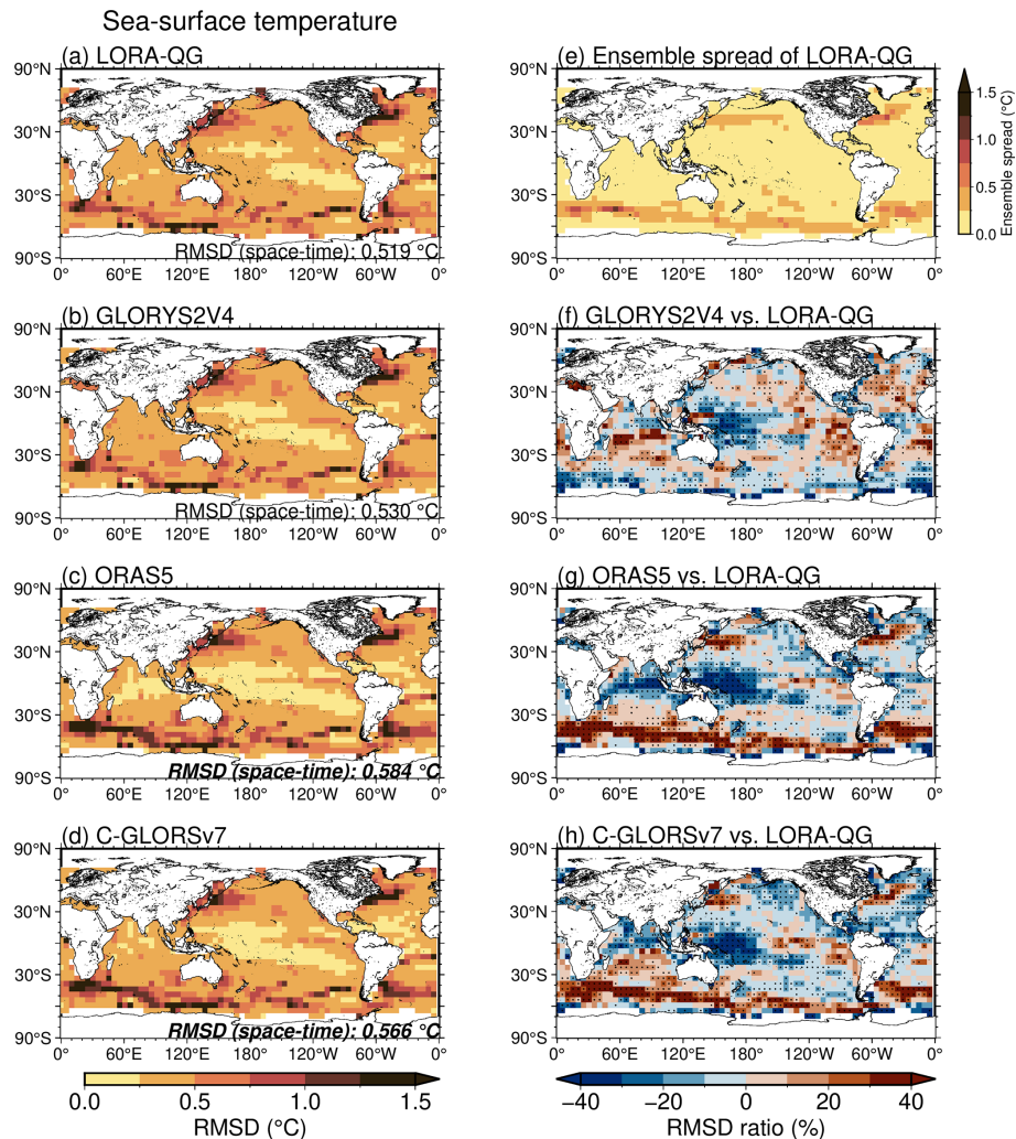
Figure 9. Same as Fig. 7, but for SST.
