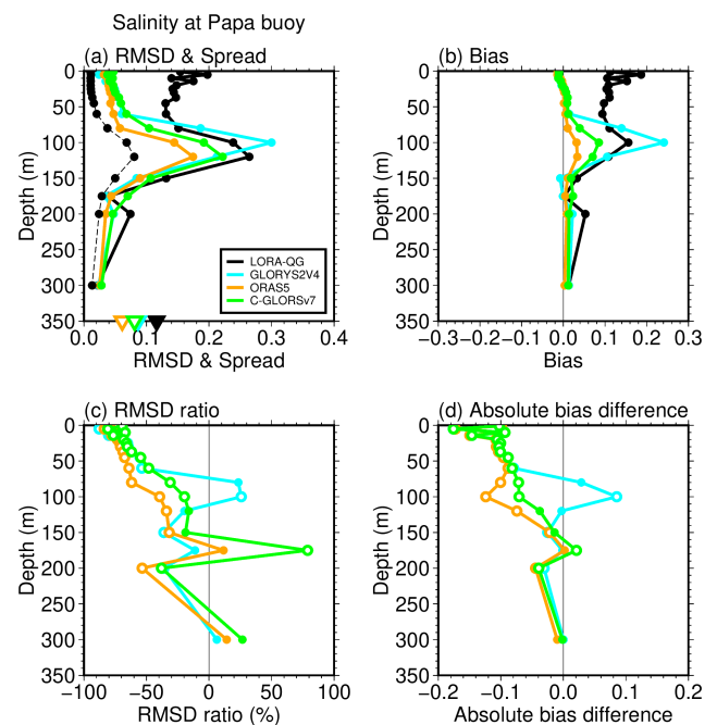
Figure 18. Same as Fig. 15, but for salinity at the Papa buoy. The ranges of the horizontal and vertical axes differ from those in Fig. 16.
