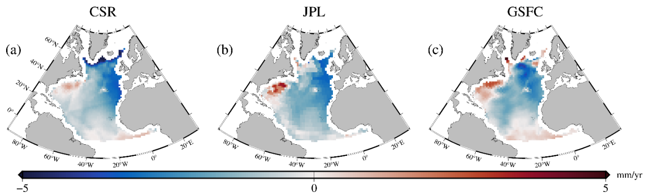
Figure S1 : Manometric sea level trends in the North Atlantic over 2004.01-2022.12 derived from the three GRACE mascon solutions. (a) from CSR. (b) from JPL, and (c) from GSFC.
