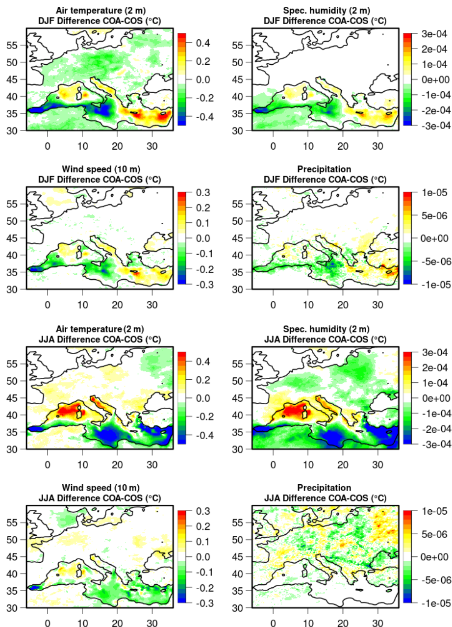
Figure 5. Long-term averaged (2000–2020) near-surface atmospheric parameter differences between COA and COS sensitivity experiments (namely, showcasing the impact of ocean data assimilation on atmospheric variables).
