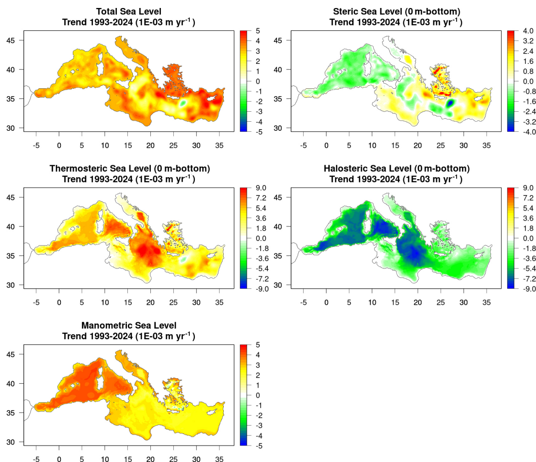
Figure 13. Maps of linear trends (1993–2024) for sea level and its components, from MESMAR-R.
