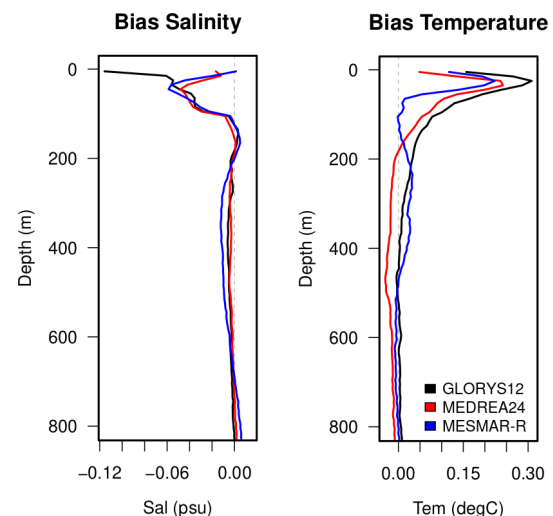
Figure 1. Profiles of salinity (left panel) and temperature (right panel) bias, calculated against all available in-situ profiles, for MESMAR-R in comparison with other state-of-the-art reanalyses. The calculation covers the period 2000–2020, and the bias is defined as model minus observations.
