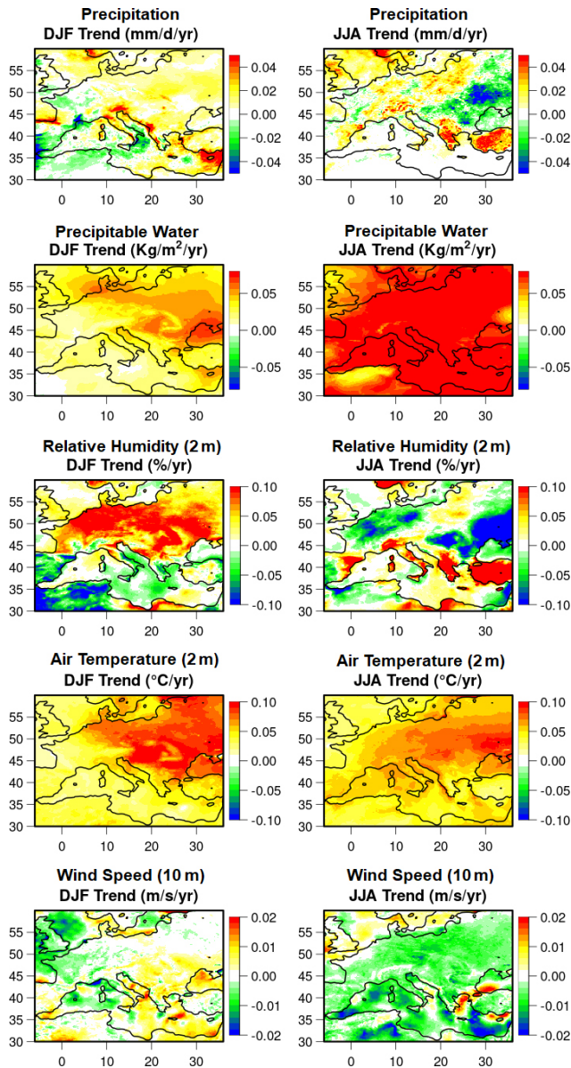
Figure 16. Winter (DJF) and summer (JJA) trends of selected atmospheric variables from MESMAR-R, computed over the period 1993–2024.
