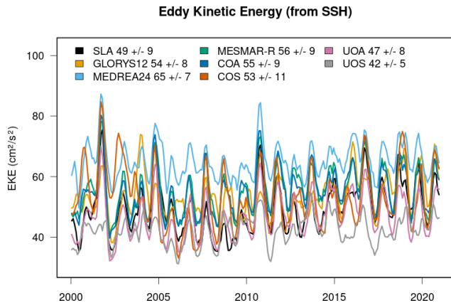
Figure 7. Eddy kinetic energy (EKE) timeseries, calculated from the MESMAR-R reanalysis, gridded altimetry data, the MEDREA24 and GLORYS12, and the sensitivity experiments, over the period 2000–2020. For all datasets, EKE is calculated from sea level, adopting the usual geostrophic relationship to calculate geostrophic currents.
