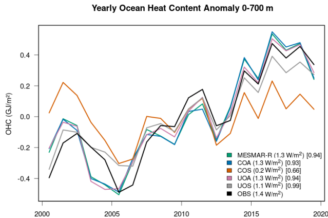
Figure 9. Yearly ocean heat content anomalies for the period 2000–2020 from MESMAR-R, the sensitivity experiments, and observation-based values. The legend also reports the trend in \text{W m}^{-2} , and the correlation with the observation-based time series.
