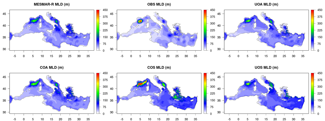
Figure 10. Long-term mean winter mixed layer depth (JFM) over 2000–2020 for the MESMAR-R reanalysis and the sensitivity experiments, together with values derived from in-situ observations.
