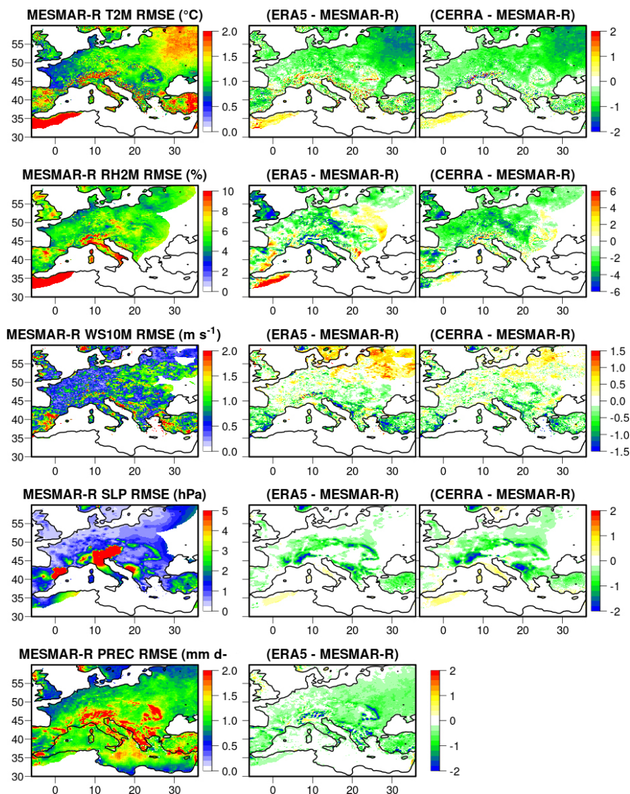
Figure 3. Maps of RMSE against atmospheric near-surface gridded observations (T2M in ^{\circ}\text{C} , RH2M in %, WS10M in \text{m s}^{-1} , SLP in hPa, and PREC in \text{mm d}^{-1} ), in comparison with other state-of-the-art reanalyses. Left panels show the MESMAR-R RMSE, while middle and right panels show the RMSE difference between either ERA5 or CERRA and MESMAR-R (where positive, MESMAR-R provides the smallest RMSE). The calculation covers the period 2000–2020.
