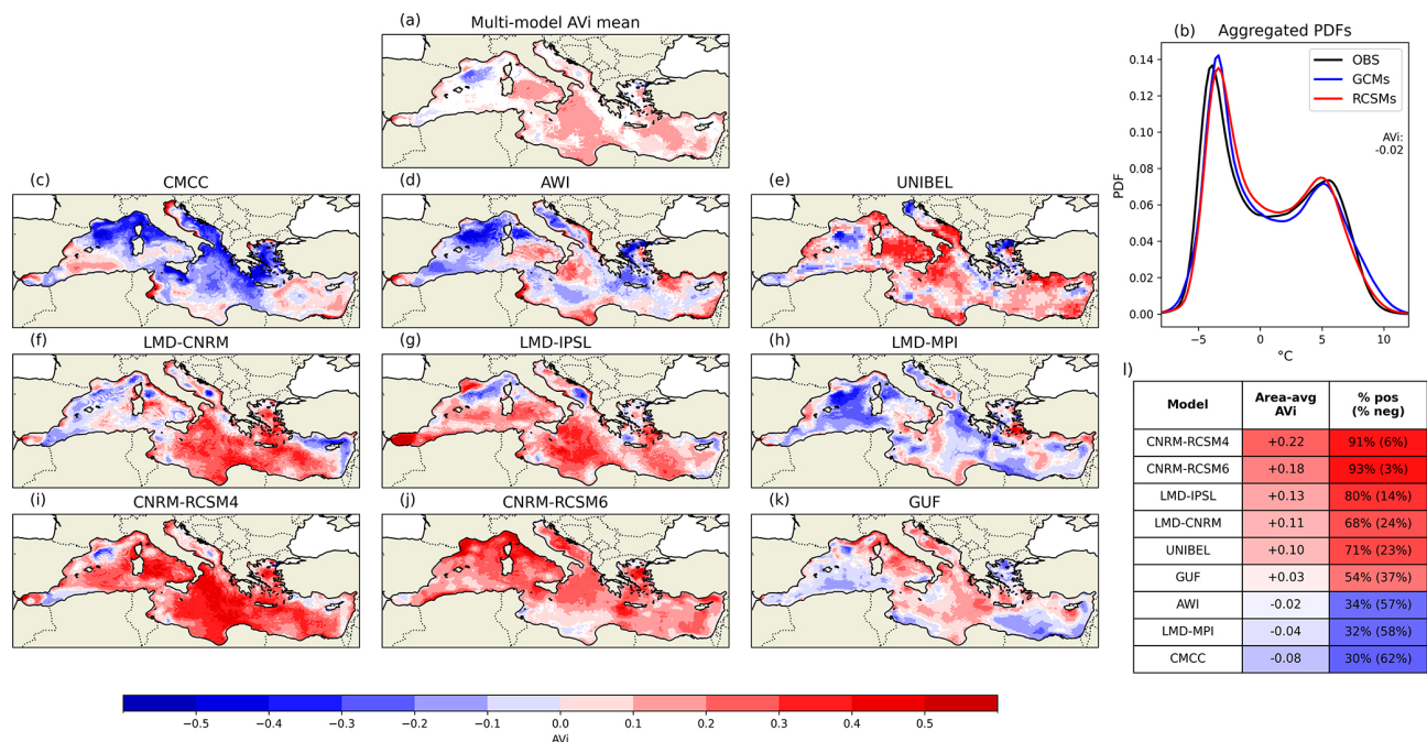
Figure 2. AVi for median-removed SST in 1982–2020. (a) Multi-model AVi mean; grid points where fewer than 6 out of 9 simulations agree in sign with the mean are masked. (b) Aggregated PDFs of median-removed SST at AVi-significant grid points across all GCMs, RCSMs and OBS, with the corresponding AVi value (see Sect. 2.2.2). Individual model AVi maps for (c) CMCC, (d) AWI, (e) UNIBEL, (f) LMD-CNRM, (g) LMD-IPSL, (h) LMD-MPI, (i) CNRM-RCSM4, (j) CNRM-RCSM6, and (k) GUF. Positive (negative) values indicate that the RCSM provides a more (less) accurate representation of the observed distribution relative to the parent GCM; non-significant grid points are shown in white. (l) Area-averaged AVi computed over the Mediterranean domain (non-significant grid points set to zero), with red (blue) indicating positive (negative) area-averaged AVi. The percentage of positive and negative AVi grid points in the domain is reported in red (blue) when the positive (negative) fraction dominates.
