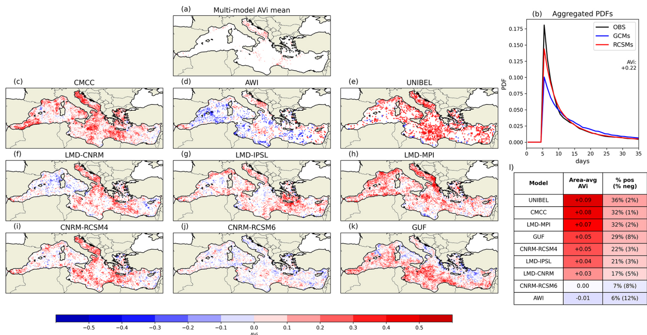
Figure 5. As in Fig. 2 but for MHW durations in 1982–2020. MHWs are calculated using a fixed baseline in 1982–2011 (see Sect. 2.2.2).
