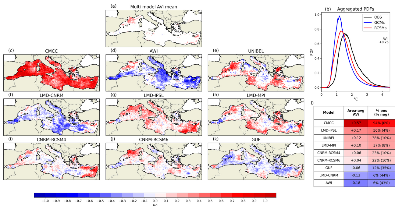
Figure 6. As in Fig. 2 but for MHW mean intensities in 1982–2020. MHWs are calculated using a fixed baseline in 1982–2011 (see Sect. 2.2.2).
