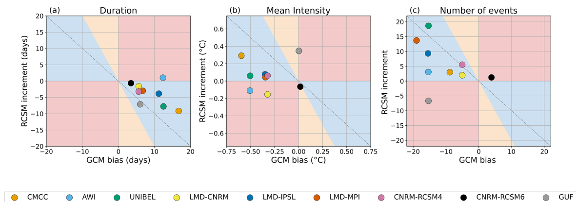
Figure 4. As in Fig. 1 for area-averaged MHW properties (1982–2020): (a) duration, (b) mean intensity, and (c) number of events. MHWs are calculated using a fixed baseline in 1982–2011 (see Sect. 2.2.2).
