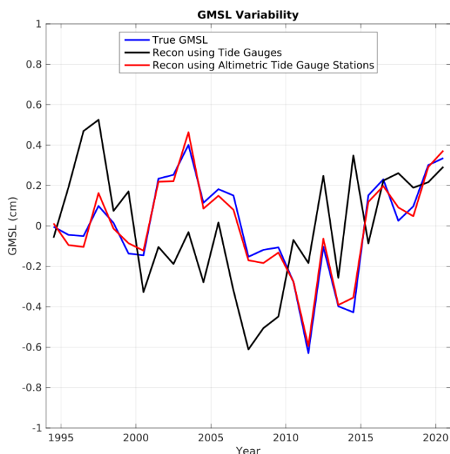
Figure 5. Comparison between the true GMSL and our GMSL reconstructions using tide gauge observations (black line) and virtual altimetric tide gauges (red line) for the period 1994 to 2020. The “true” GMSL derived from altimetry is shown as a blue line. All timeseries are detrended.
