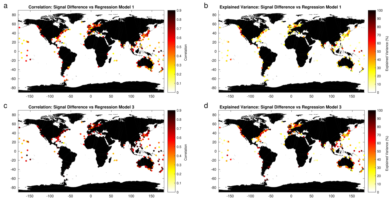
Figure 11. The correlations (a) between the Signal Differences and the regression Model 1, Eq. (3) and the corresponding explained variance (b). The correlations (c) between the Signal Differences and the regression Model 3, Eq. (5) and the corresponding explained variance (d).
