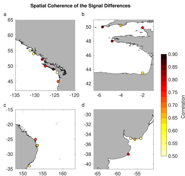
Figure 7. The spatial coherence of the Signal Differences in the west coast of North America (a); the Bay of Biscay (b); north-east Australia (c) and the Río de la Plata basin Argentina/Uruguay (d). The correlations are significant at the 95 % Confidence Interval (CI).
