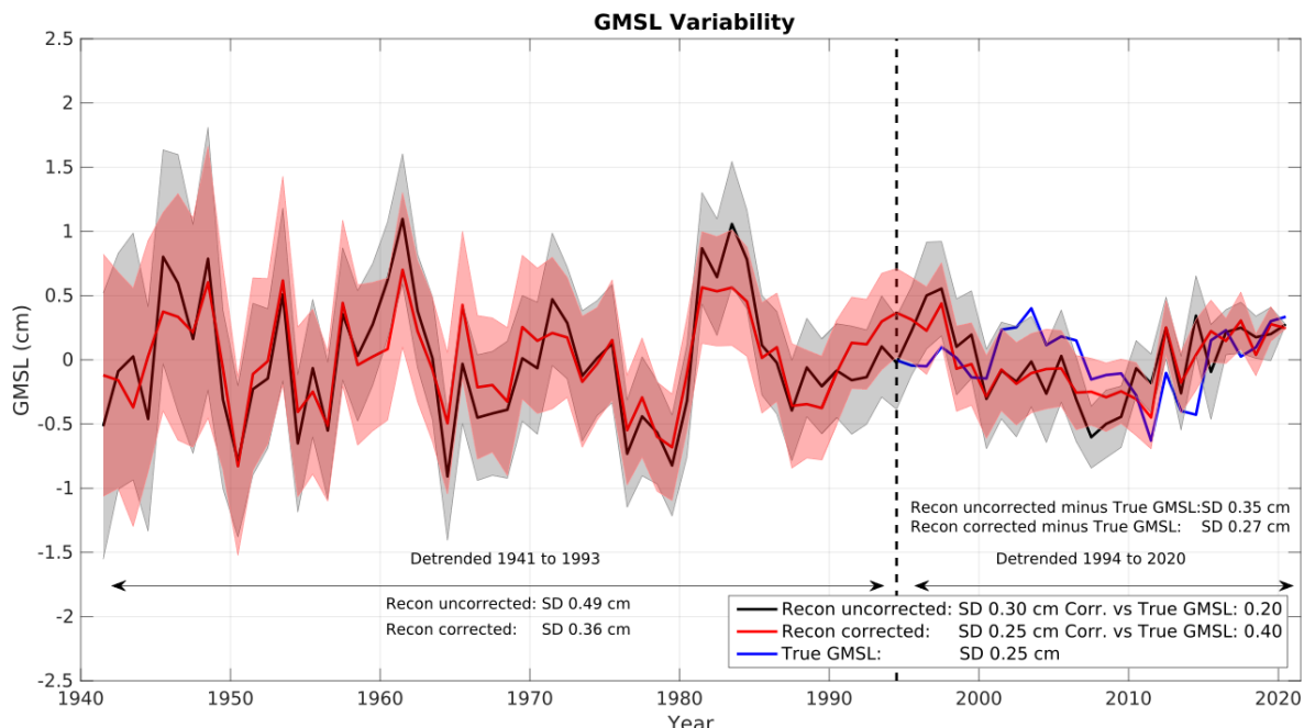
Figure 13. The variability of the GMSL that has been detrended for two time periods 1941 to 1993 and 1994 to 2020 showing the uncorrected EOF reconstruction (black line) derived from Eq. (2) and the corrected EOF reconstruction (red line). The 1-sigma uncertainty intervals shaded grey (uncorrected) and light red (corrected) reflect the sensitivity of the reconstruction to the number of tide gauges as evaluated standard deviation (SD) using a bootstrap method. The detrended “true” GMSL derived from altimetry is shown as a blue line (1994 to 2020).
