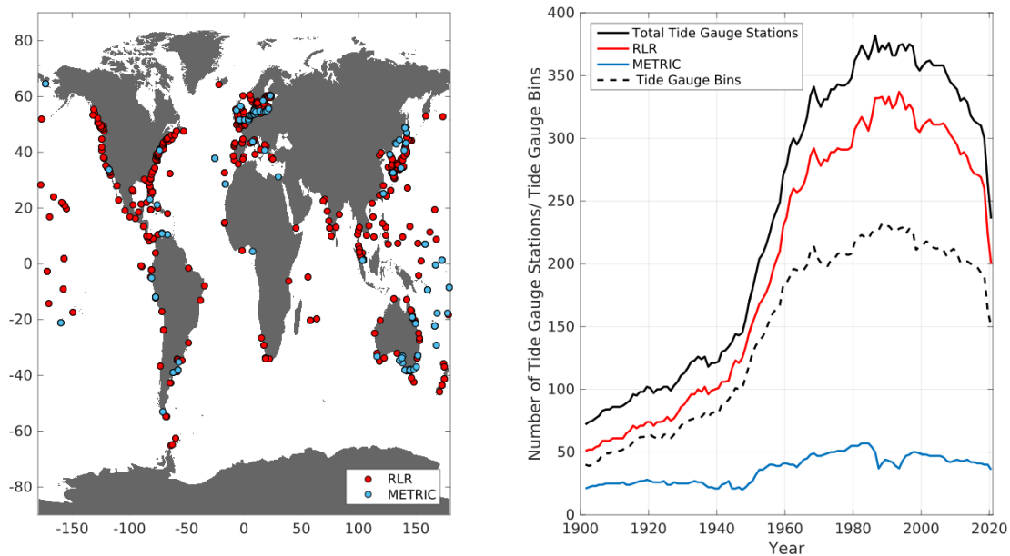
Figure 2. The spatial and temporal distribution of the number of tide gauges used in this study (1901–2020). The dashed black line represents the temporal distribution of the tide gauge bins containing composite tide gauge observations for the EOF GMSL reconstruction.
