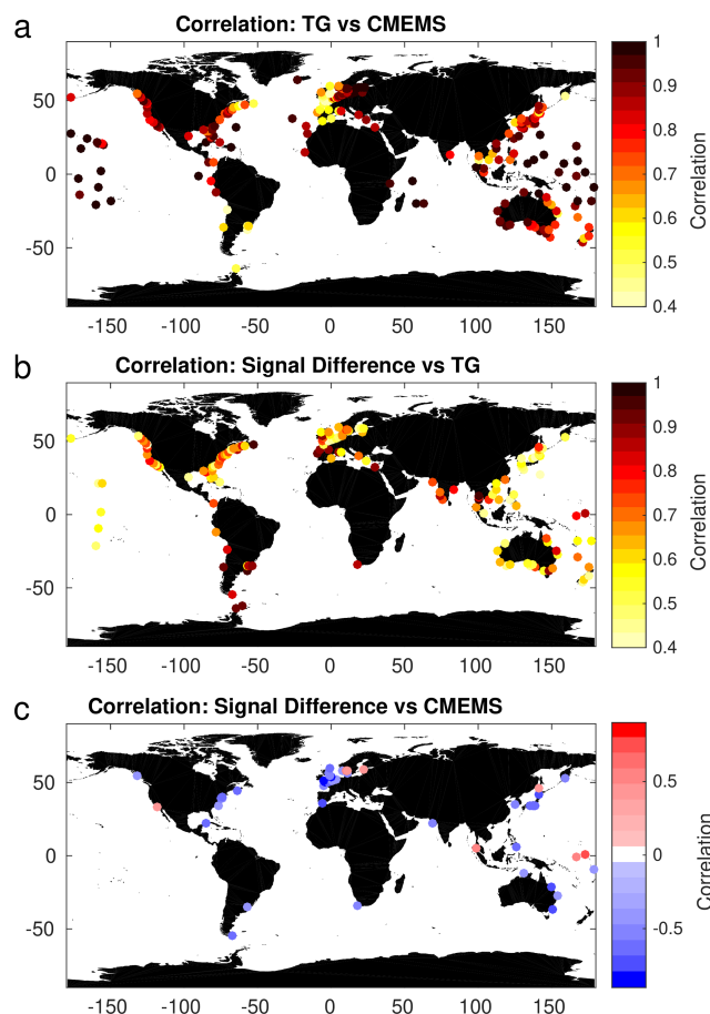
Figure 8. Correlations between tide gauge and CMEMS altimetry (a); between the Signal Differences and tide gauges (b); and between Signal Differences and CMEMS altimetry (c). Only correlations that are statistically significant at the 95 % CI are shown.
