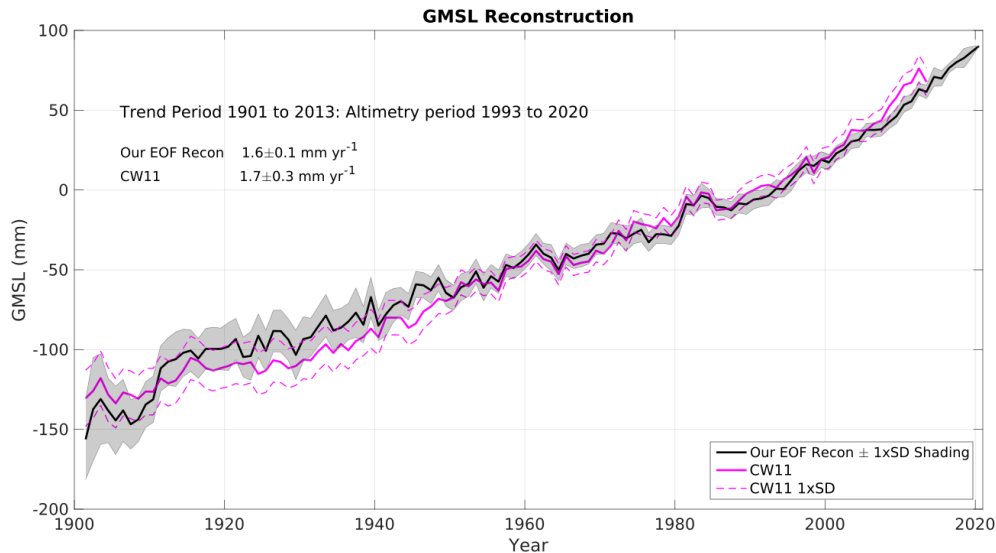
Figure 4. Comparison of our EOF reconstruction (black) derived from Eq. (2) with that of CW11 (magenta). The shaded area (grey) represent the 1-sigma uncertainty interval, which reflects the sensitivity of the reconstruction to the number of tide gauge bins as evaluated Standard deviation (SD) using a bootstrap method.
