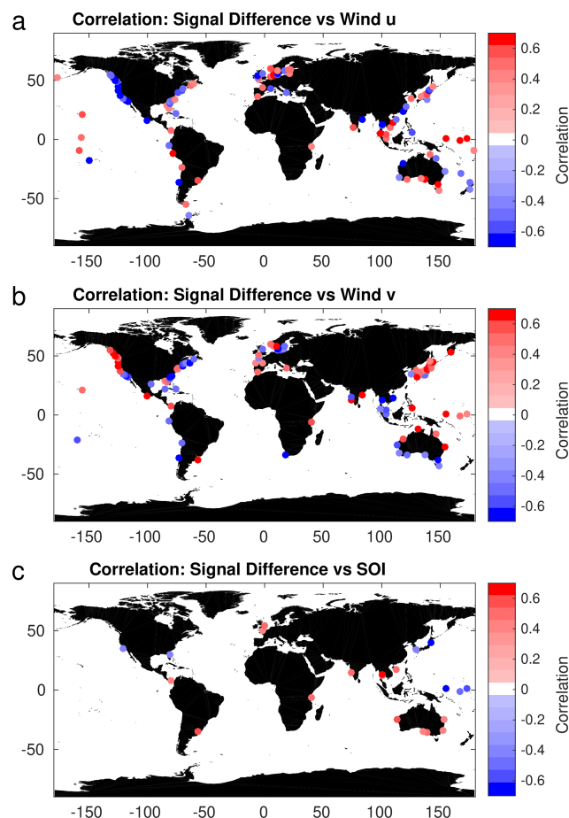
Figure 9. Correlations between the Signal Differences and wind u parameter (a); between the Signal Differences and wind v (b); and between the Signal Differences and the Southern Oscillation Index (SOI) (c). Only correlations that are statistically significant at the 95 % CI are shown.
