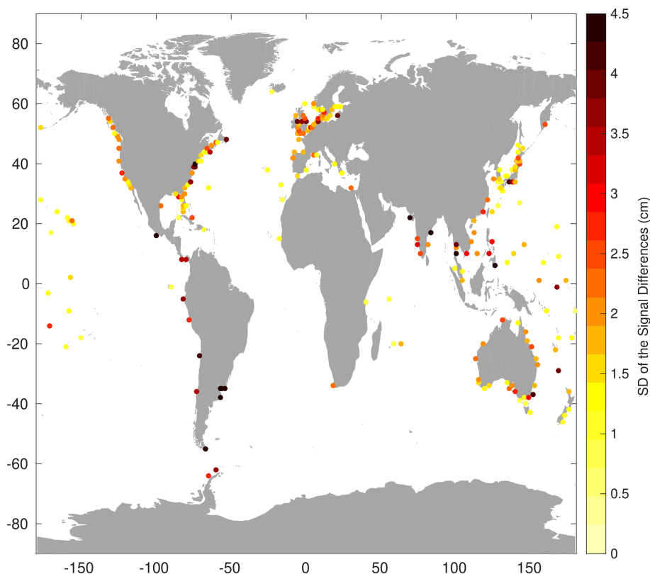
Figure 6. The Standard Deviation (SD) of the Signal Differences.
