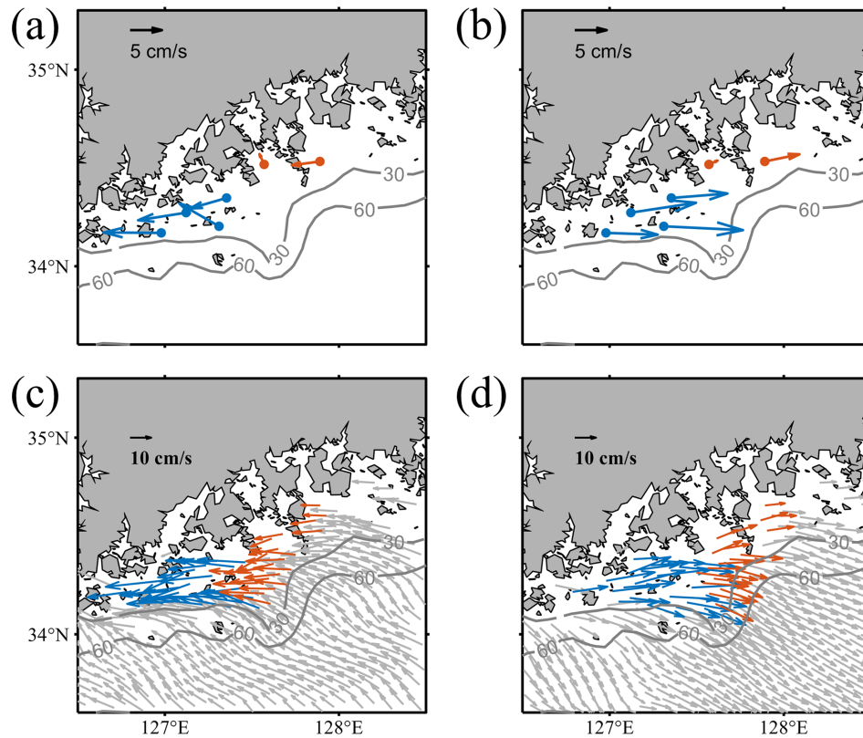
Figure 5. Composite means of (top) observed surface currents and (bottom) simulated surface currents from the realistic model during (left) westward and (right) eastward winds exceeding 5 \text{ m s}^{-1} from 1 July to 18 September.
