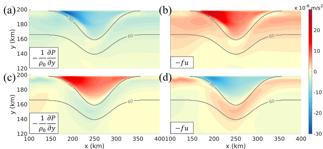
Figure 7. Cross-shore depth-averaged momentum balances calculated from the idealized model results during (top) westward winds on day 18 and (bottom) eastward winds on day 22. Gray contours represent the bottom topography, with depths indicated in meters.
