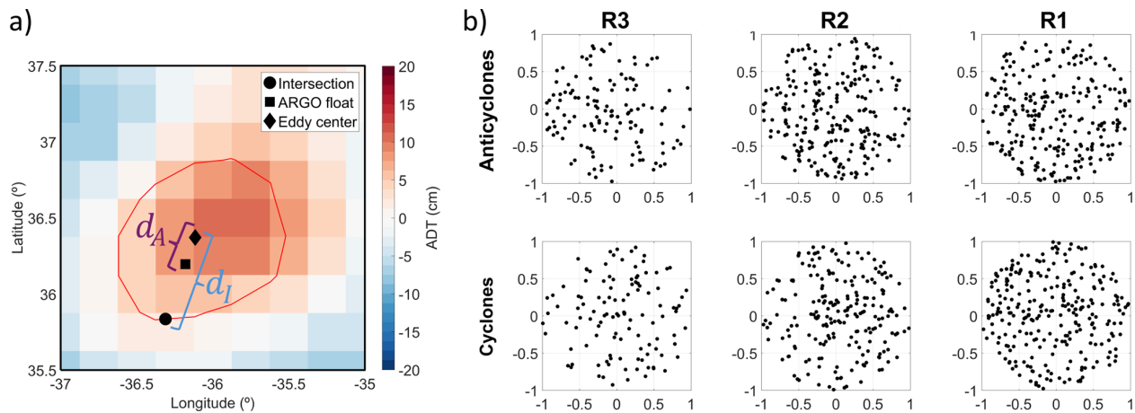
Figure 2. (a) Illustration of an anticyclone’s characteristics: ADT (colours), eddy centre (black diamond), and the eddy speed contour (red line). The float’s position (black square) and the intersection of a line (in the direction of the float azimuth) with the eddy speed contour (black circle) are also shown. The distances d_A and d_I were used to normalise the distance of every float to the eddy centre. (b) Normalised distance of the Argo profiles to the eddy centre for all points used to construct the eddy composite for the three AzCCo regions and both sign structures.
