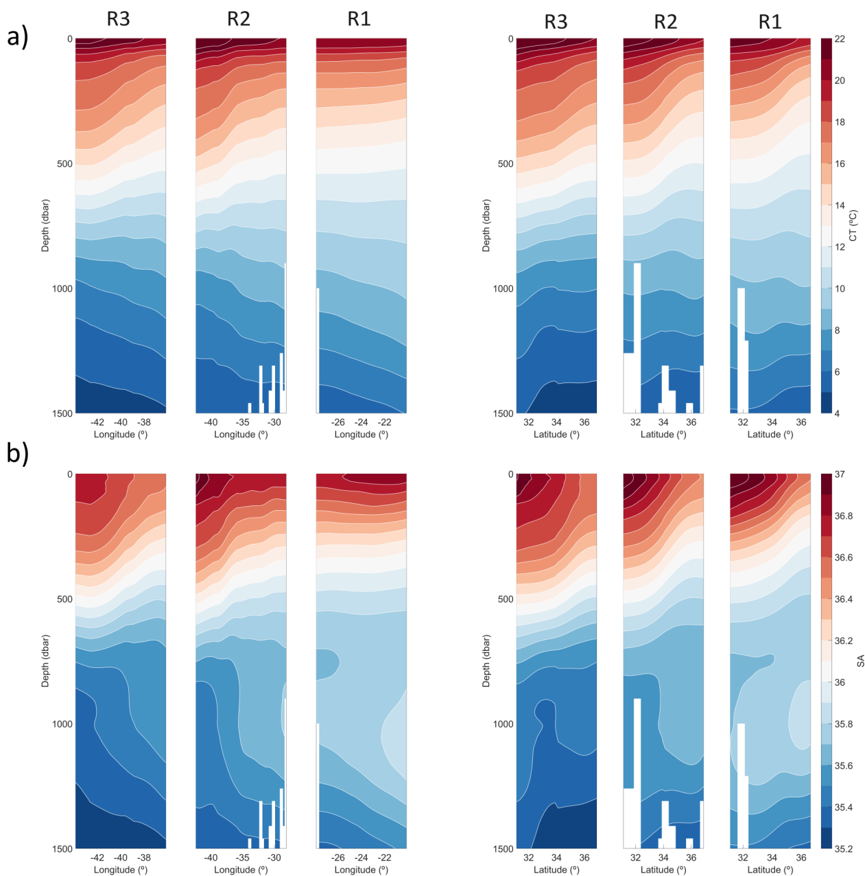
Figure 6. Mean WOA2018 climatology inside the three regions associated with the AzCCo for (a) CT and (b) SA. On the left are represented the meridional means and, on the right, the zonal. White represents the topography of the region associated with the SWSM chain and the shallower part of MAR.
