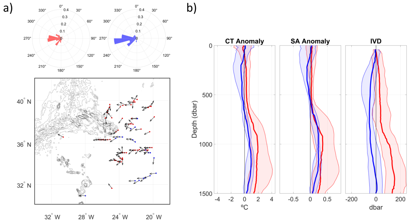
Figure 10. (a) Map of the general trajectories of the sampled meddies (anticyclones red and cyclones blue) for a period of 10 d. The polar graph represents the relative frequency in each class of the individual trajectory's azimuth, binned in 15° classes. (b) Median vertical structure of the meddies' profiles for both sign structures (anticyclone red and cyclone blue) for the CT and SA anomalies and the vertical displacement, IVD.
