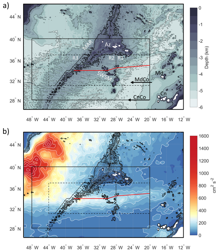
Figure 1. (a) Bathymetric map. MAR – Mid-Atlantic Ridge; SWSM – Seawate Seamount Chain; MdCo – Madeira Corridor; CnCo – Canary Corridor; Md – Madeira Island; Cn – Canary Island; Az – Azores Islands. Bathymetric contours are drawn every 500 m from the surface down to 6 km depth. The thick black contour represents the 2500 m bathymetry, and the thin black ones the 4000 and 5000 m bathymetry. (b) Spatial distribution of mean EKE ( \text{cm}^2 \text{s}^{-2} ) for the period 2005–2017. Contours are highlighted in white every 50 up to 400 \text{cm}^2 \text{s}^{-2} , and then every 200 \text{cm}^2 \text{s}^{-2} thereafter. Bathymetric contours are drawn every 500 m from the surface down to 2500 m depth. The thick black contour represents the 2500 m bathymetric contour. In both panels, the black box indicates the study area, and the three dashed boxes represent the regions directly associated with the Azores Current Corridor: the eastern region (R1), the central region (R2), and the western region (R3). The red line represents the mean axis location of the AzC, following Silva-Fernandes and Peliz (2020). Land is shown in white.
